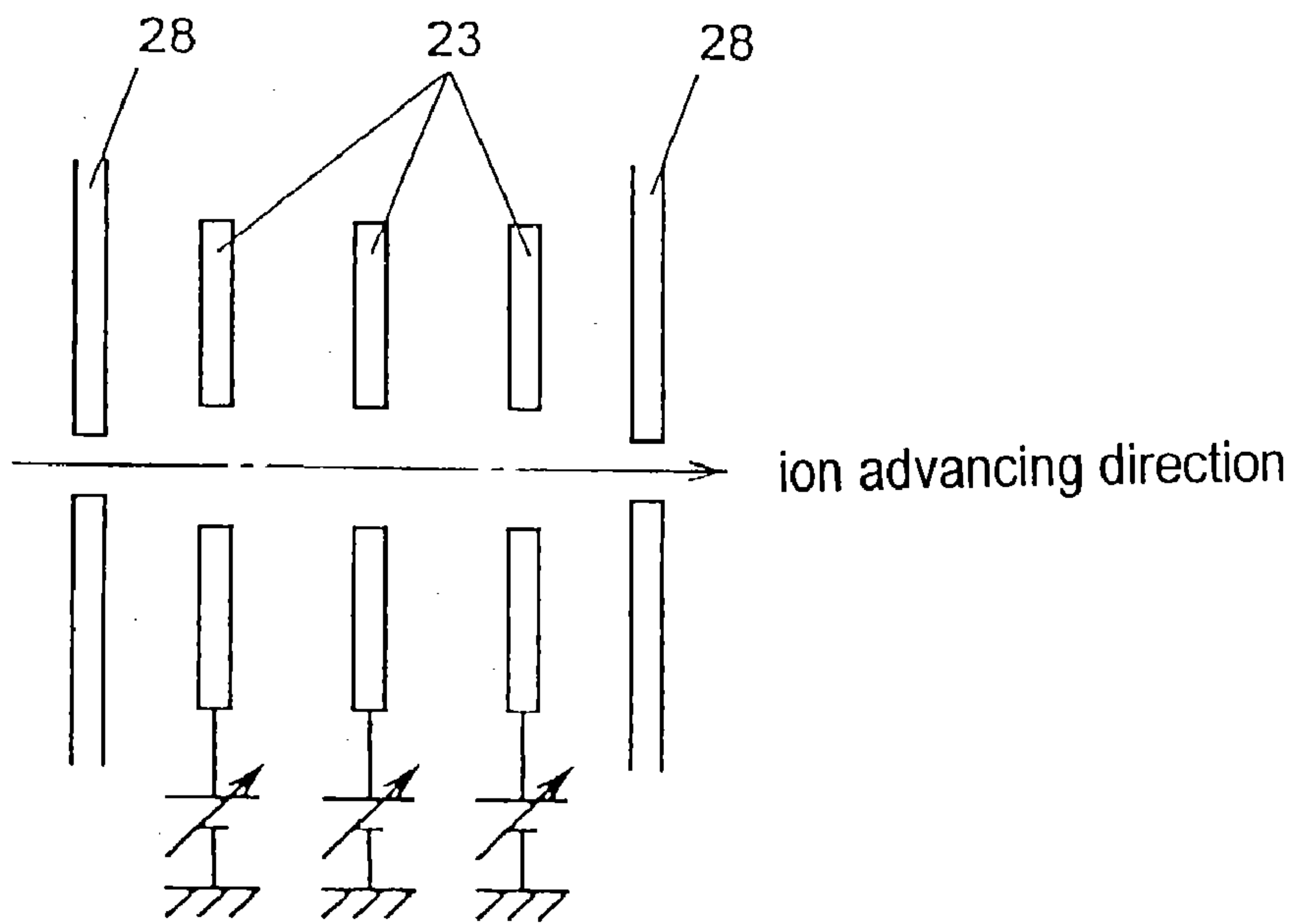
Fig. 2 Prior Art
