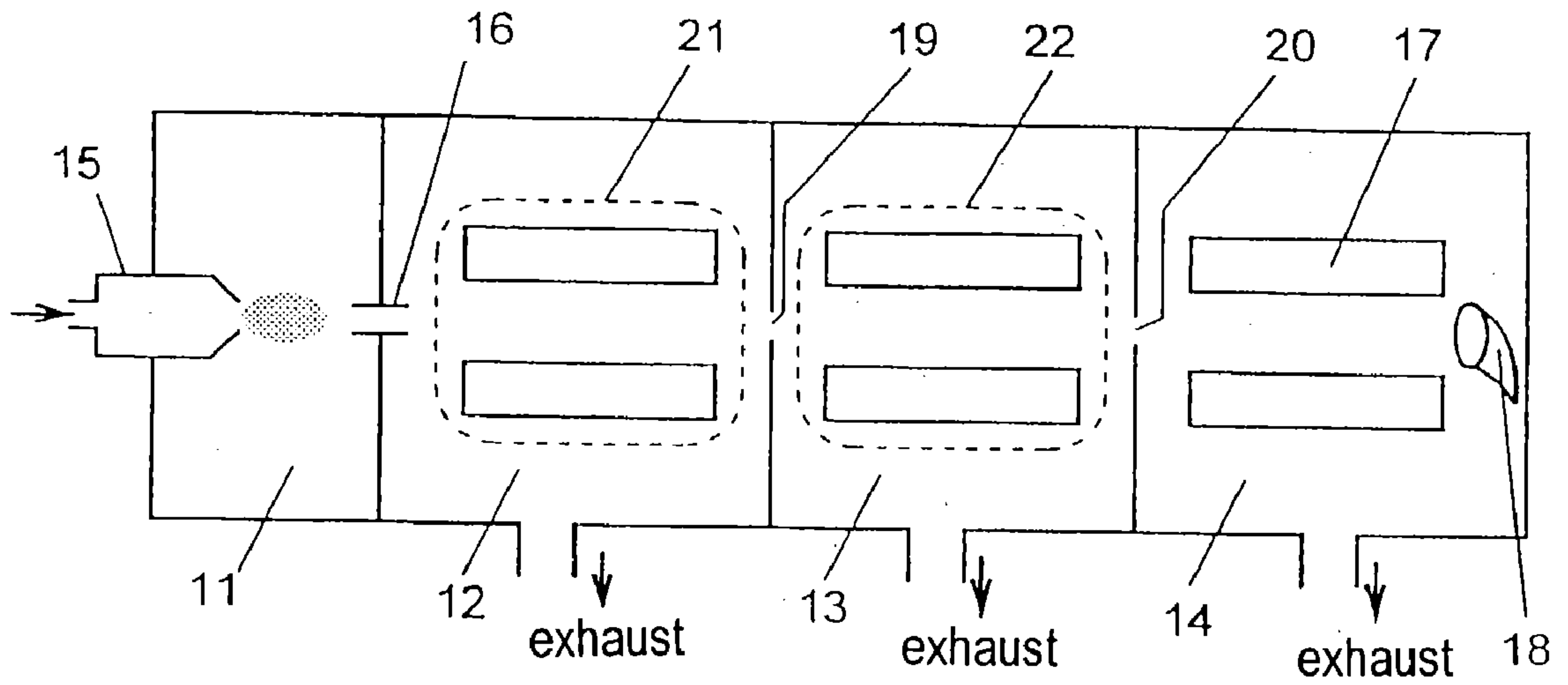
Fig. 2 Prior Art
