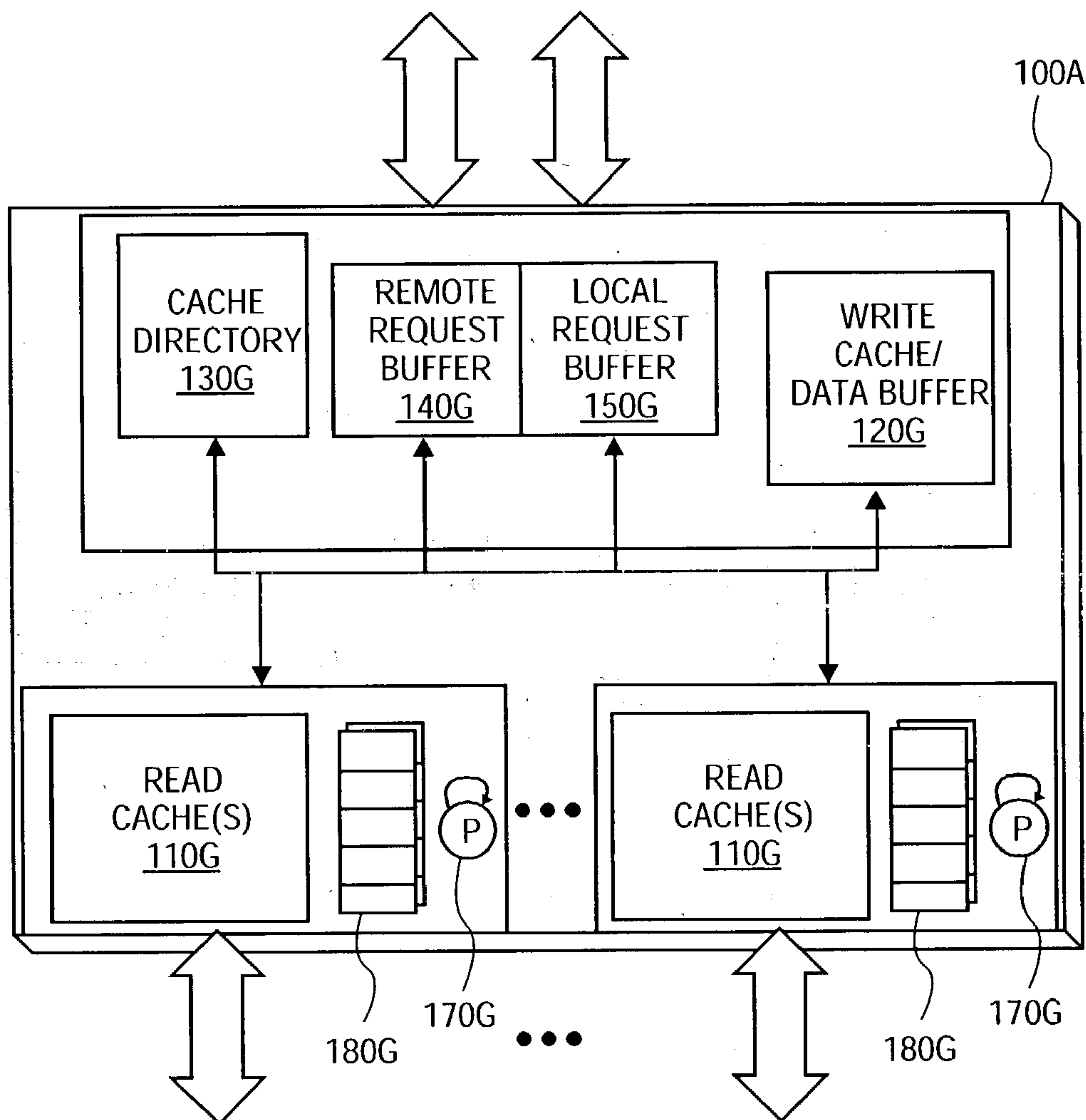
I/O HUB MICROARCHITECTURE
