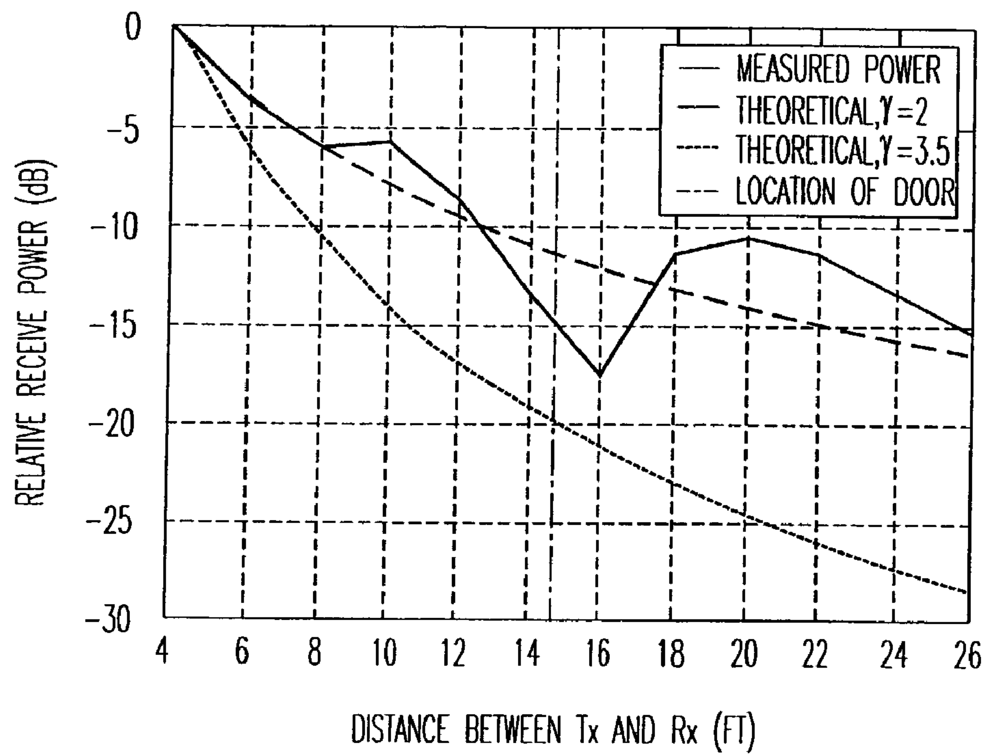
RECEIVE SIGNAL POWER AS A FUNCTION OF DISTANCE BETWEEN TRANSMITTER AND RECEIVER
