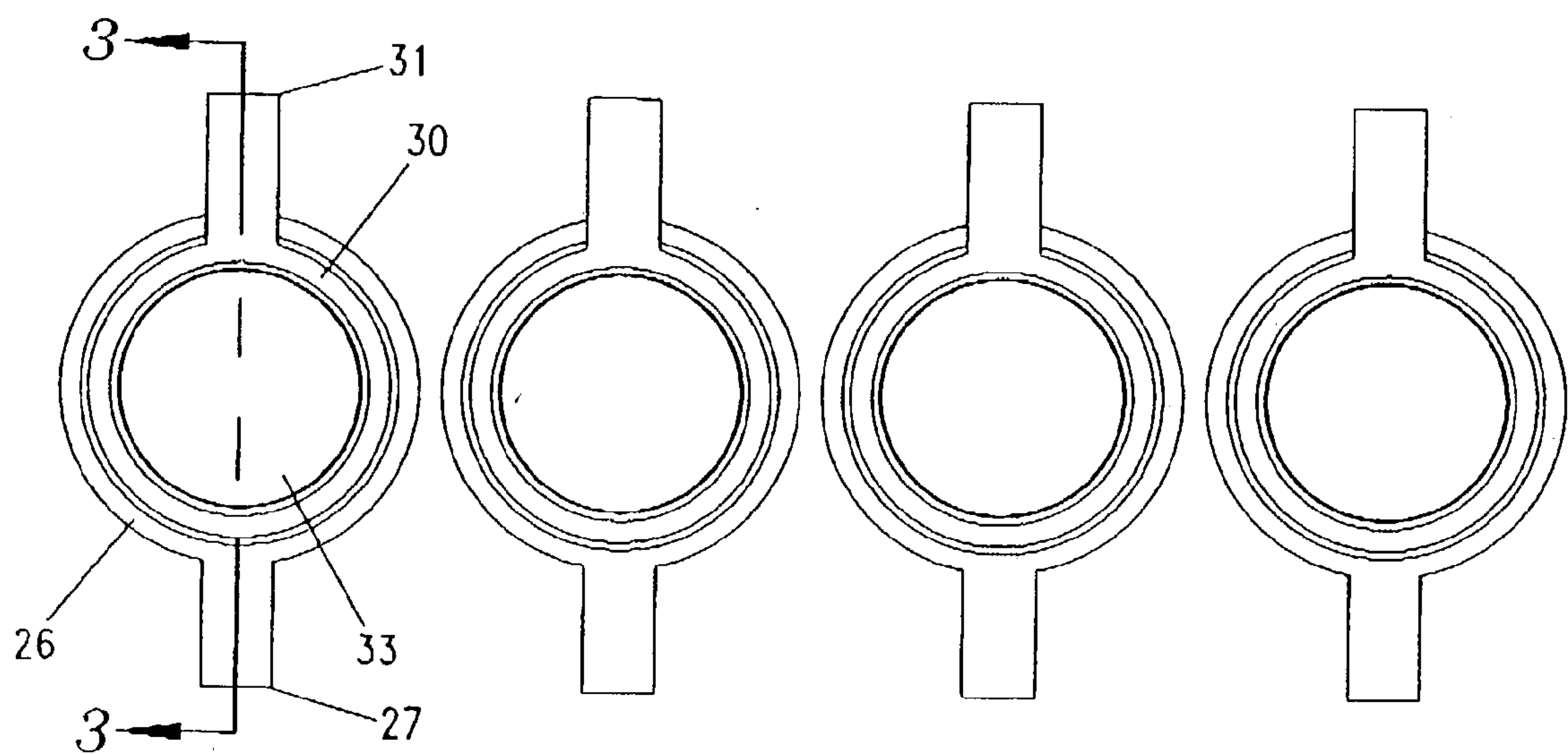
FIG. 4 (Prior Art)
