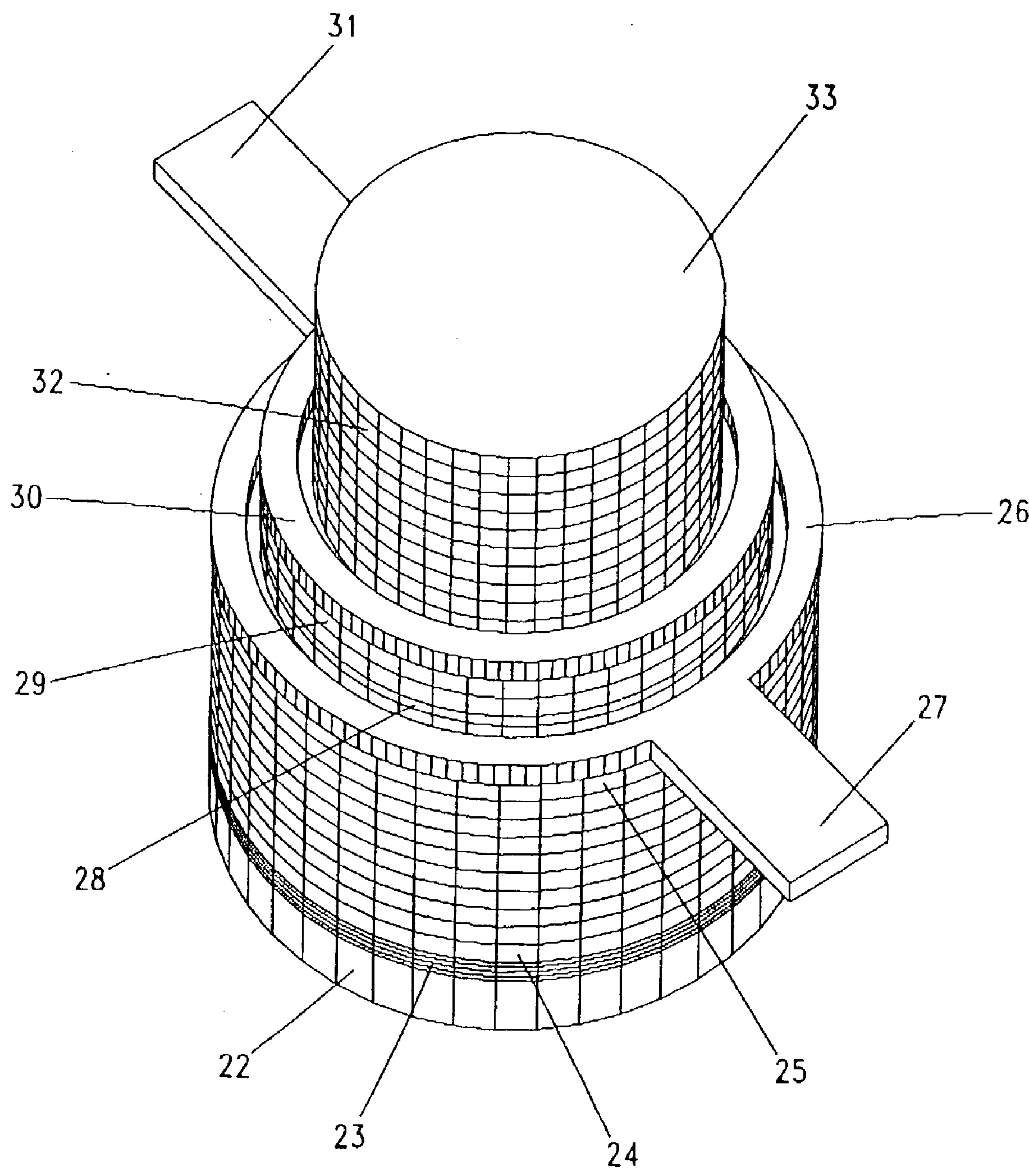
FIG. 1 (Prior Art)
