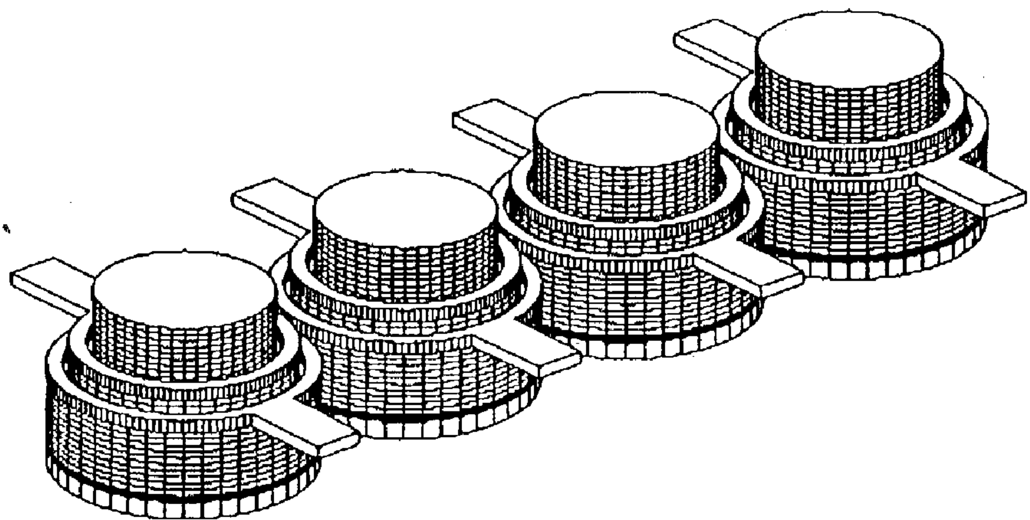
FIG. 5 (Prior Art)
