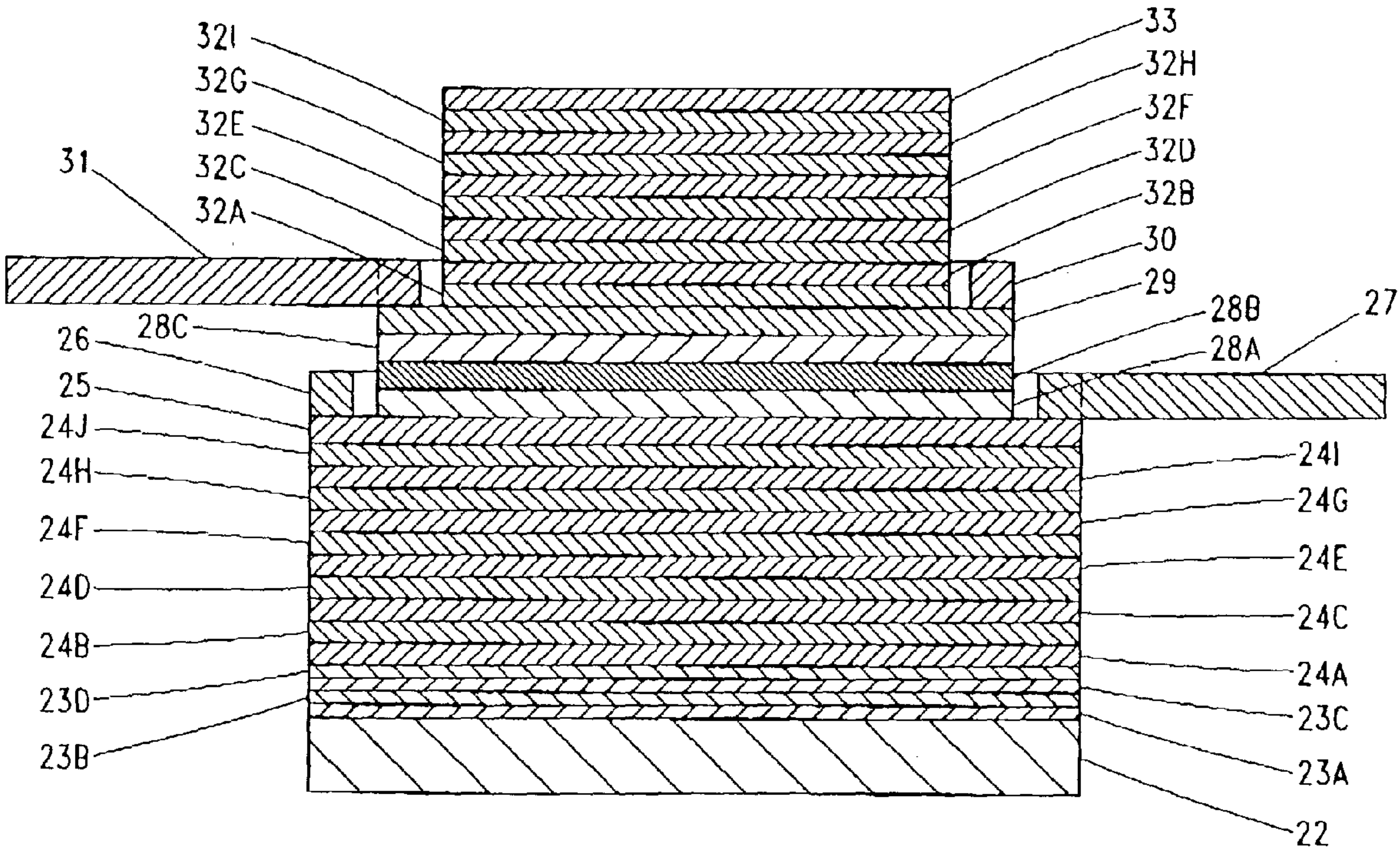
FIG.3 (Prior Art)
