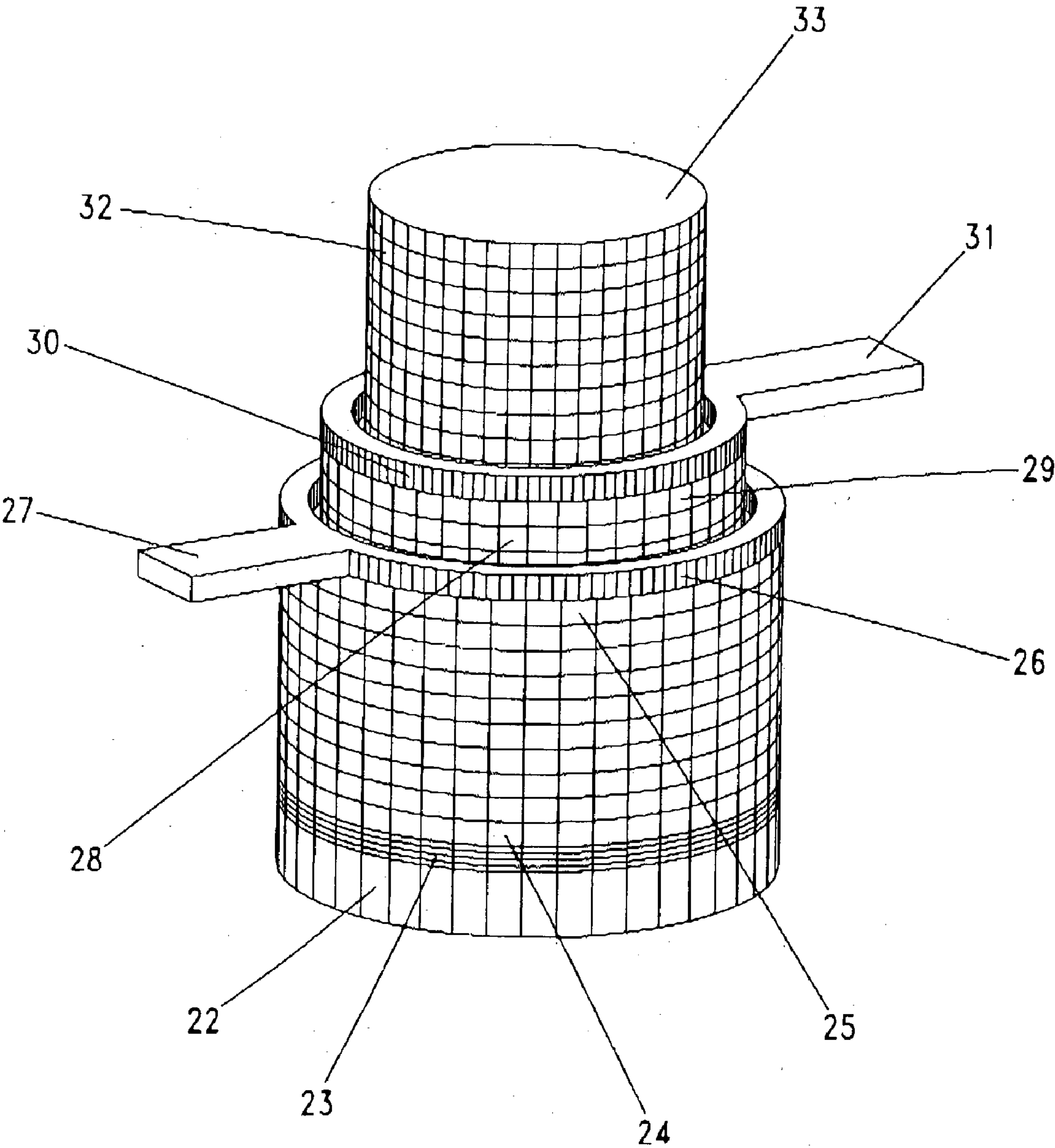
FIG. 2 (Prior Art)
