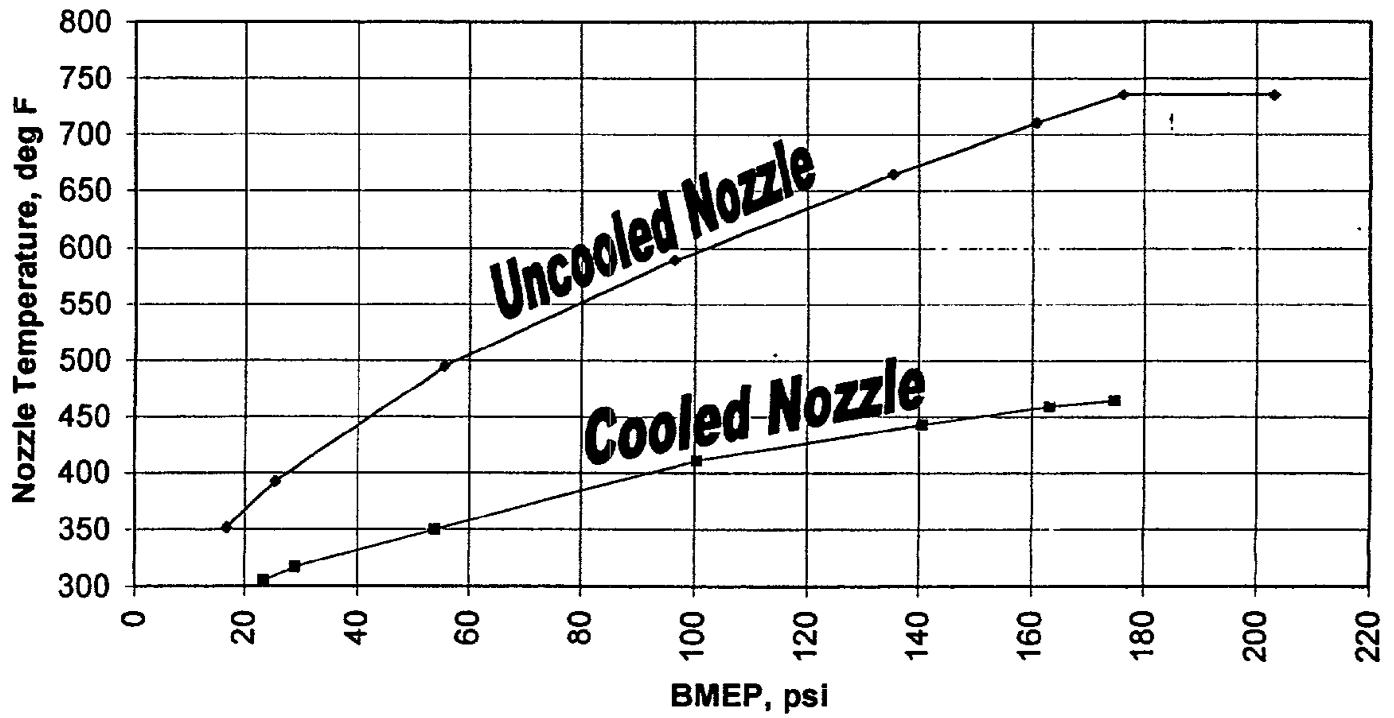
Injector Nozzle Temperature 2000 RPM
