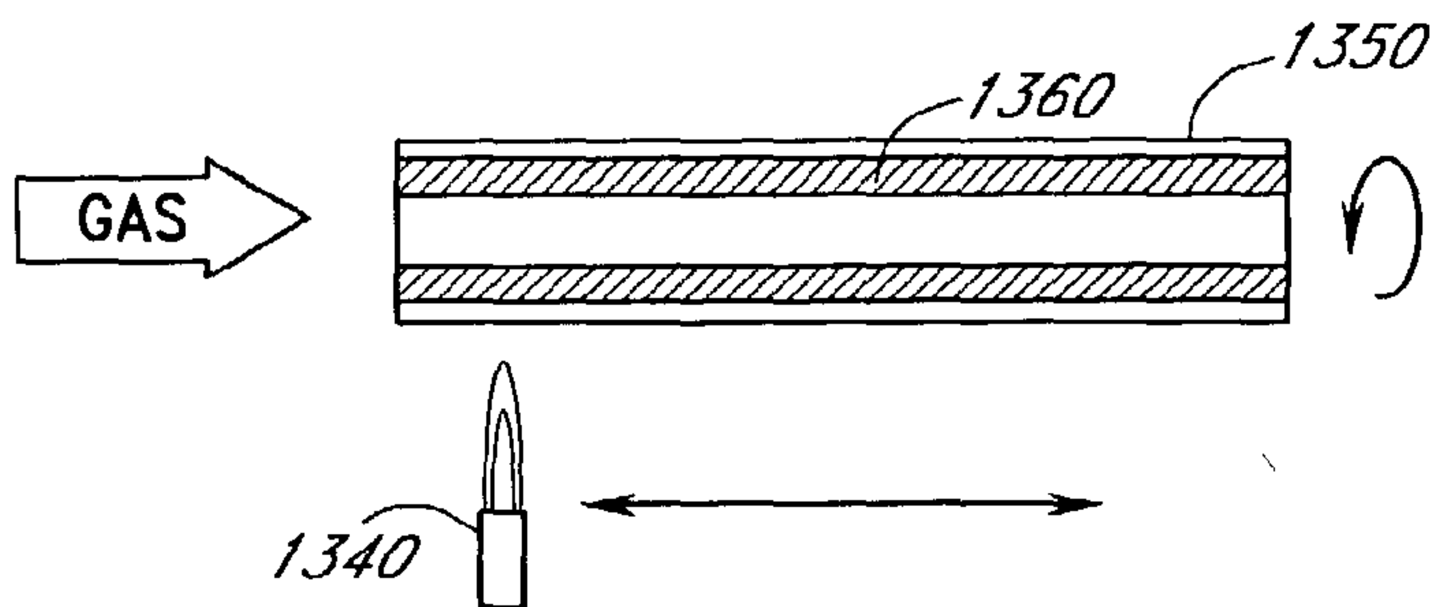
FIG. 28C (PRIOR ART)
