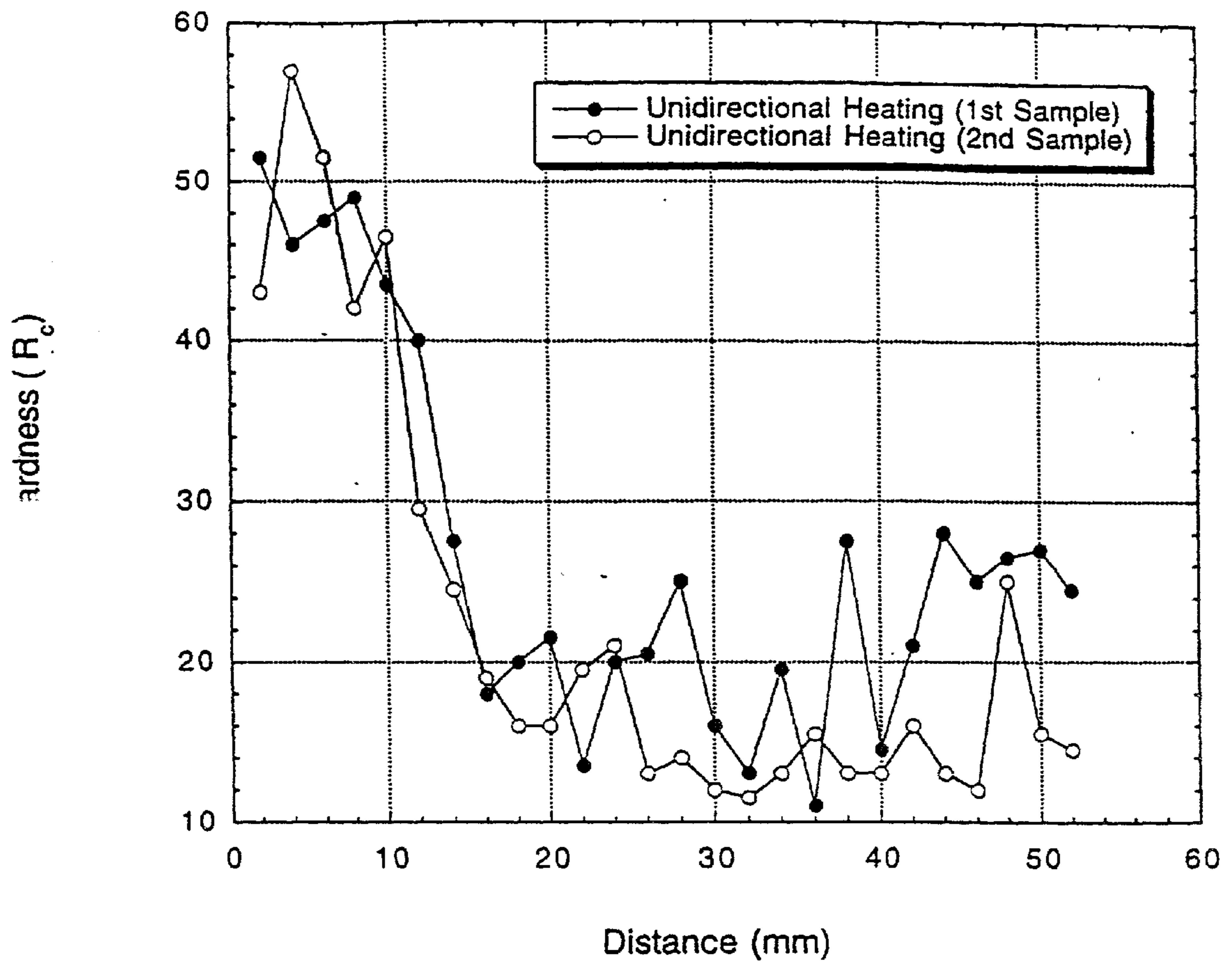
Hardness versus distance plot for Extendo-Die™ block after gradient heating by infrared source and water quenching.
