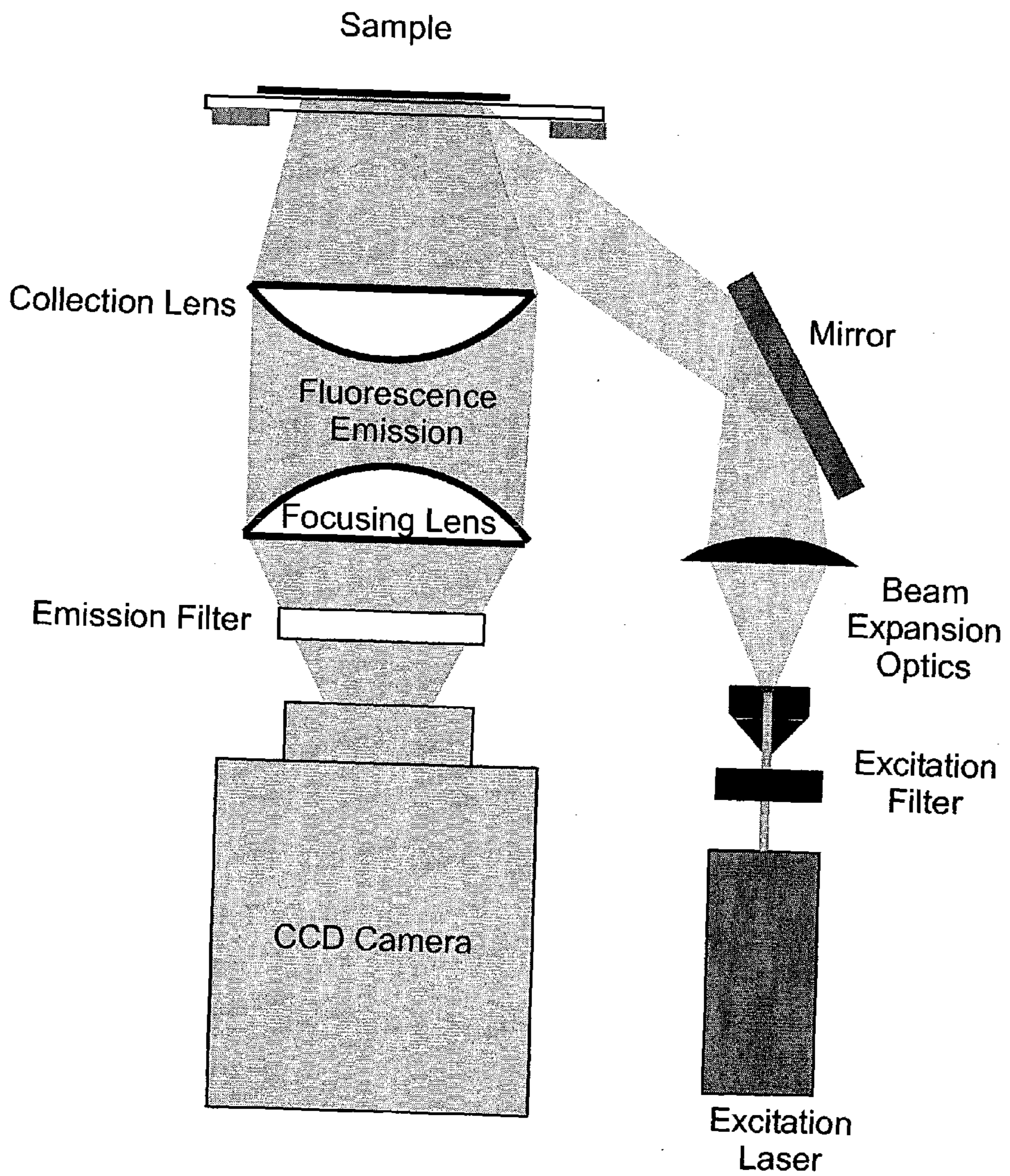
FIG. 4. A CCD imaging system for non-magnified large area imaging.
