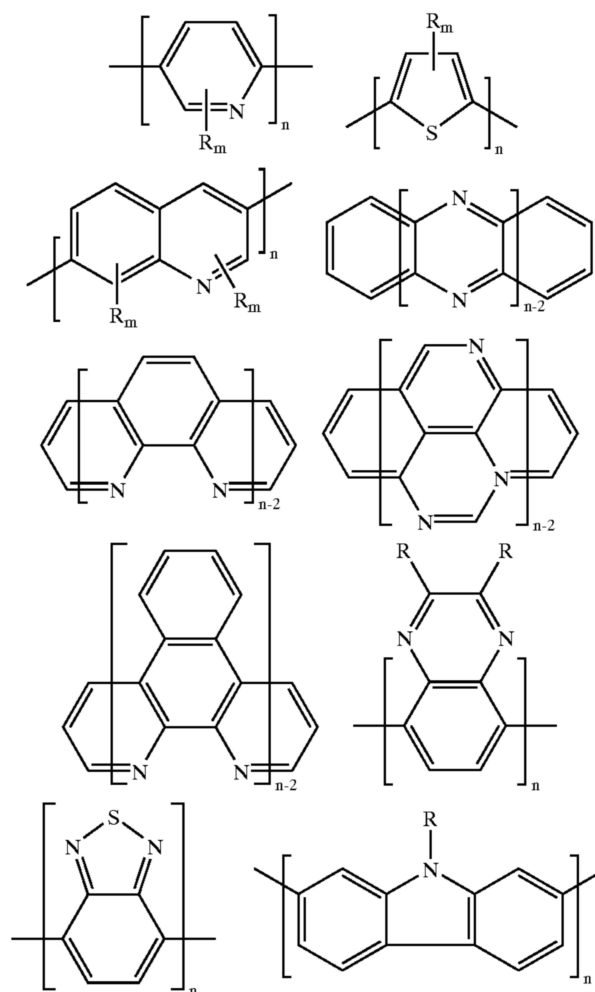
Scheme 3. Heterocyclic/fused ring heterocyclic combination.
