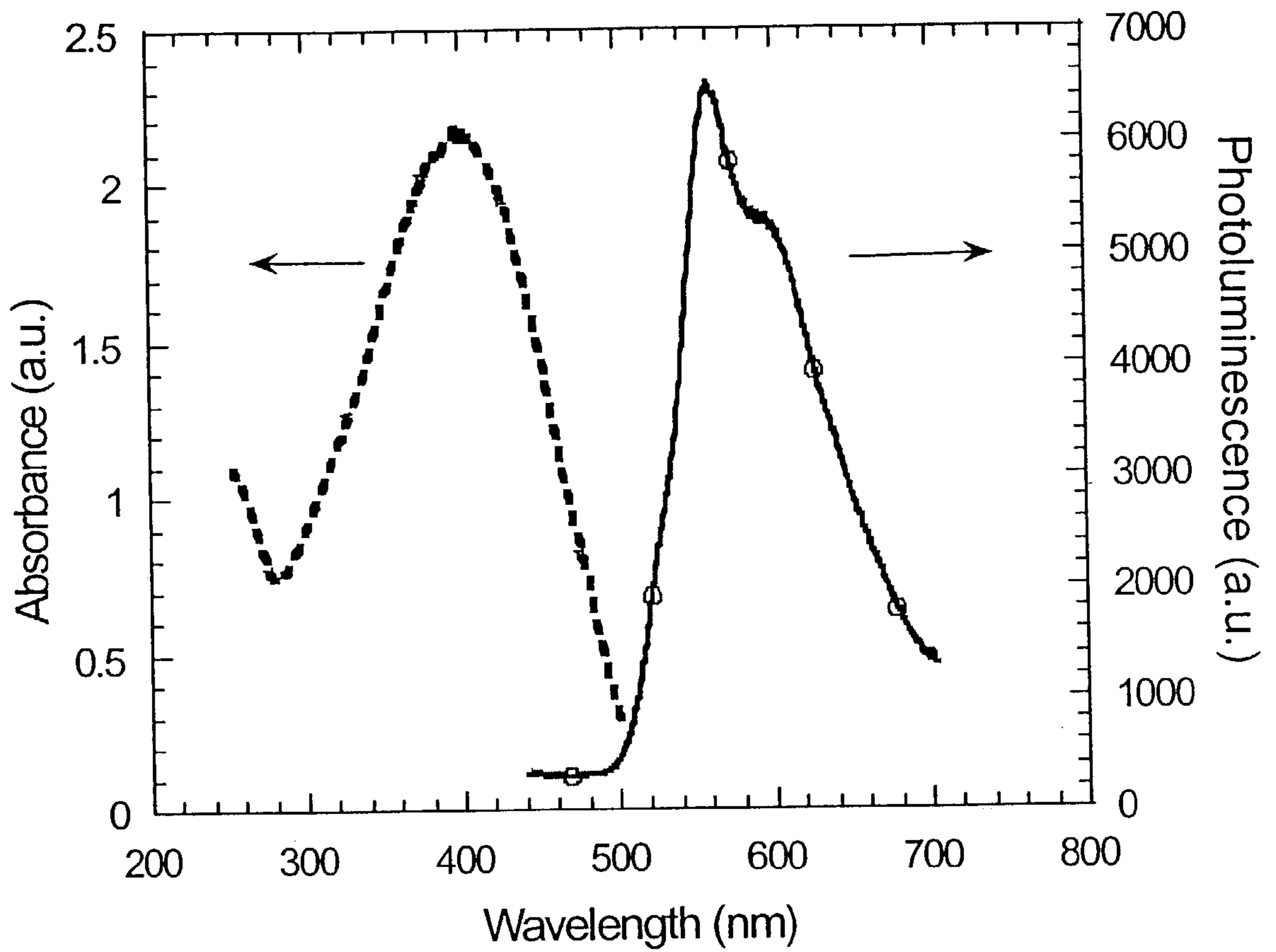
UV-Visible and Photoluminescent Spectra of D-PPV
