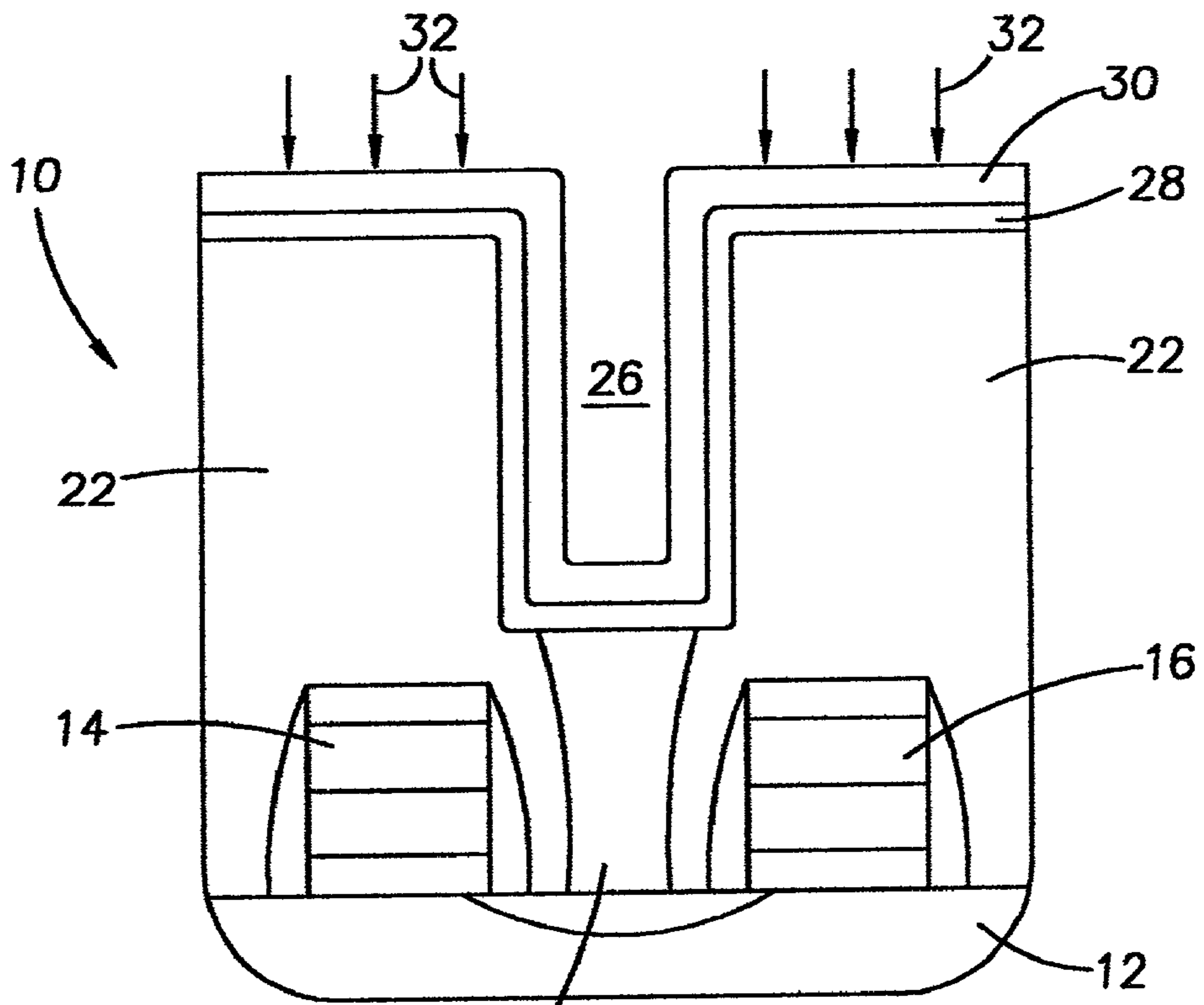
FIG. 1C PRIOR ART
