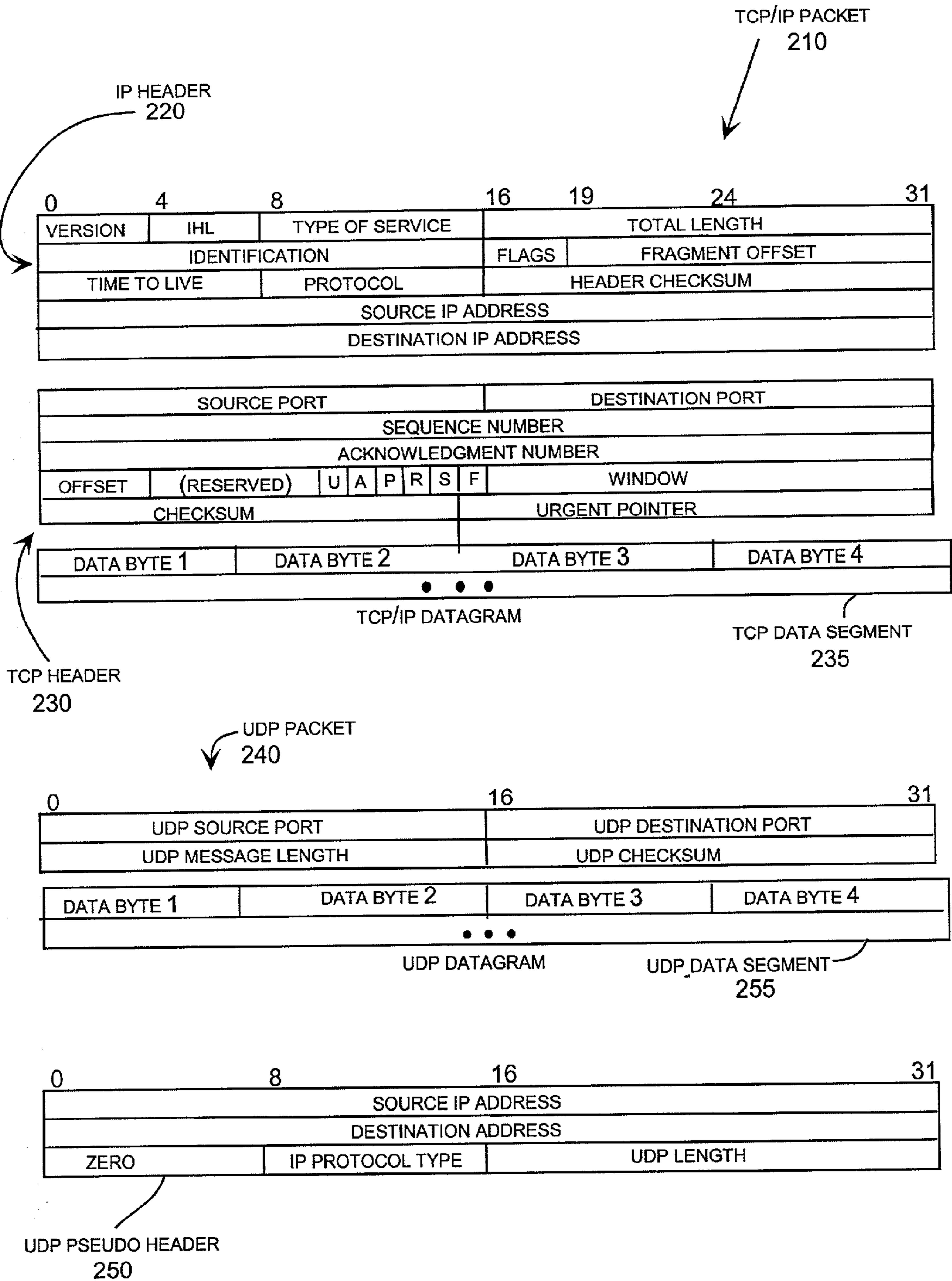
PACKET HEADERS FIG. 2
