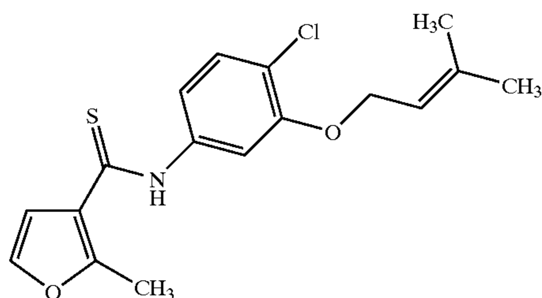
Structure of UC781™
