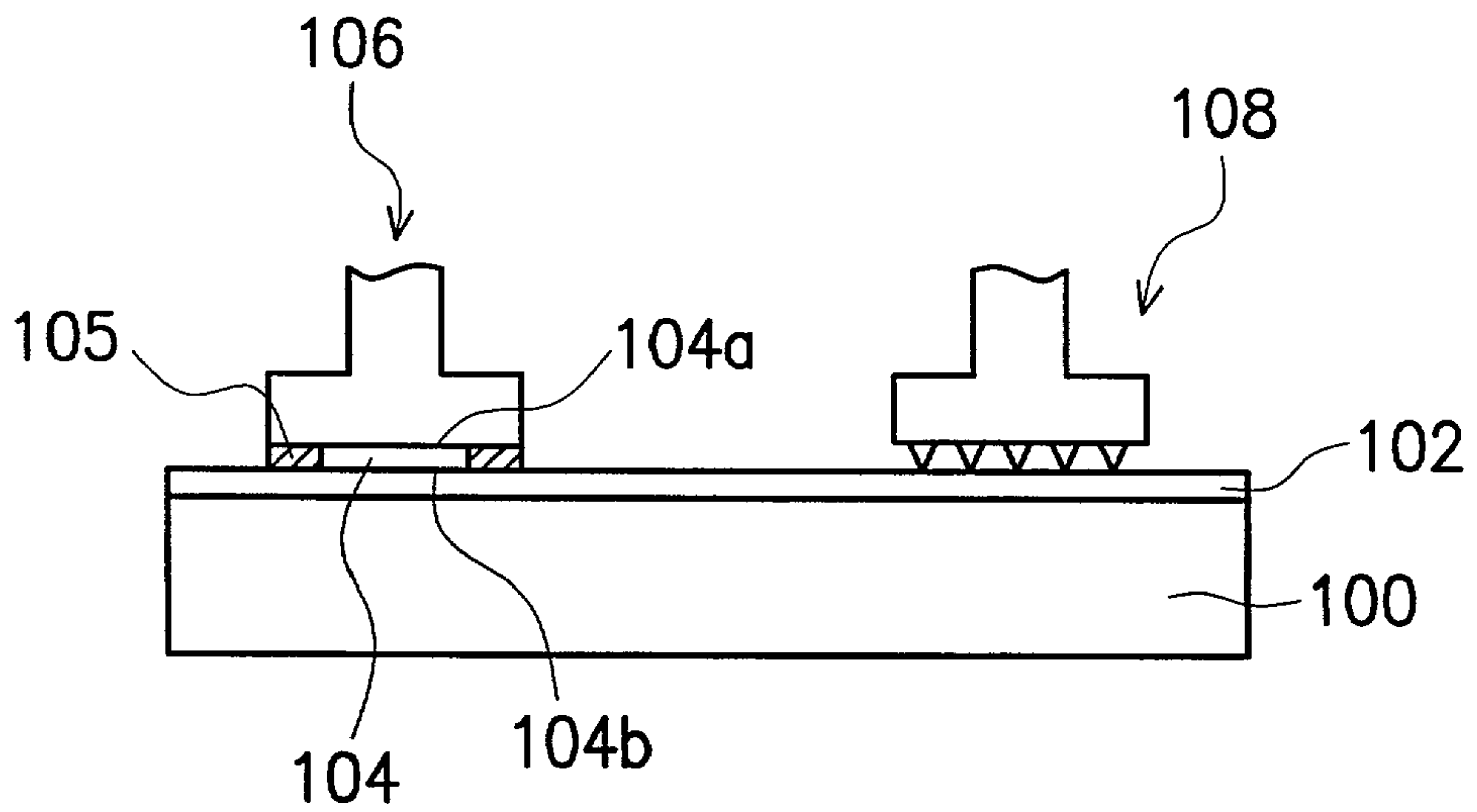
FIG. 1 (PRIOR ART)
