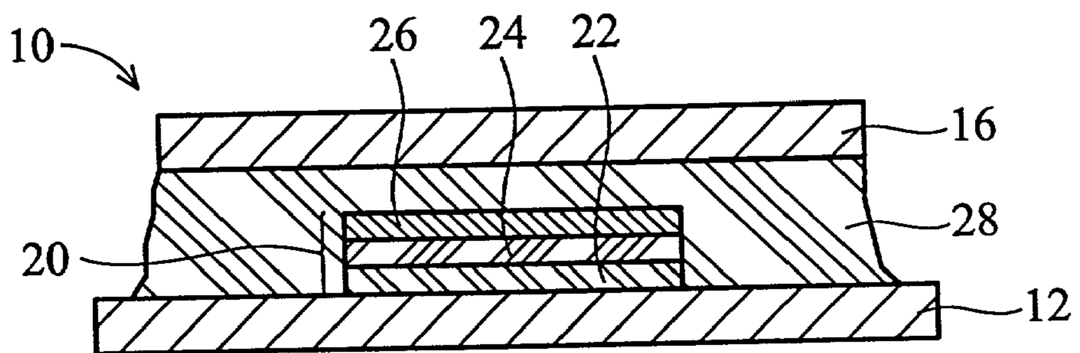
FIG. 1C ( PRIOR ART )
