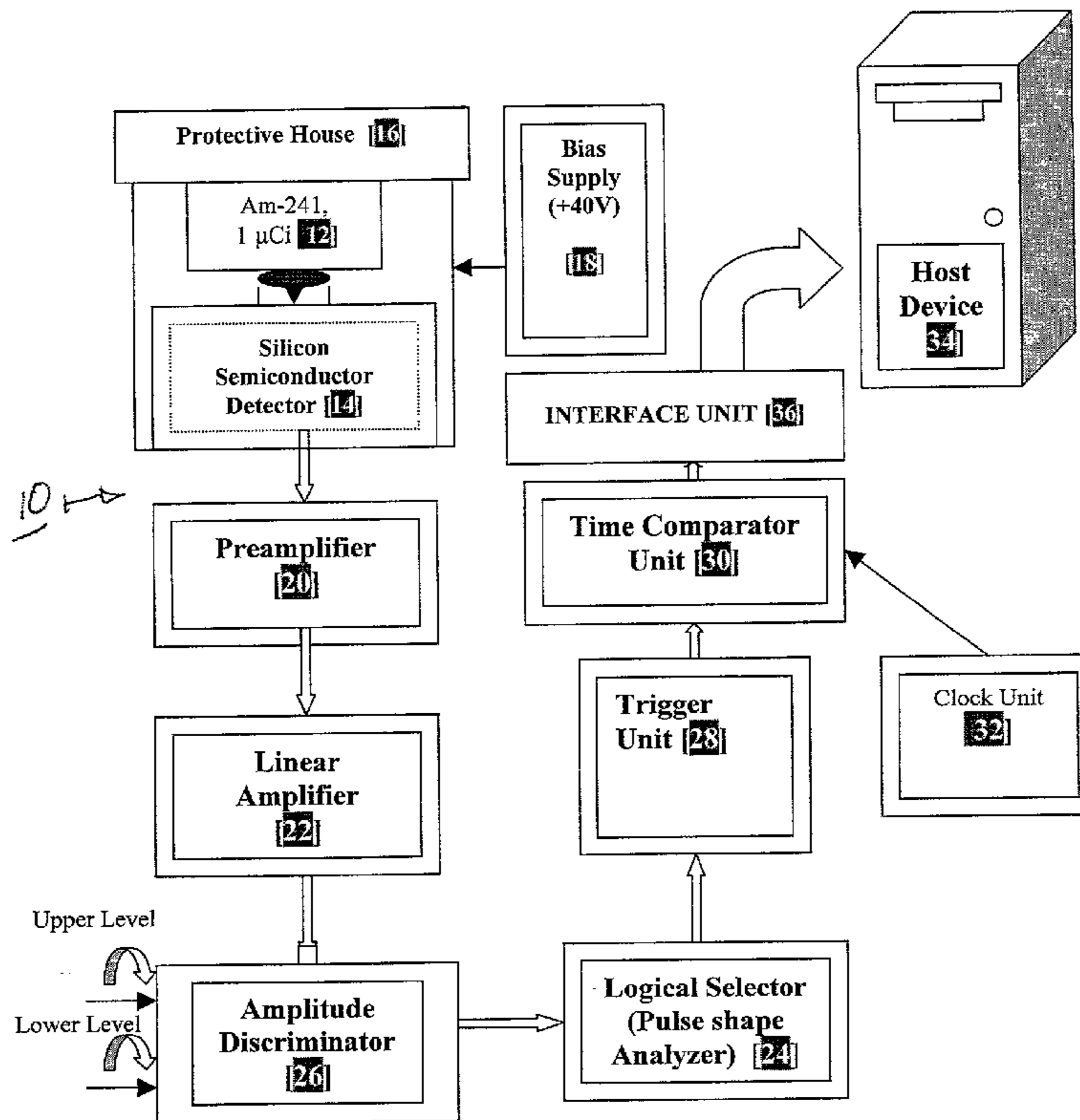
Block Diagram of an alpha-based RNG
