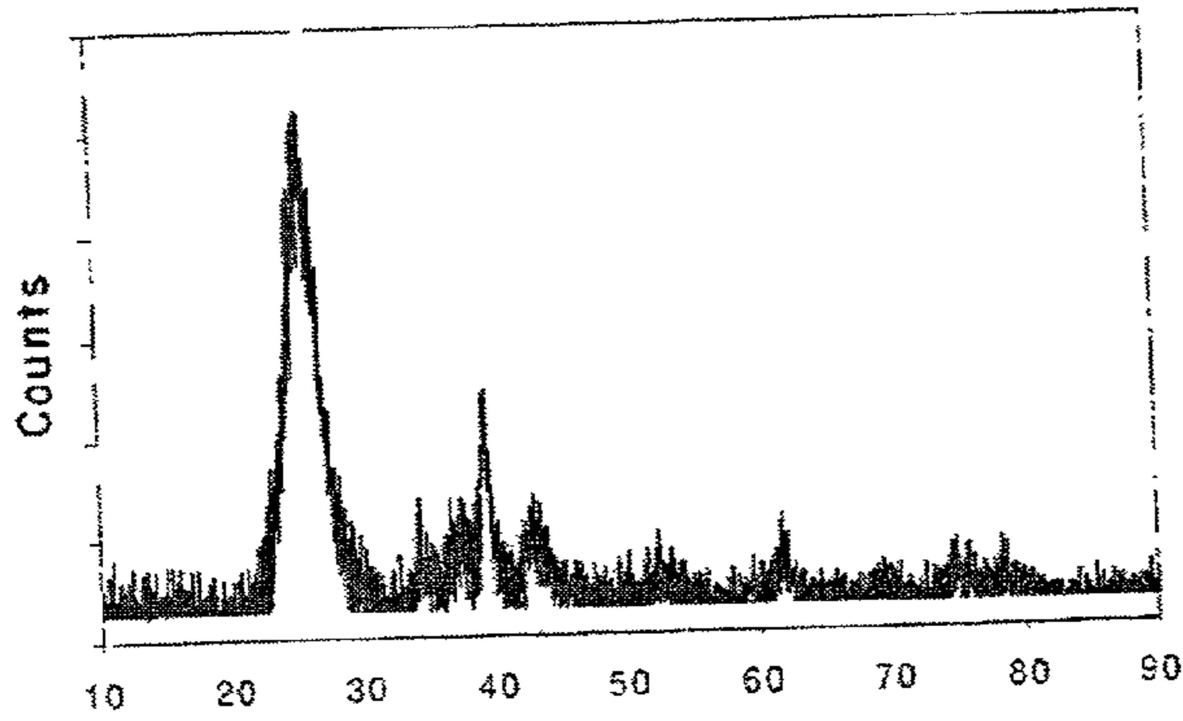
Reference XRD Pattern, hexagonal Mo 2 C
