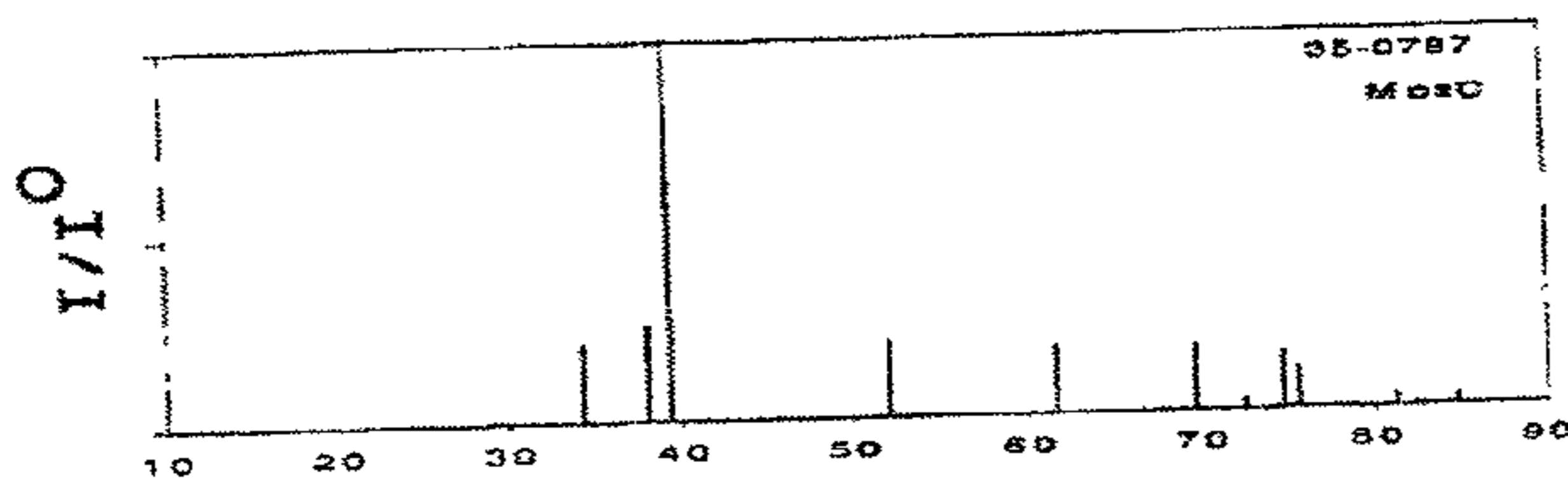
Reference XRD Pattern, cubic Mo 2 C
