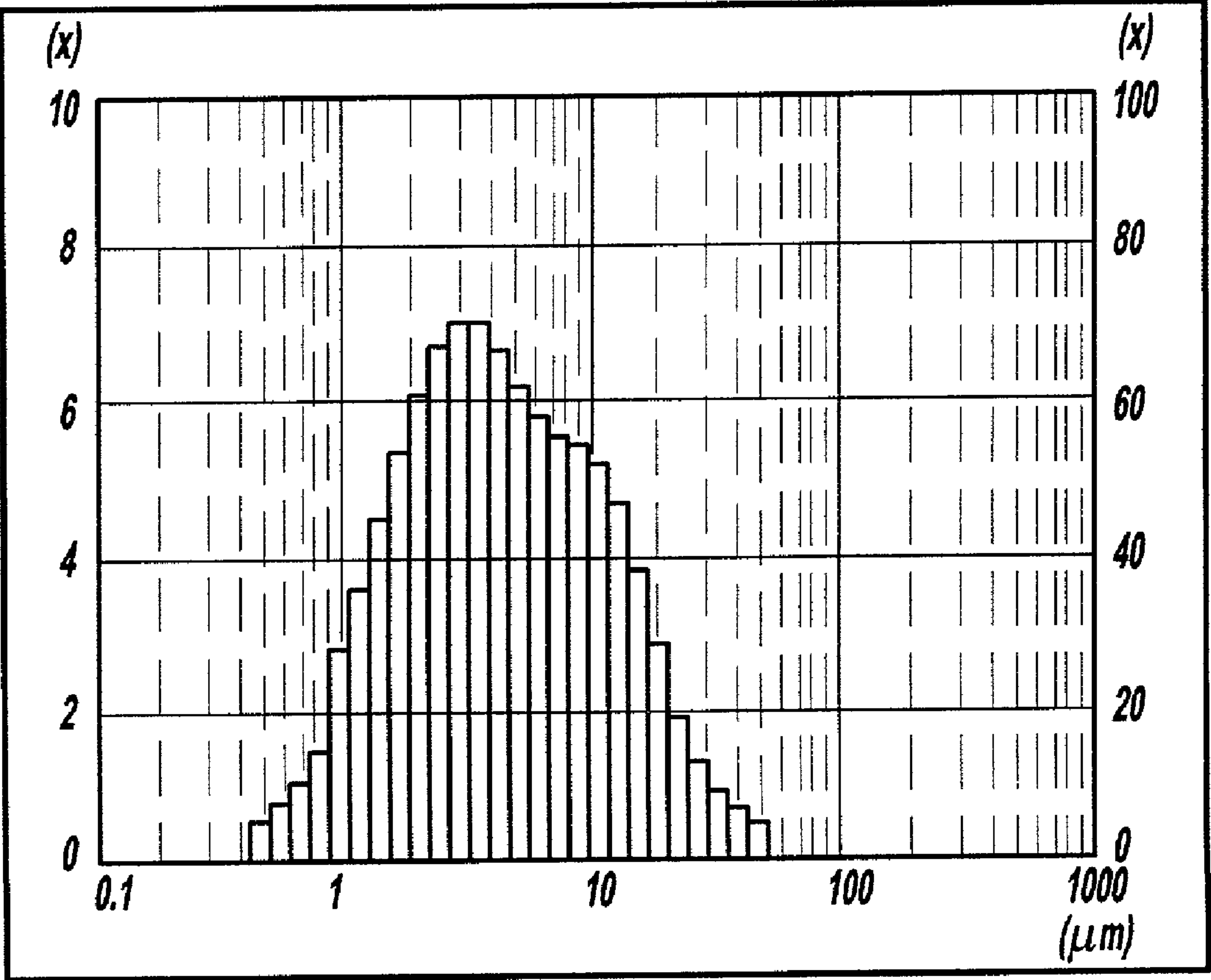
Particle Distribution of Hard Carbon
