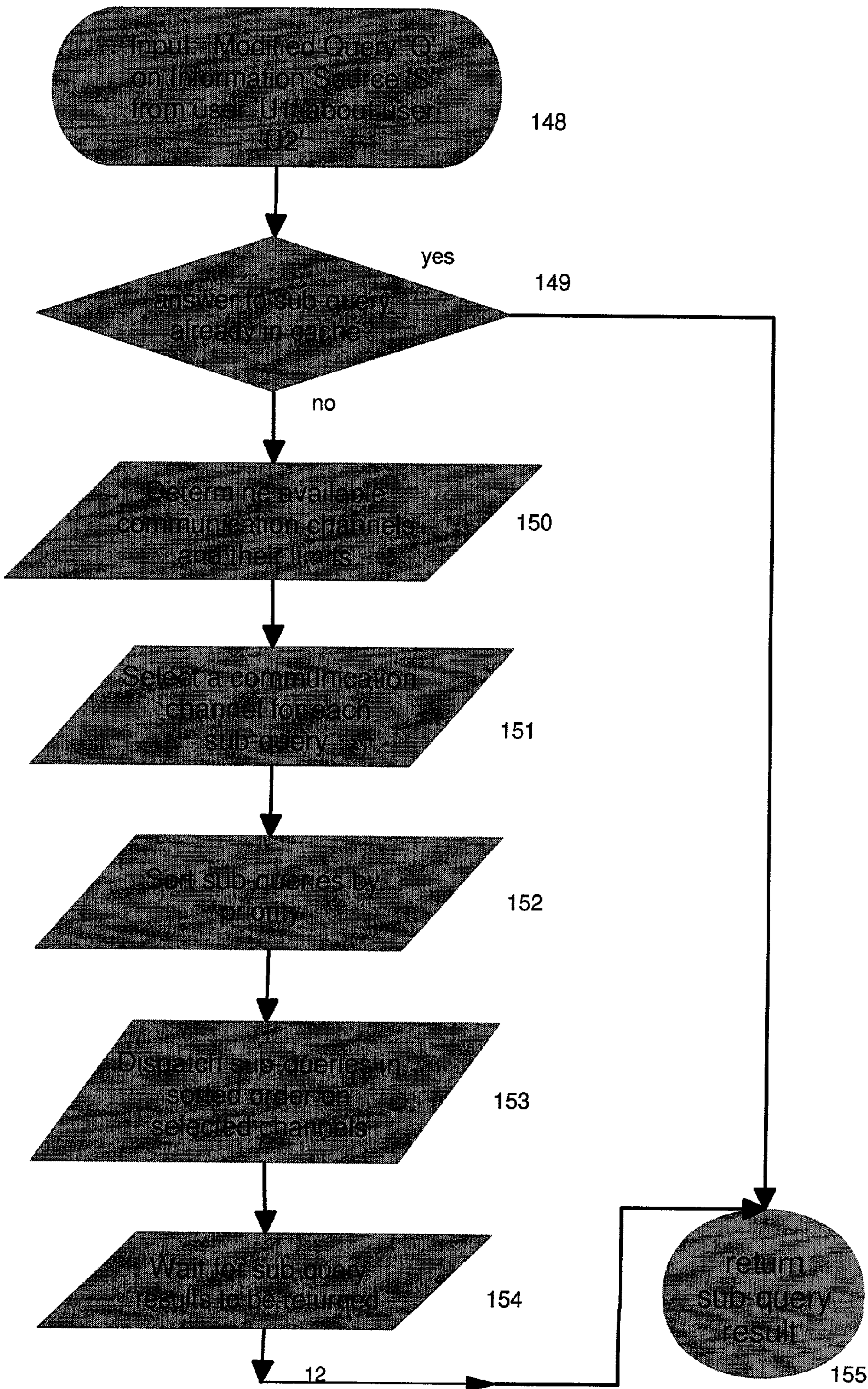
Figure 11 - Execute Query
