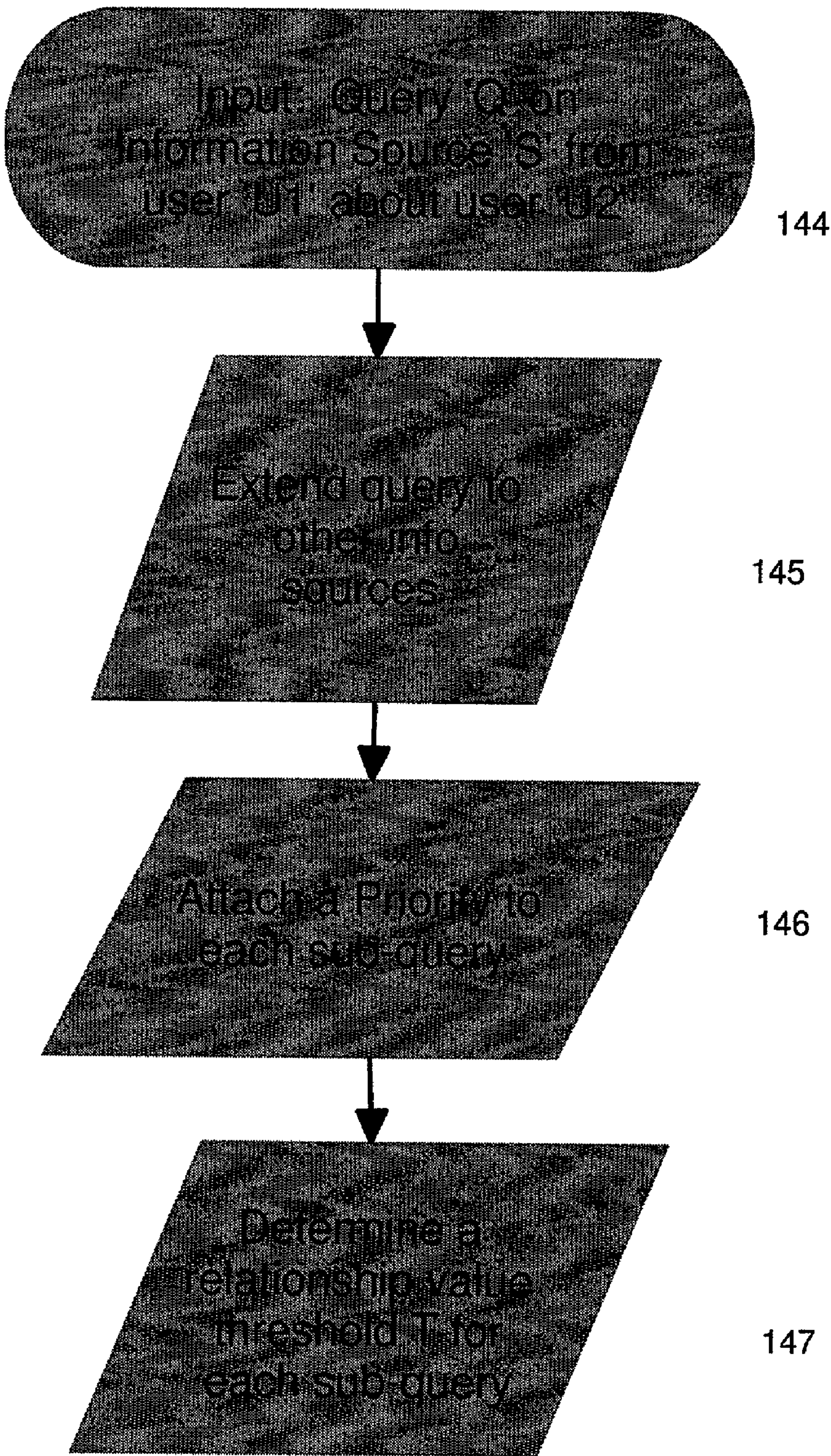
Figure 10 - Modify Query
