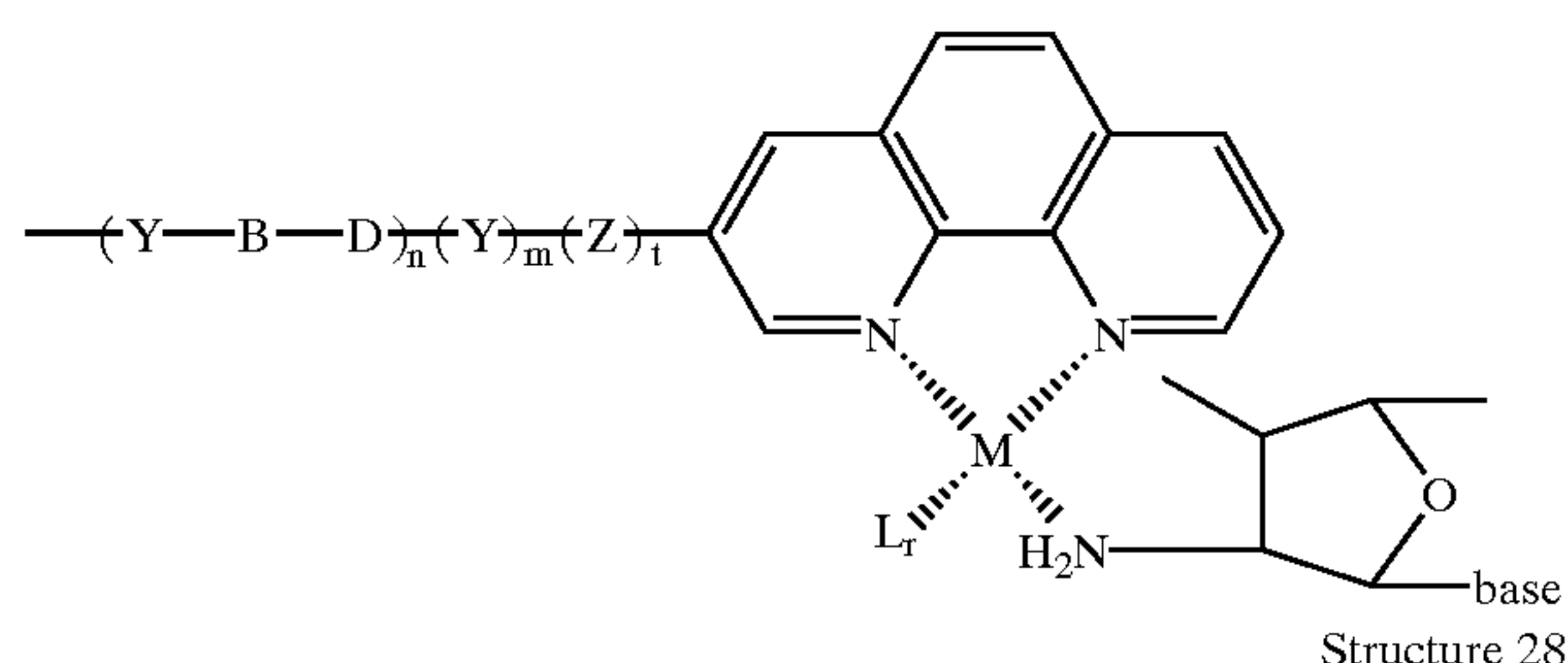
Structure 28
