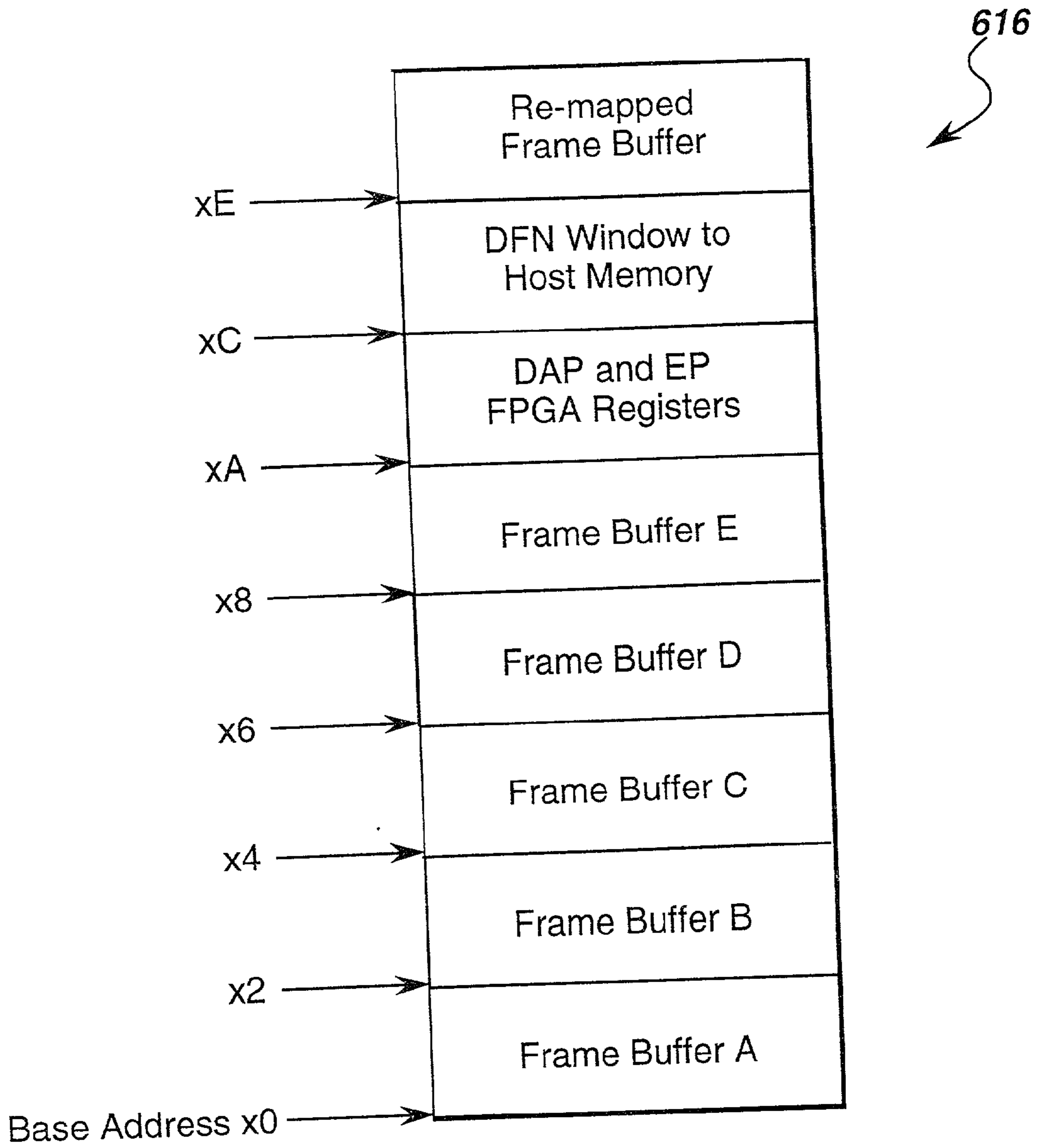
Mapping of 16 MByte PCI Address Space
