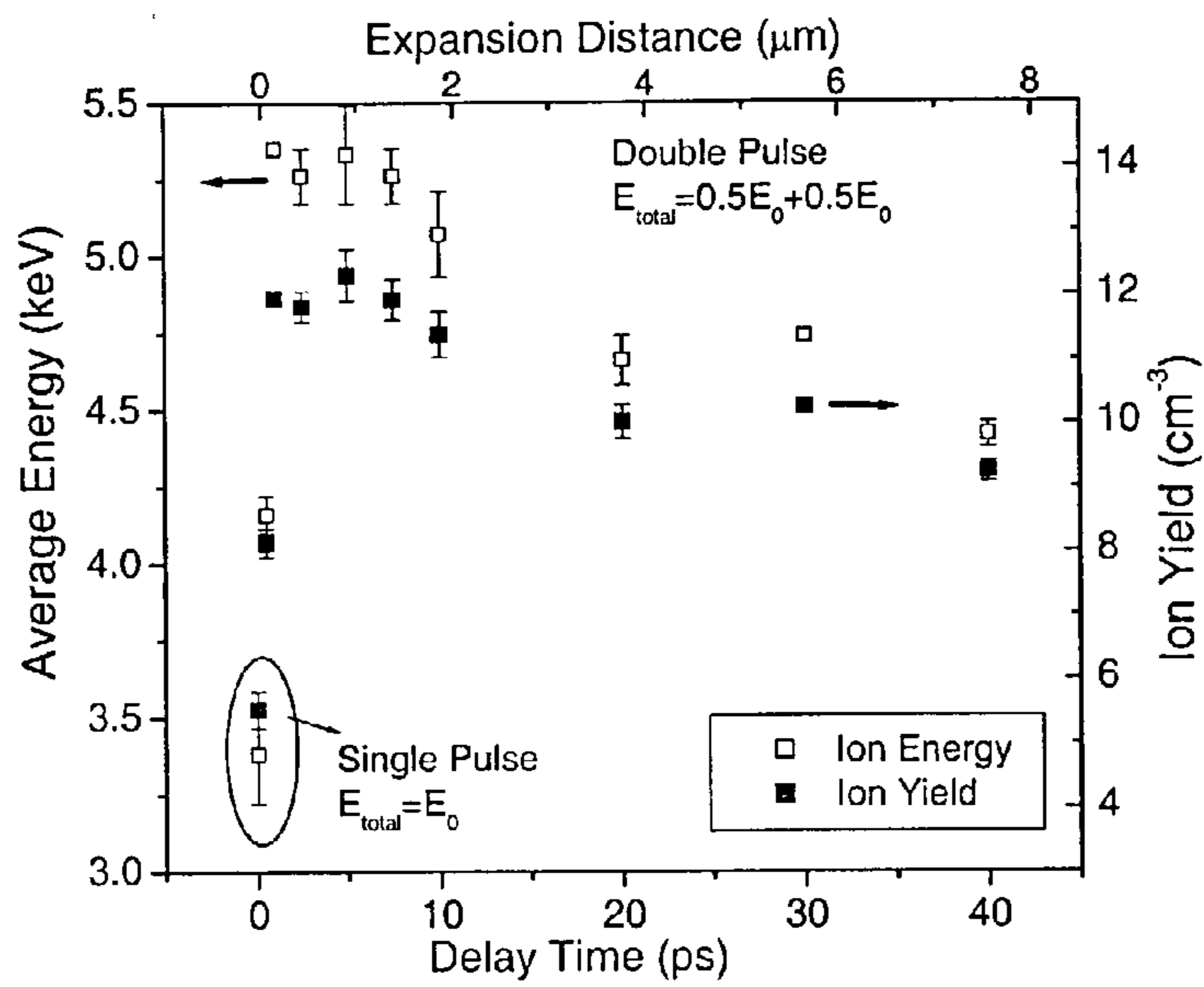
Fig 1. Average ion yield and energy as a function of time-delay between two identical 120 femtosecond ablation pulses on silicon. The single pulse at zero delay has an energy fluence of 2.2 kJ/cm 2 on a beam spot diameter of 42 microns. The two double pulses have a fluence of 1.1 kJ/cm 2 each. Expansion distance based on measured average ion velocity of 1.9x10 7 cm/s
