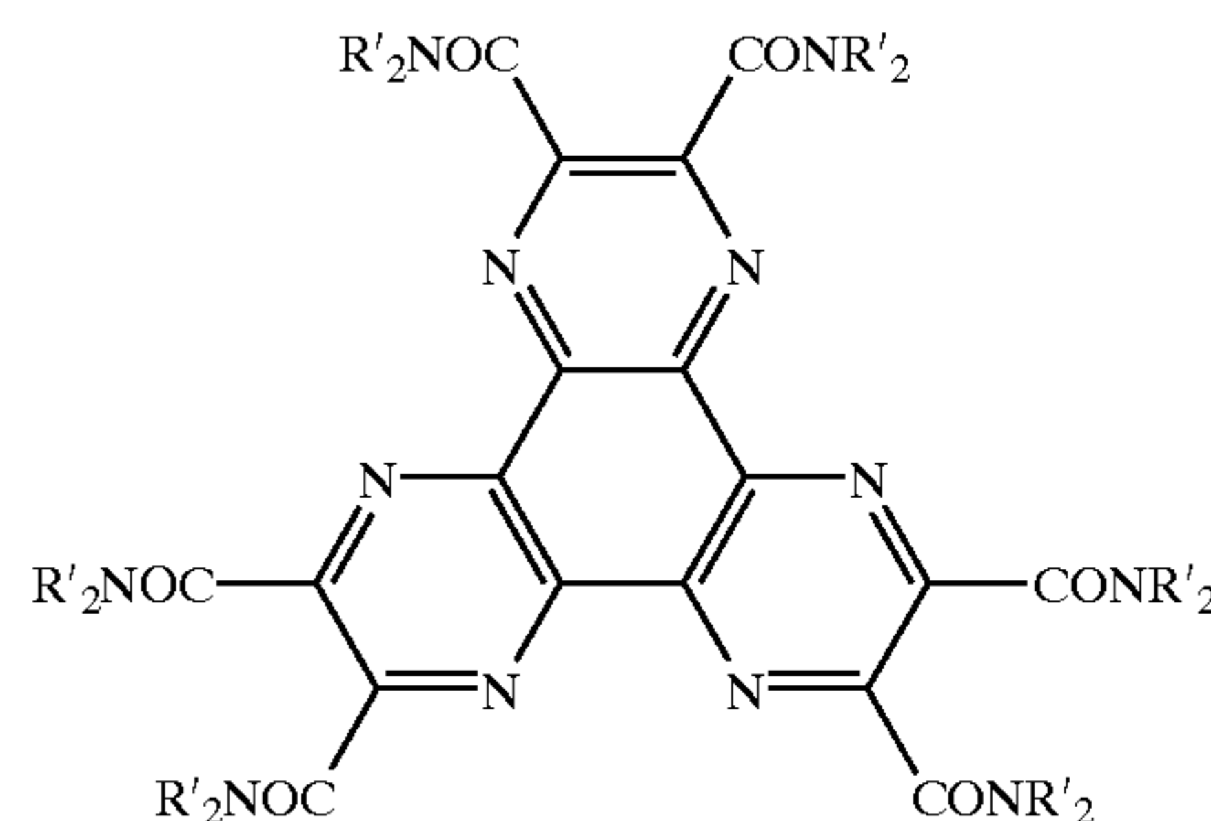
[Chemical Formula 1c]
