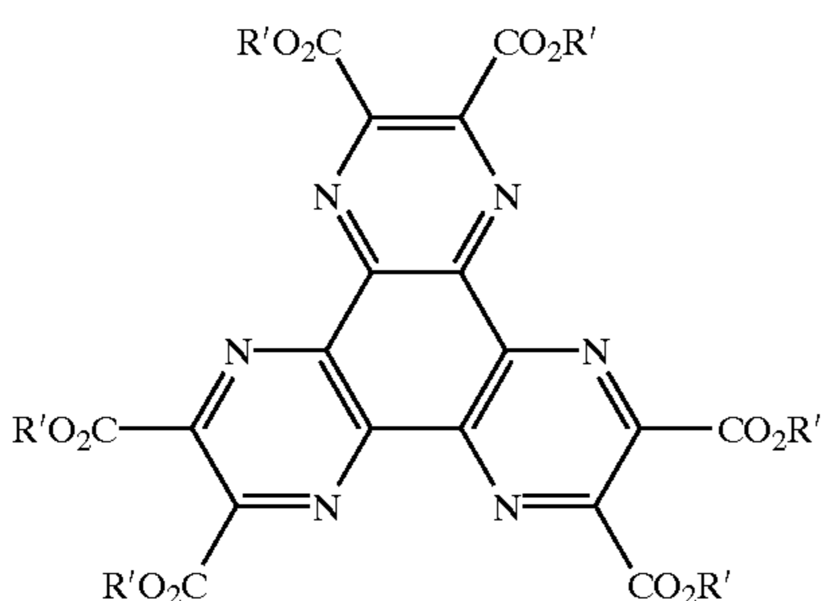
[Chemical Formula 1c]
