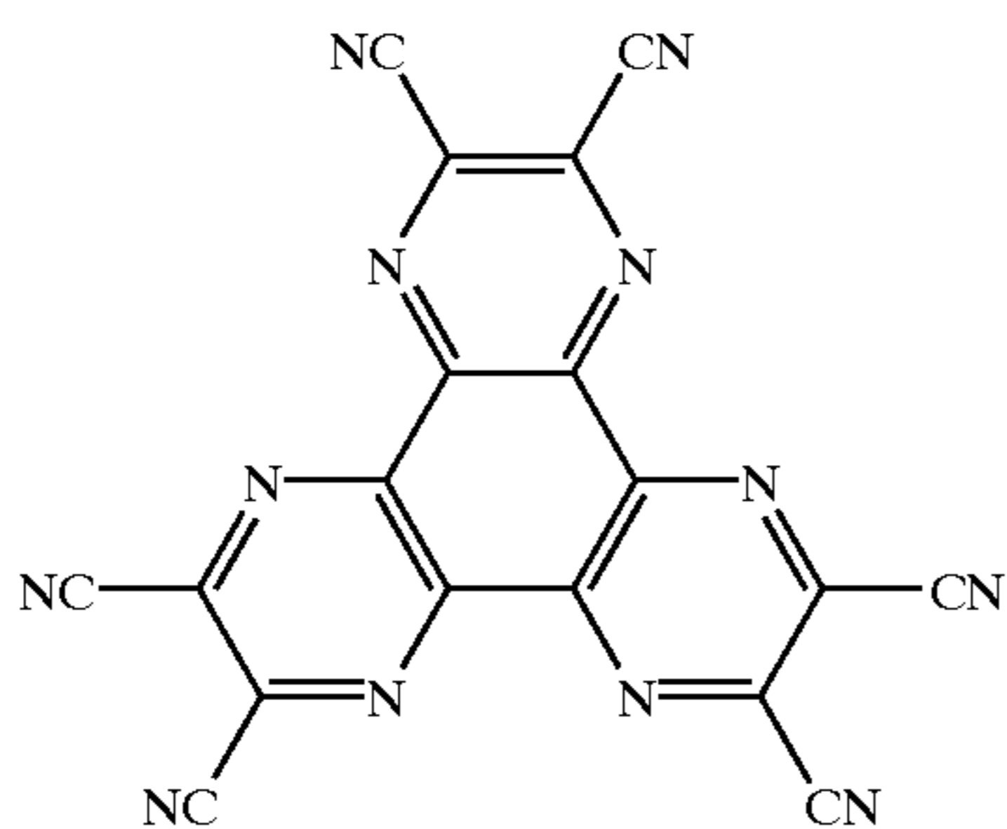
[Chemical Formula 1b]
