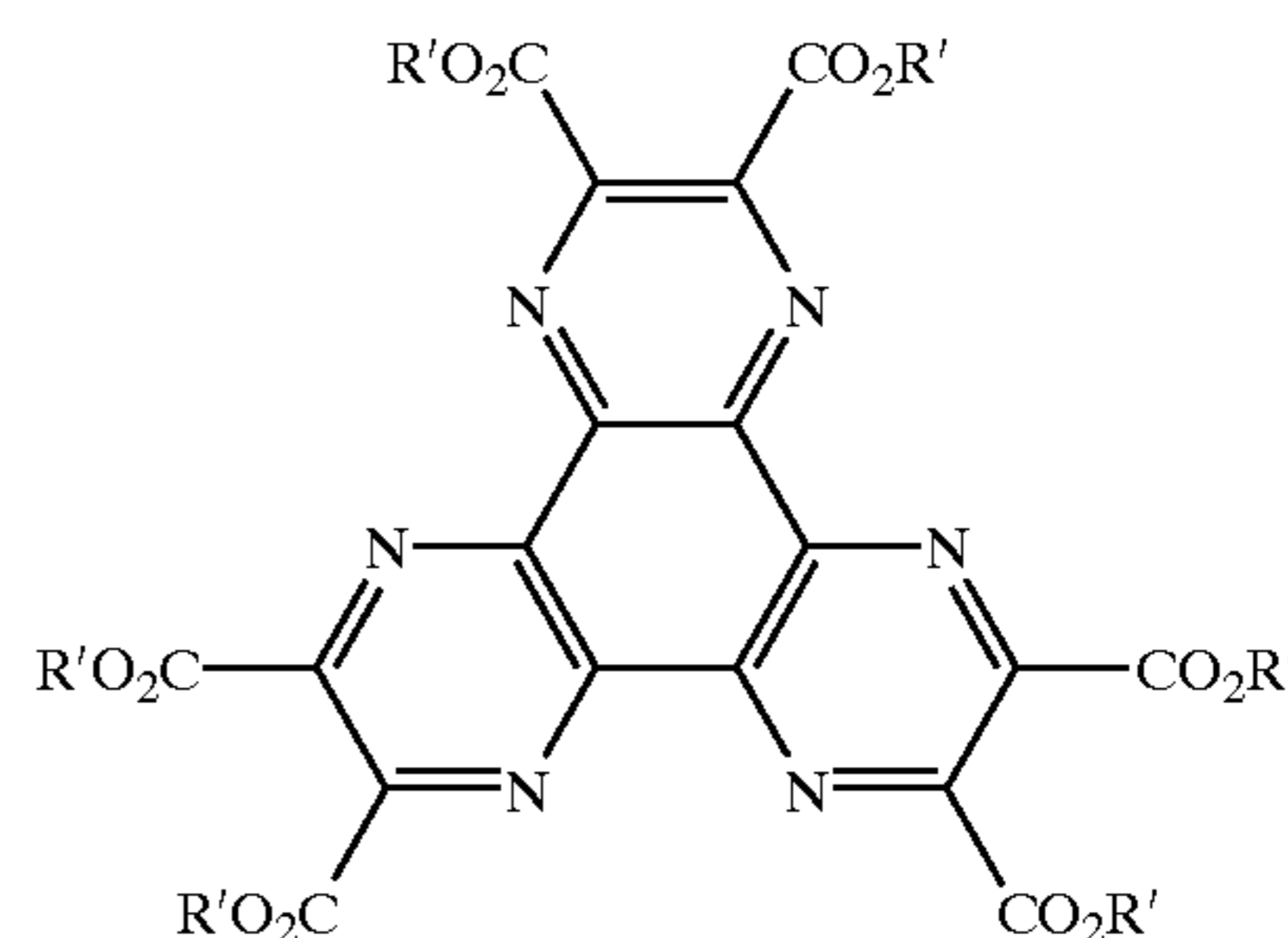
[Chemical Formula 1b]
