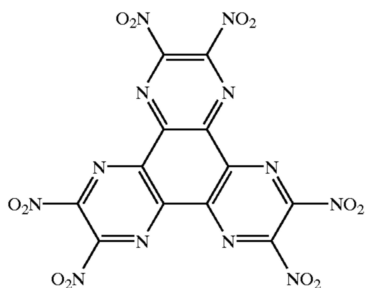
[Chemical Formula 1d]
