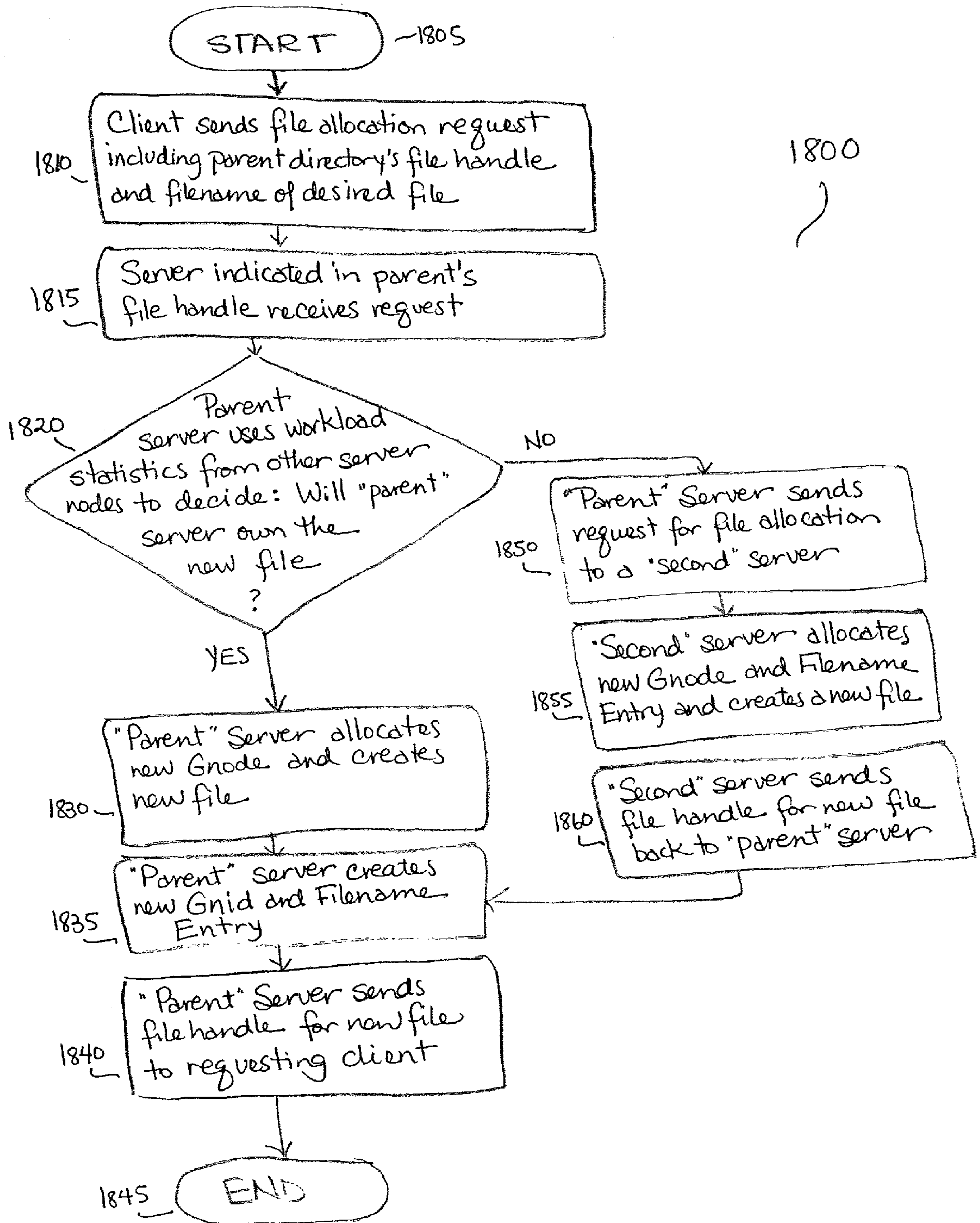
FIGURE 18 - File Allocation
