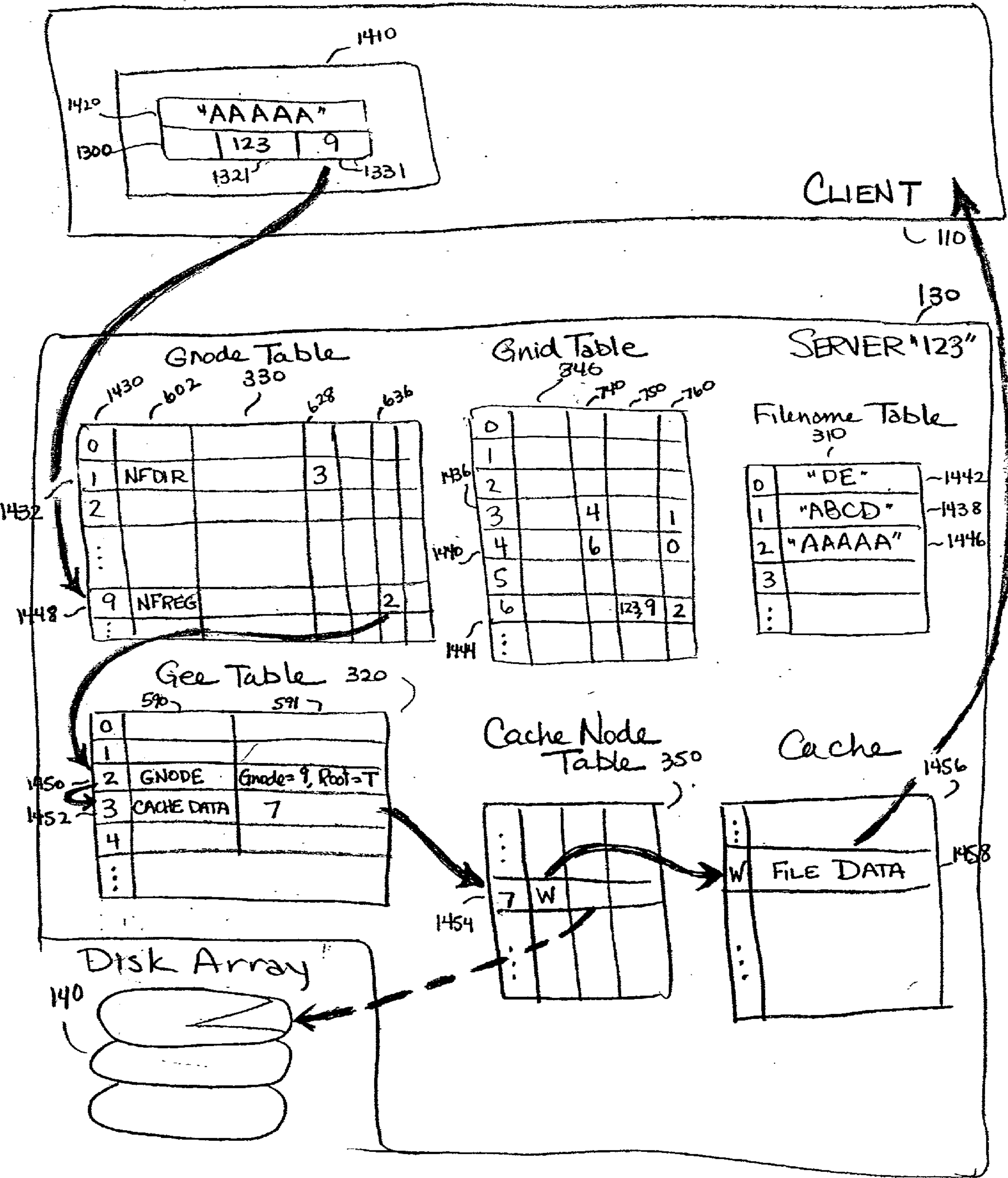
FIGURE 14b Example of a File Access
