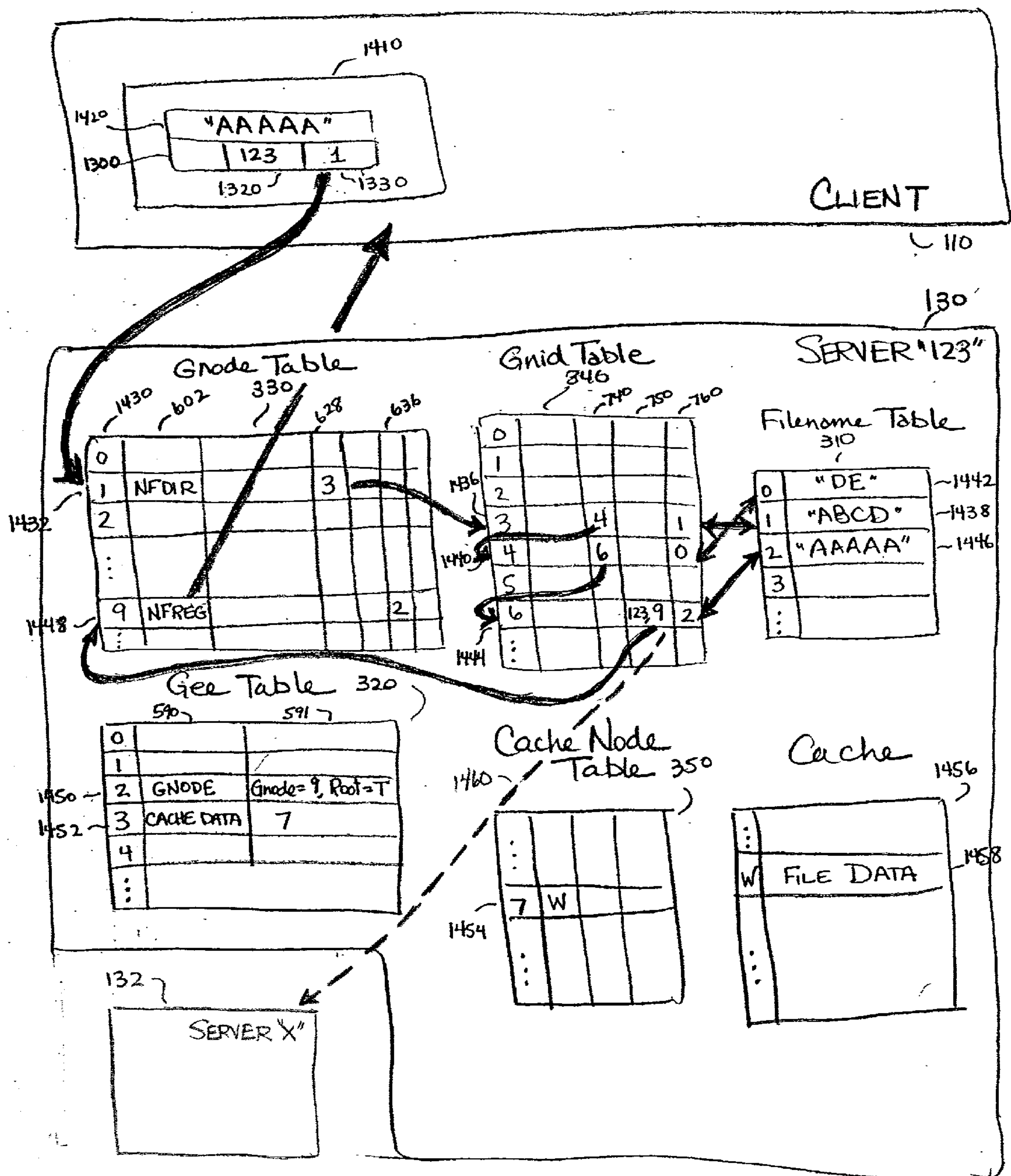
FIGURE 14a: Example of a File Look-Up
