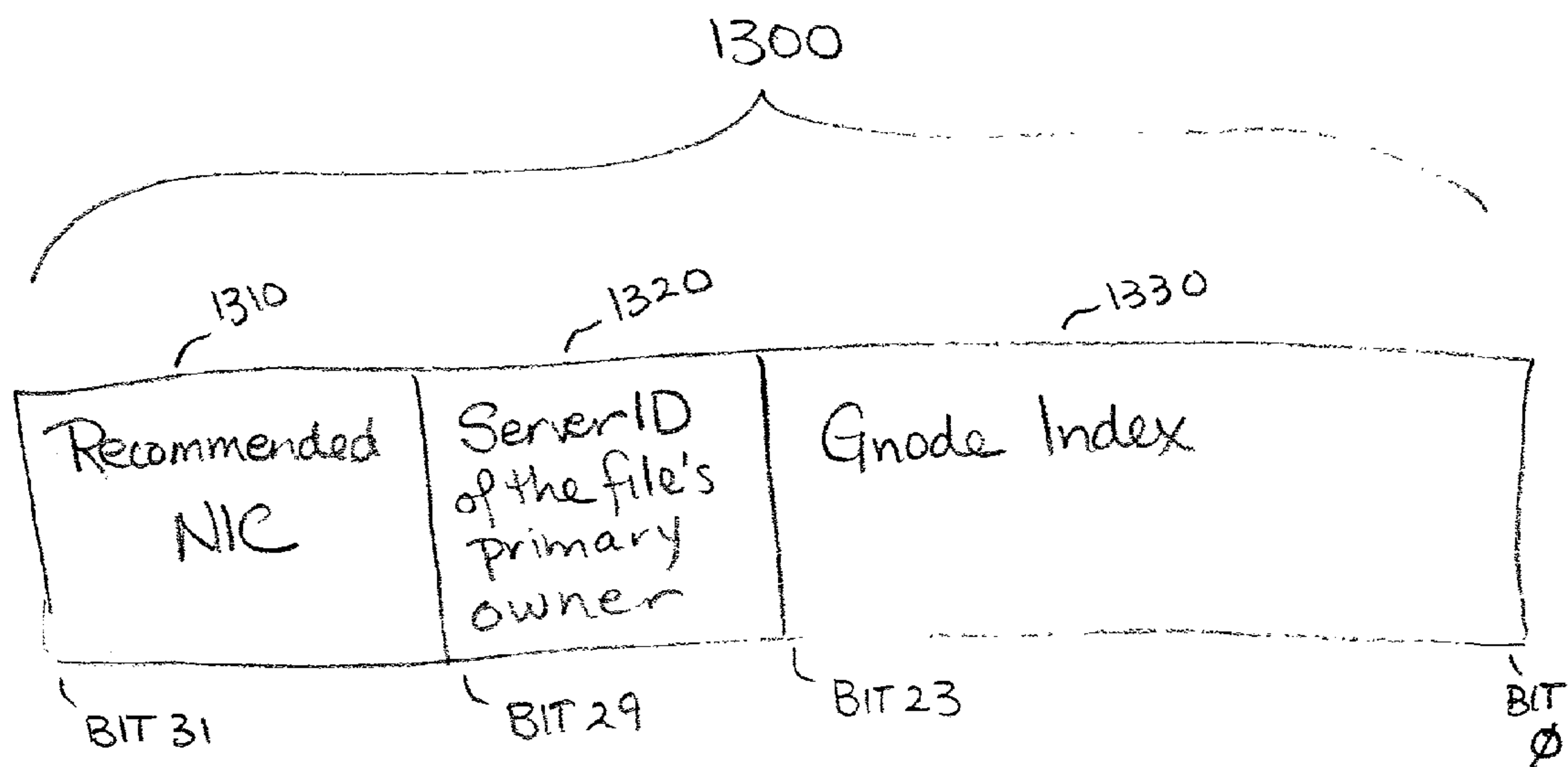
FIGURE 13 - Structure of a File Handle
