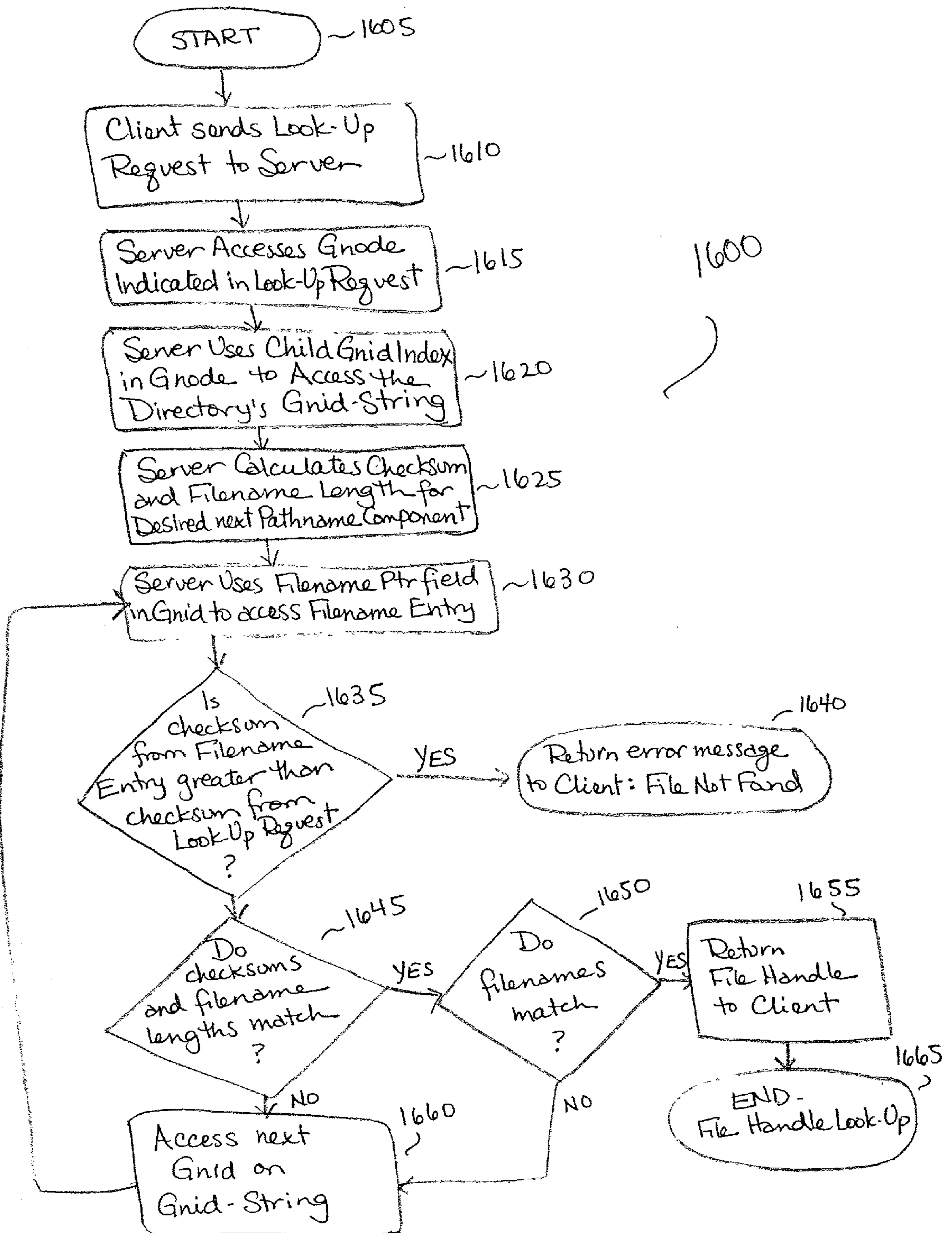
FIGURE 16: Performing a File Handle Look-Up
