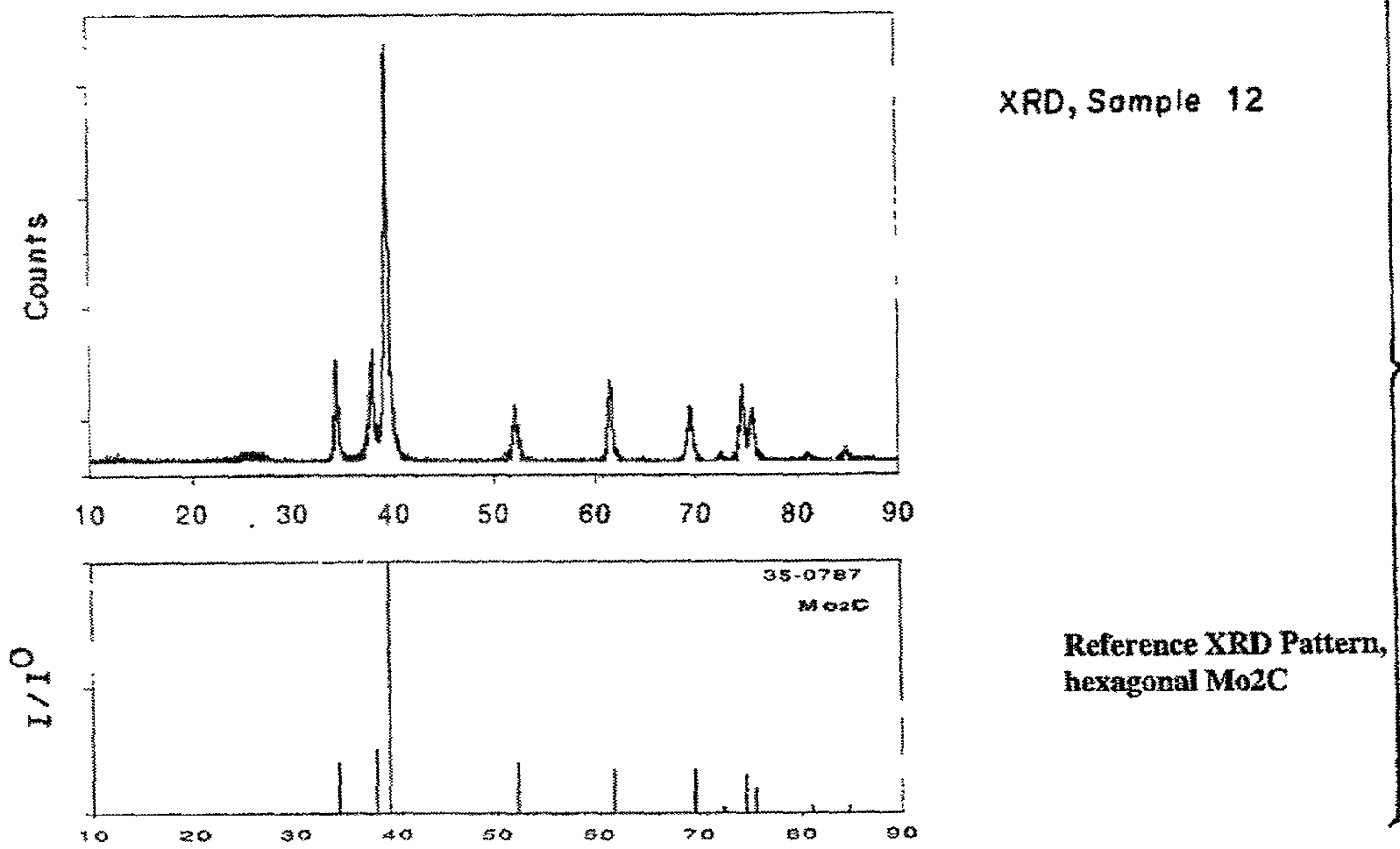
FIG.1A XRD and SEM of CARBIDE NANORODS
