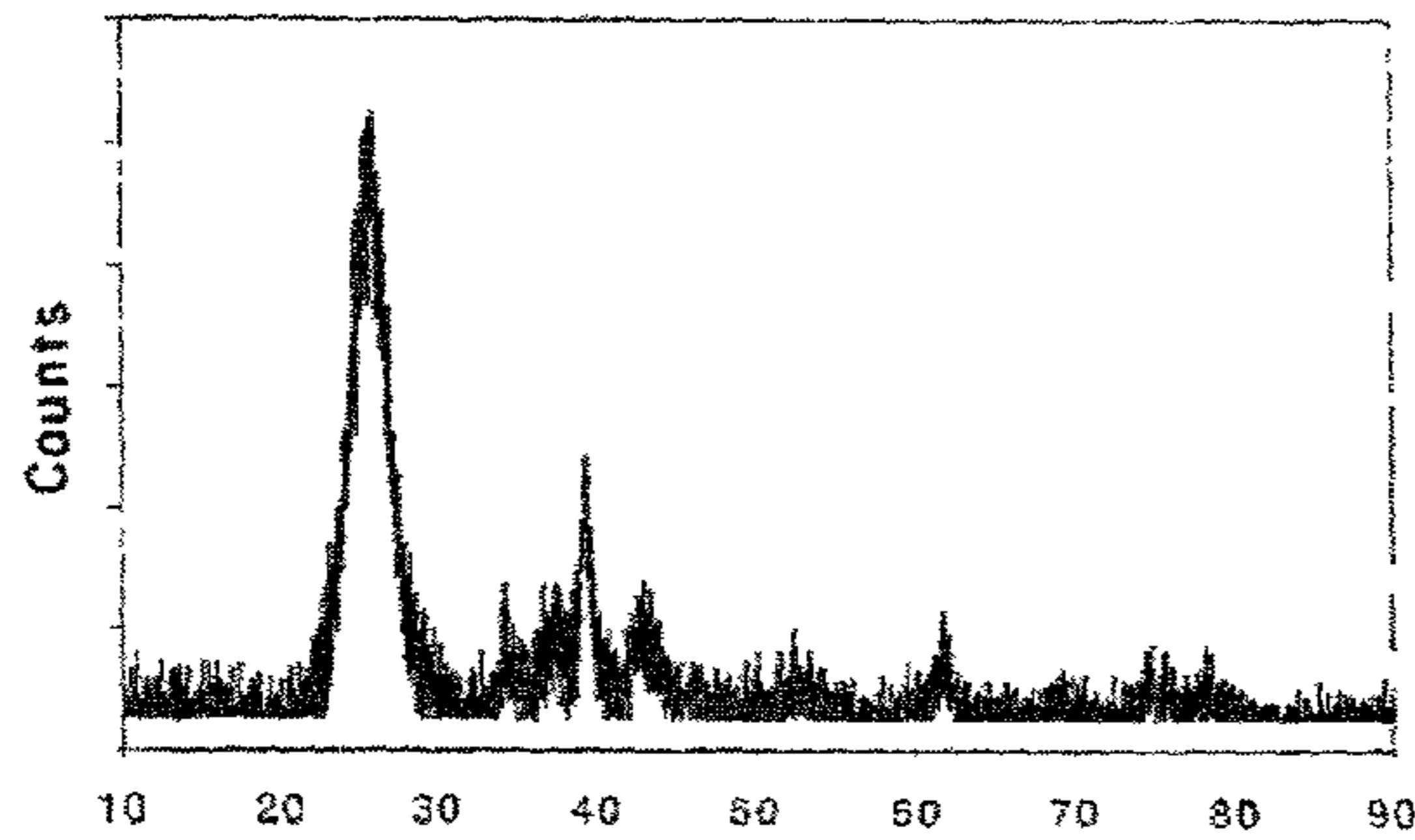
Reference XRD Pattern, hexagonal Mo 2 C
