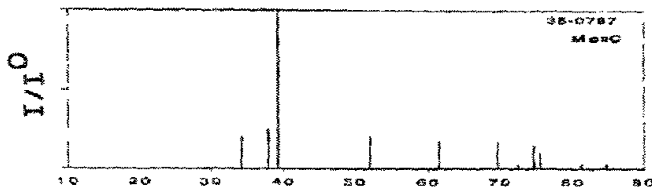
Reference XRD Pattern, cubic Mo 2 C
