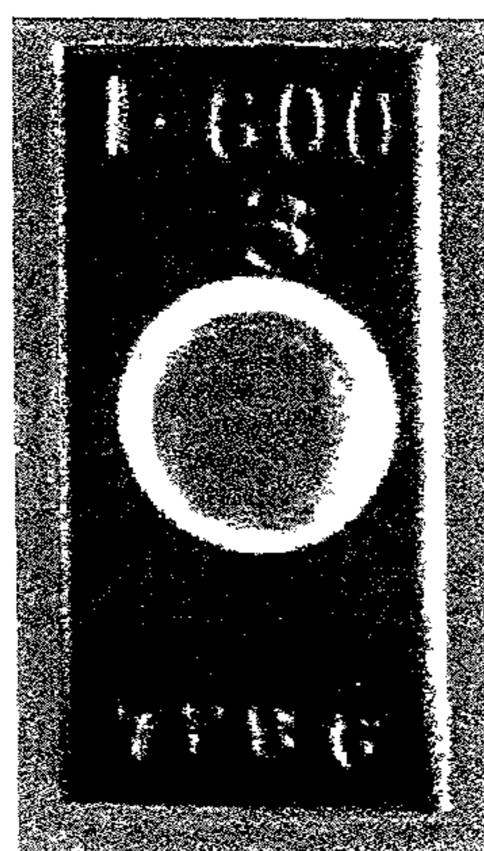
Fig. 22C 50 ppm H 2 S
