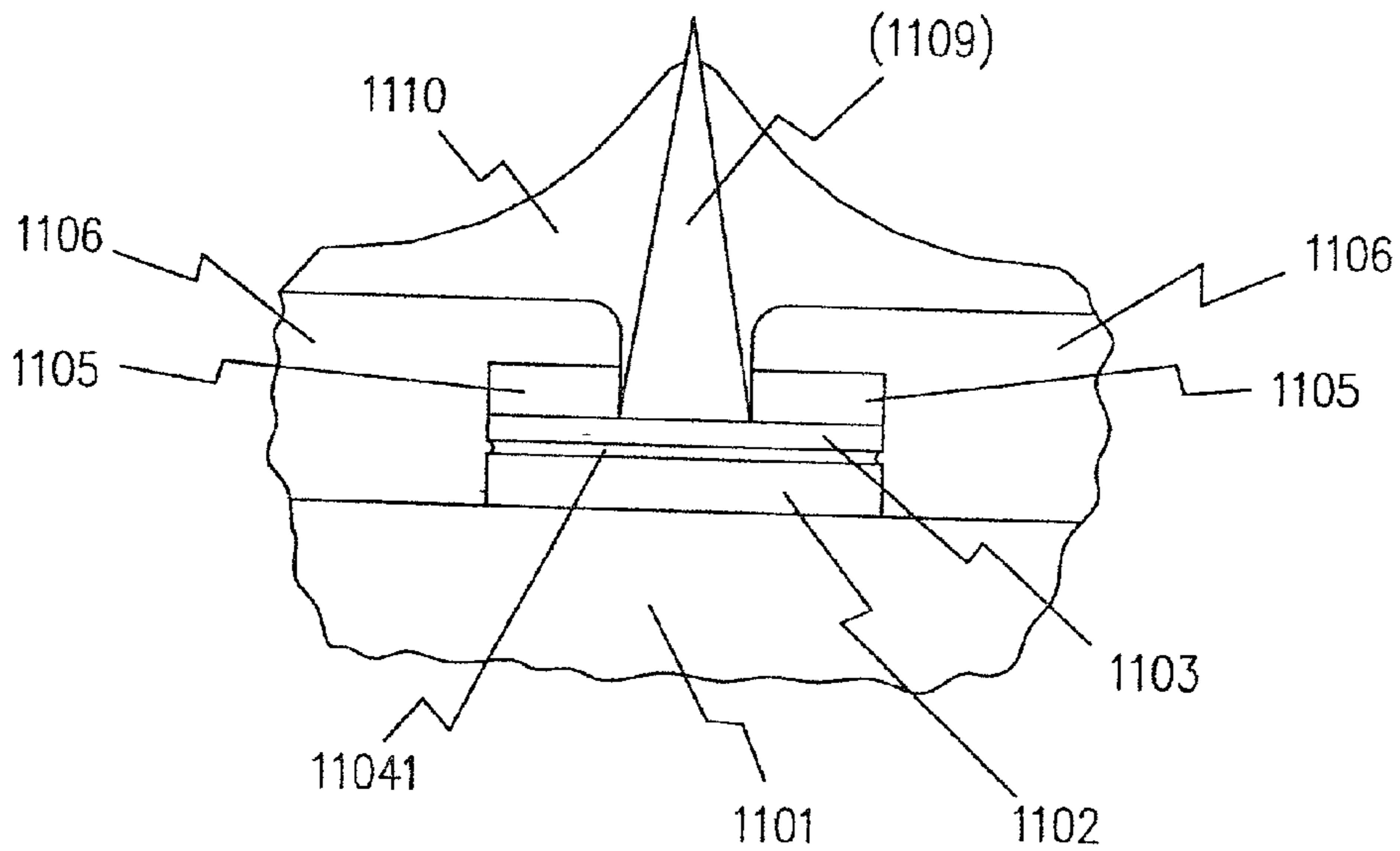
FIGURE 11b ELECTRODES
