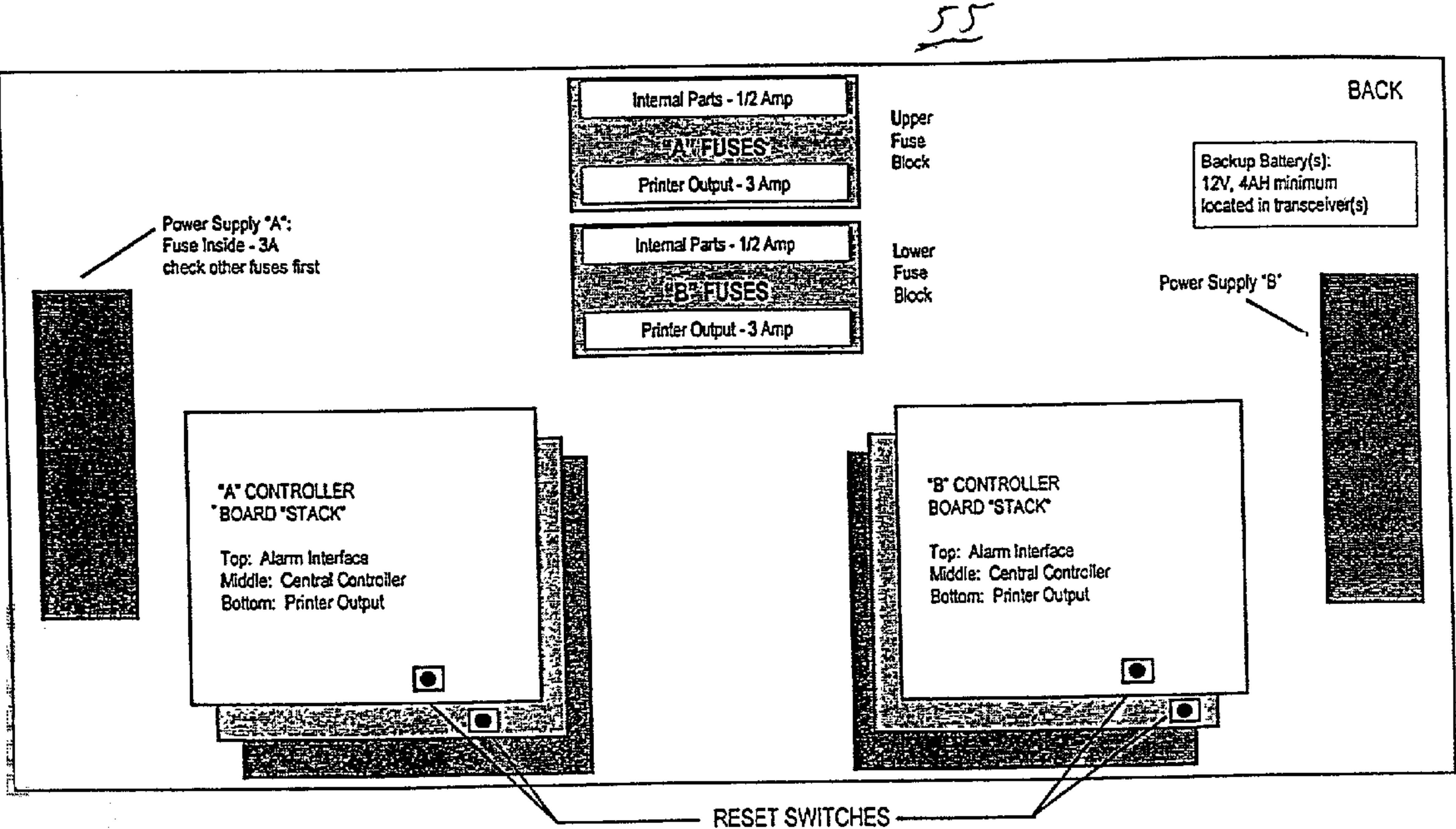
PC Board Key Components
