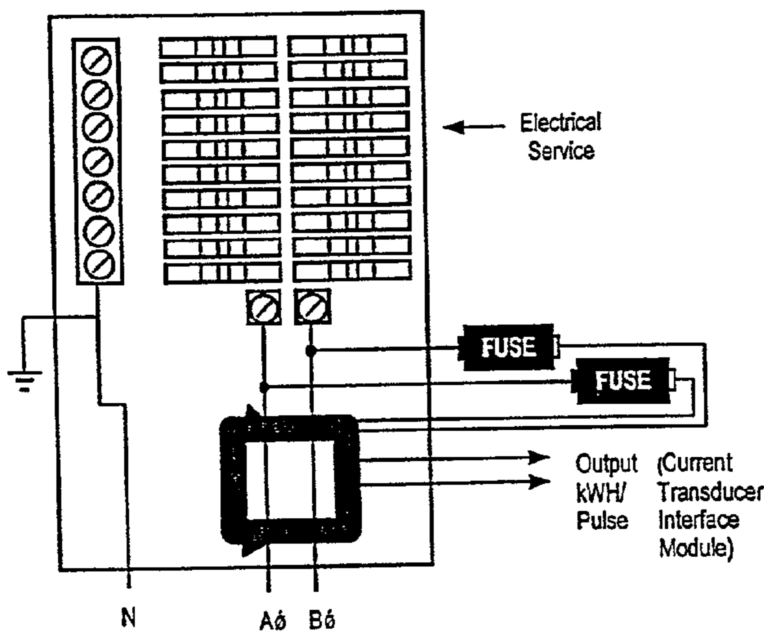
240V, 1Ø, 2-Wire Connection
