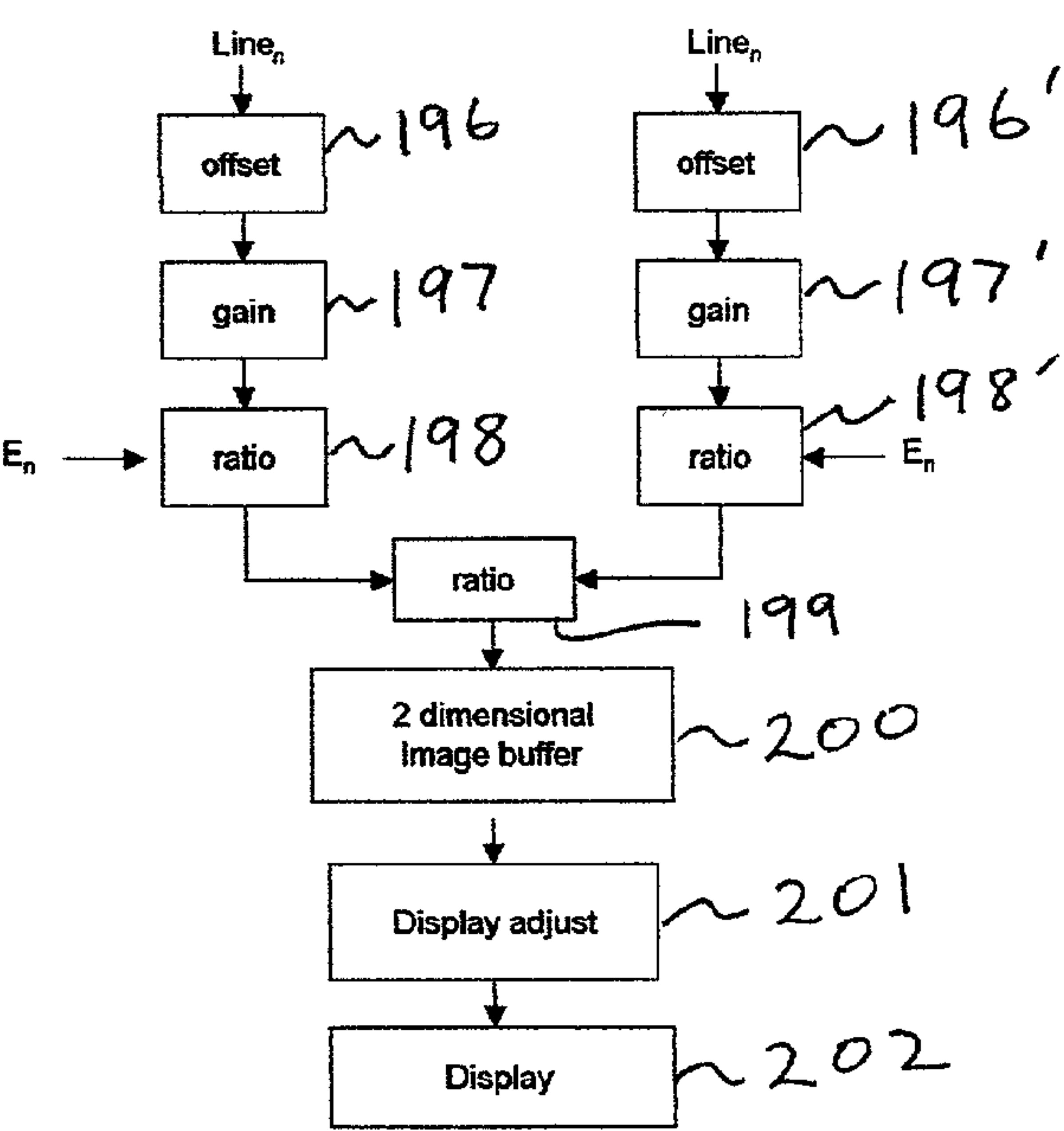
Differential mode
