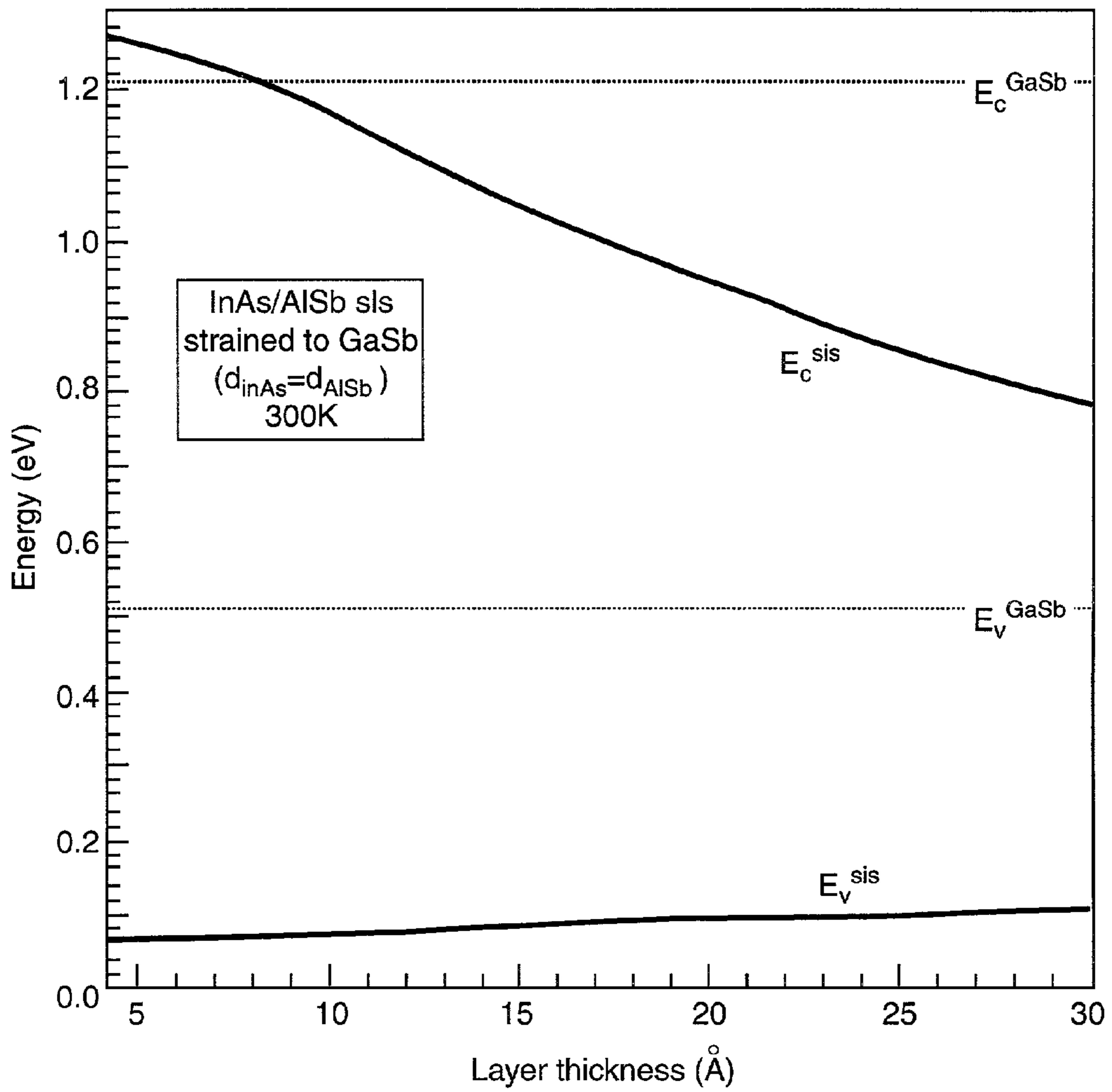
FIG. 1 Conduction and valence band edges of an InAs/AlSb Superlattice as a function of constituent layer thicknesses. GaSb band edges are shown for reference.
