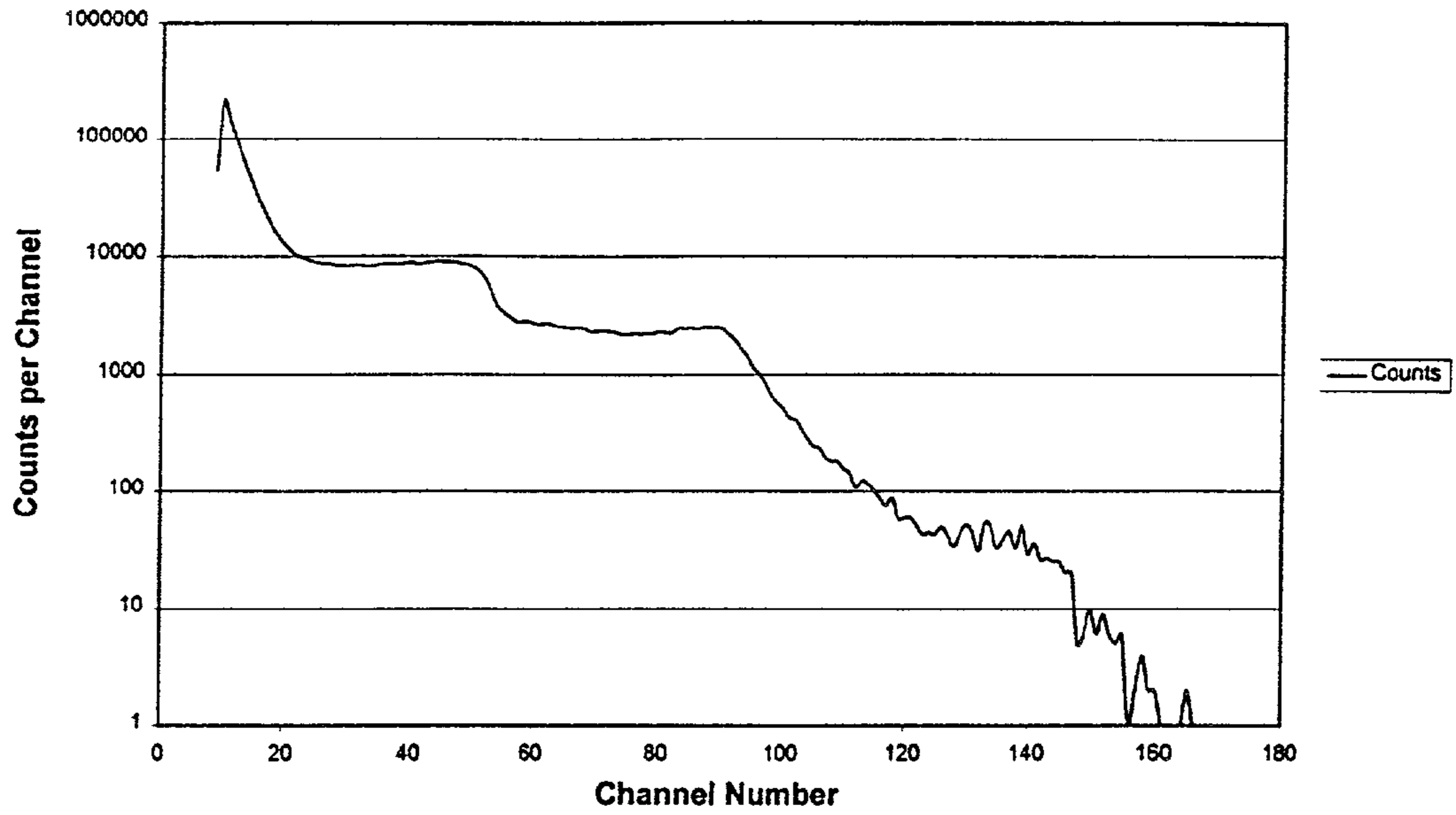
Pulse Height Spectrum for SBD (Line of sight center channel Pu-Be source, 2850 second count.)
