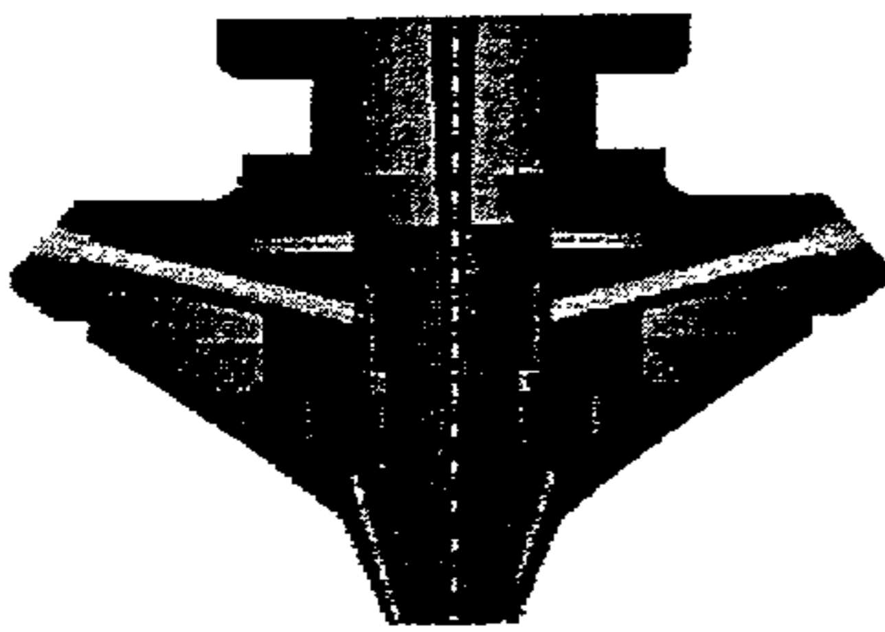
DMD Nozzle - 28.0 mm Stand-off
