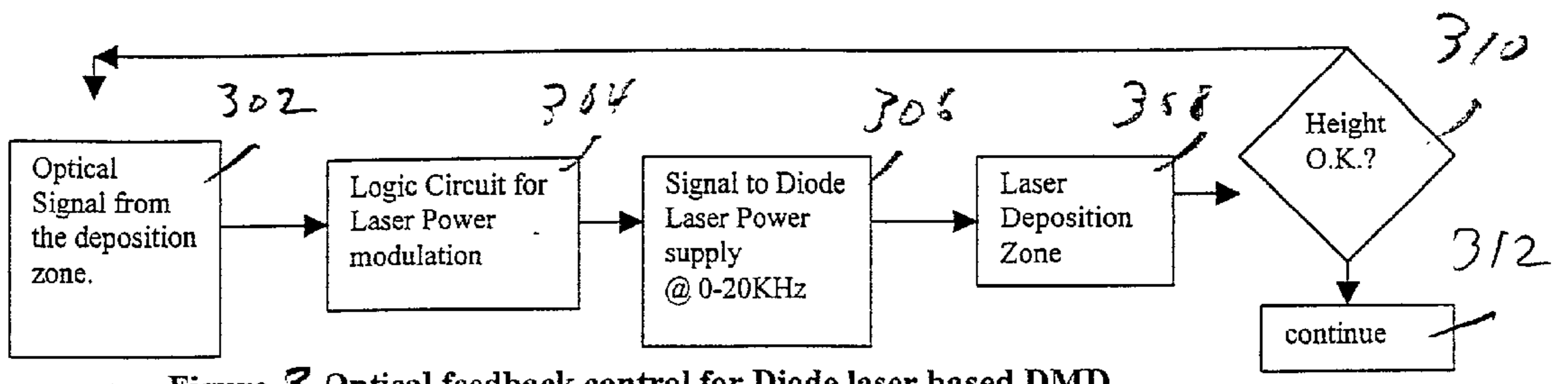
Figure 3 Optical feedback control for Diode laser based DMD
