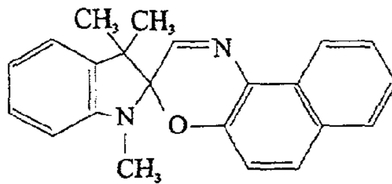
1,3-Dihydro-1,3,3-trimethylspiro[2 H -indole-2,3'-[3 H ]naphth[2,1- b ][1,4]oxazine]
