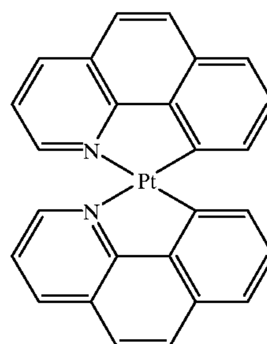
cis-Bis[benzo(h)quinolinato-N,C]Pt(II) Pt(Bhq) 2 (3)
