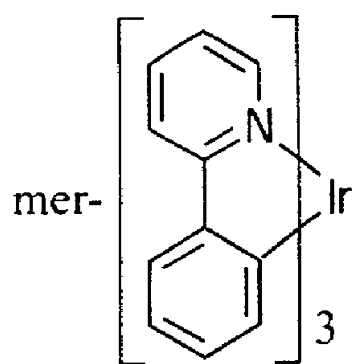
mer-Irppy
