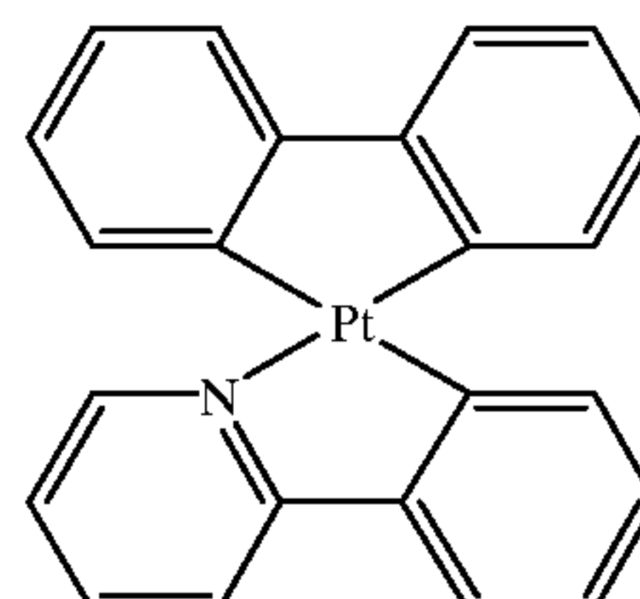
(Biphenylinato-C,C)-(bipyridinato-N,N)Pt(II) Pt(bph)(bpy)(4)
