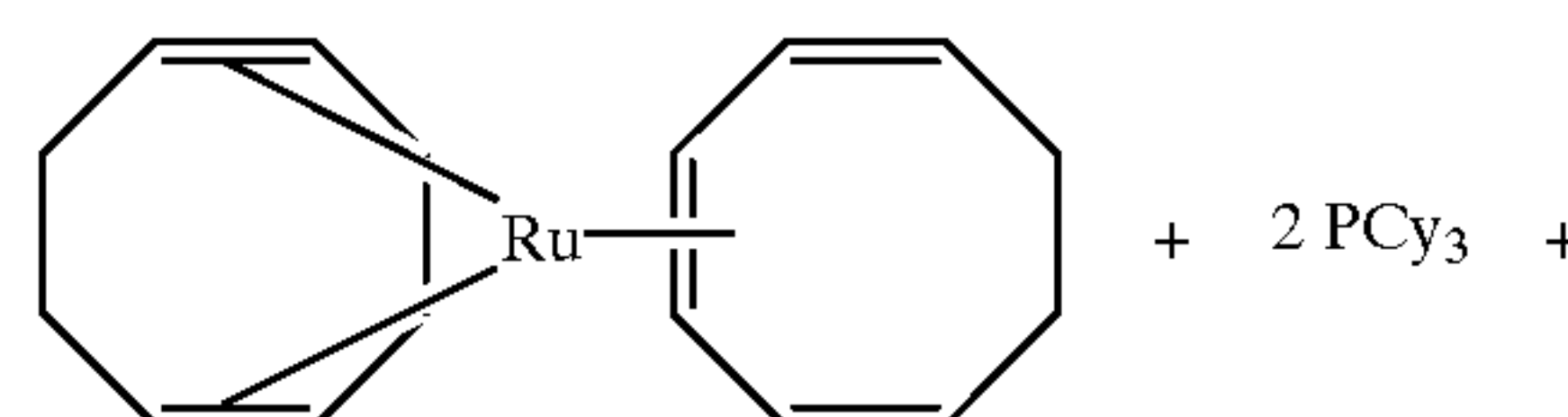
REACTION SCHEME 4
