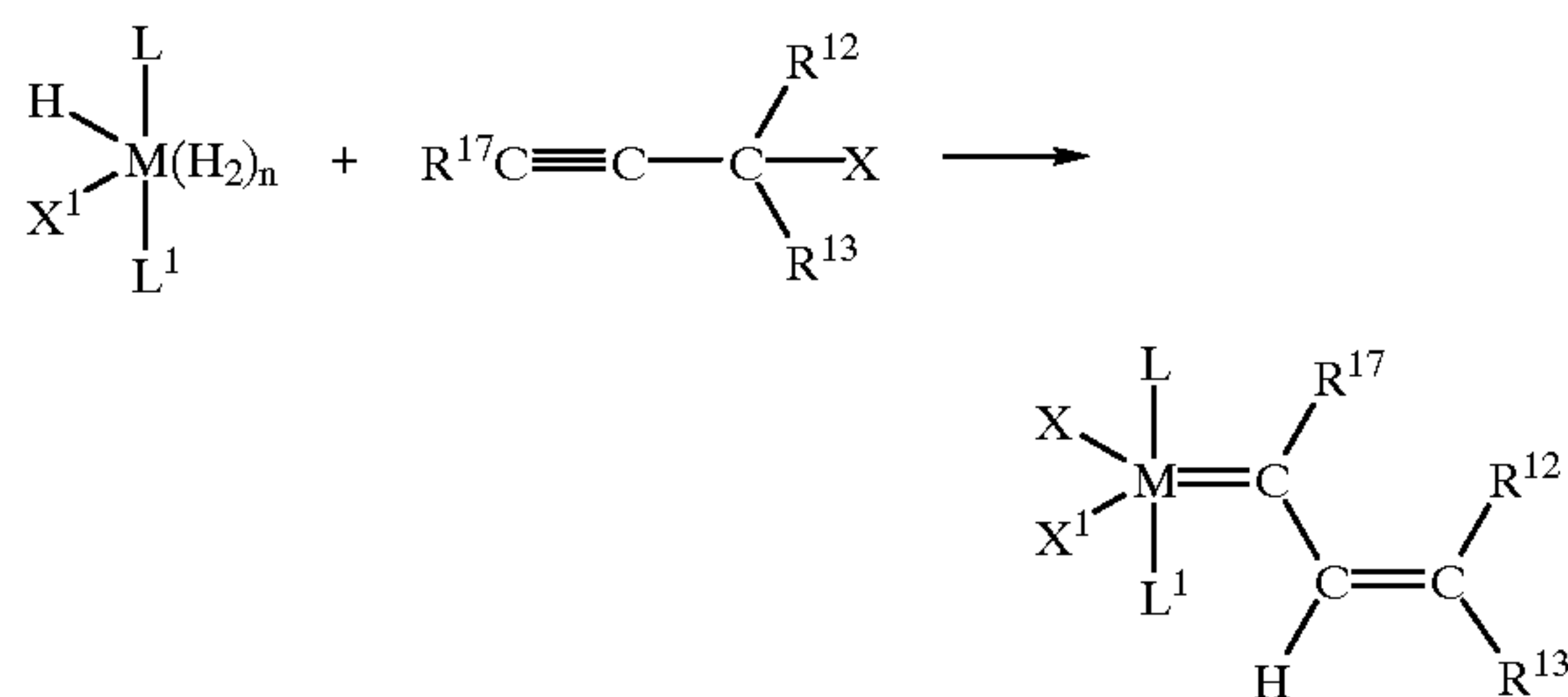
REACTION SCHEME 2
