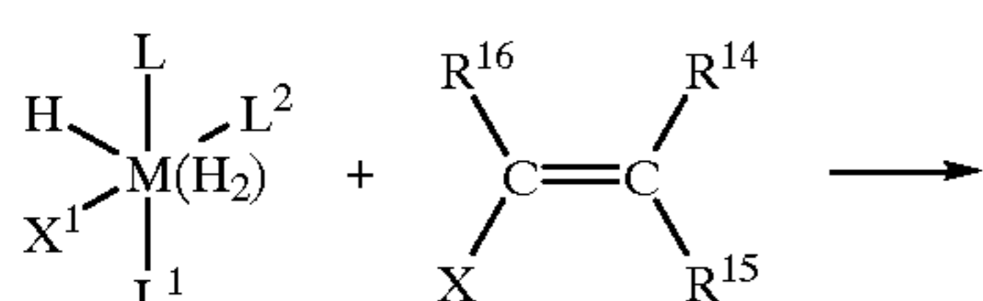
REACTION SCHEME 3A
