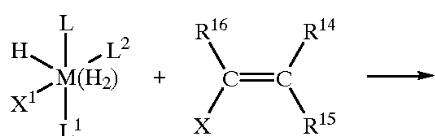
REACTION SCHEME 3A
