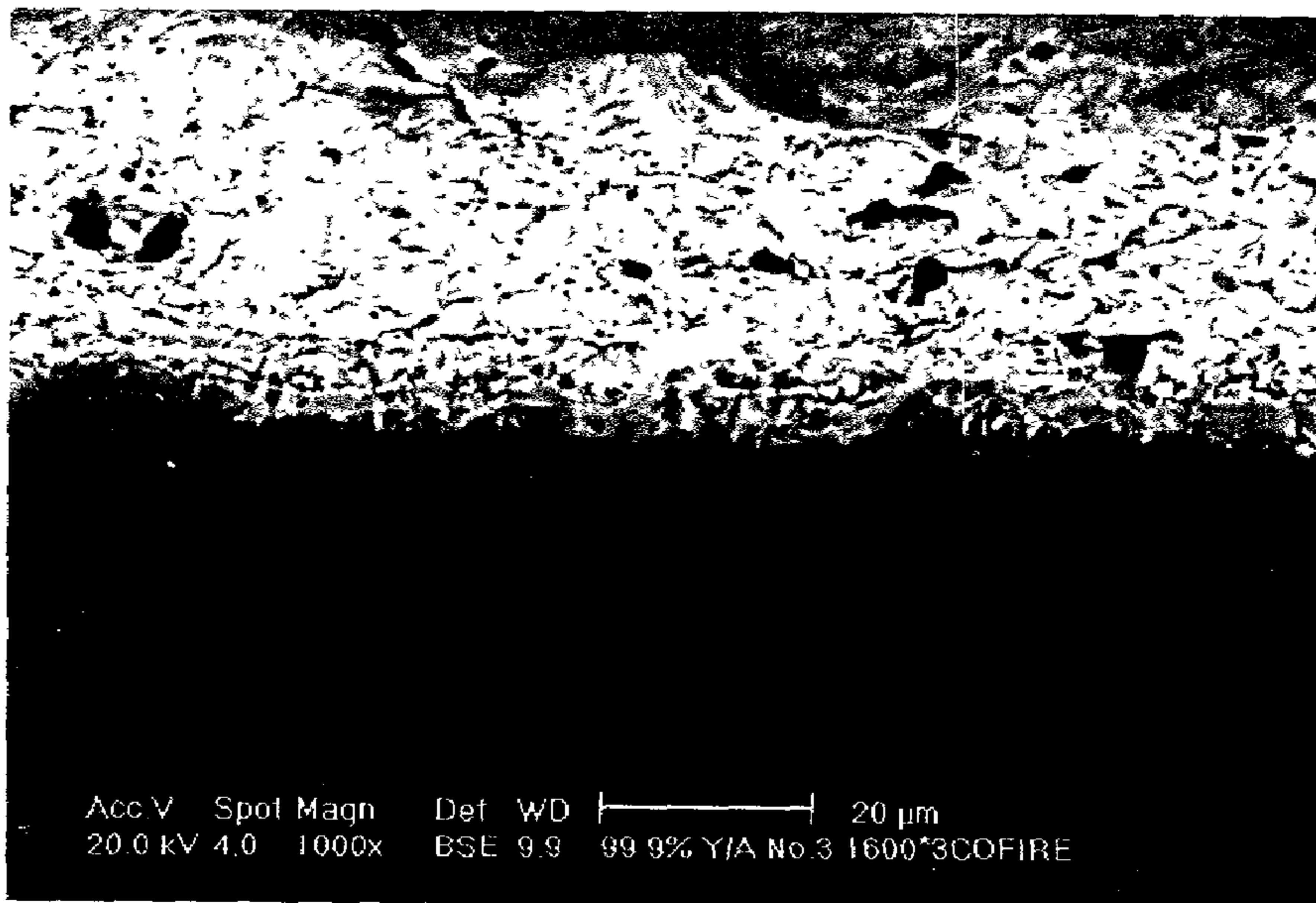
Surface of 1600°C Co-sintered product (×1000)
