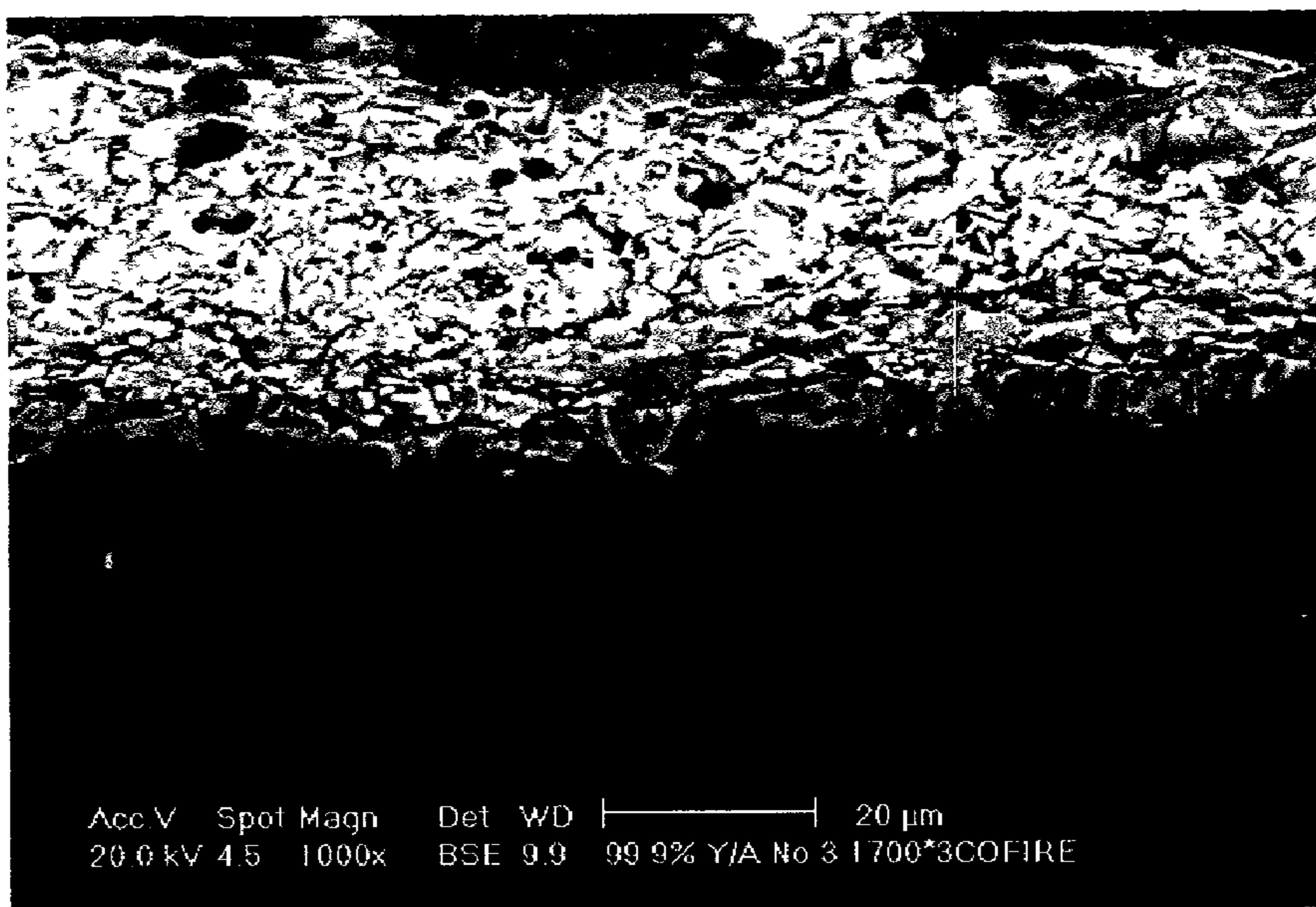
Surface of 1700°C Co-sintered product (X1000)
