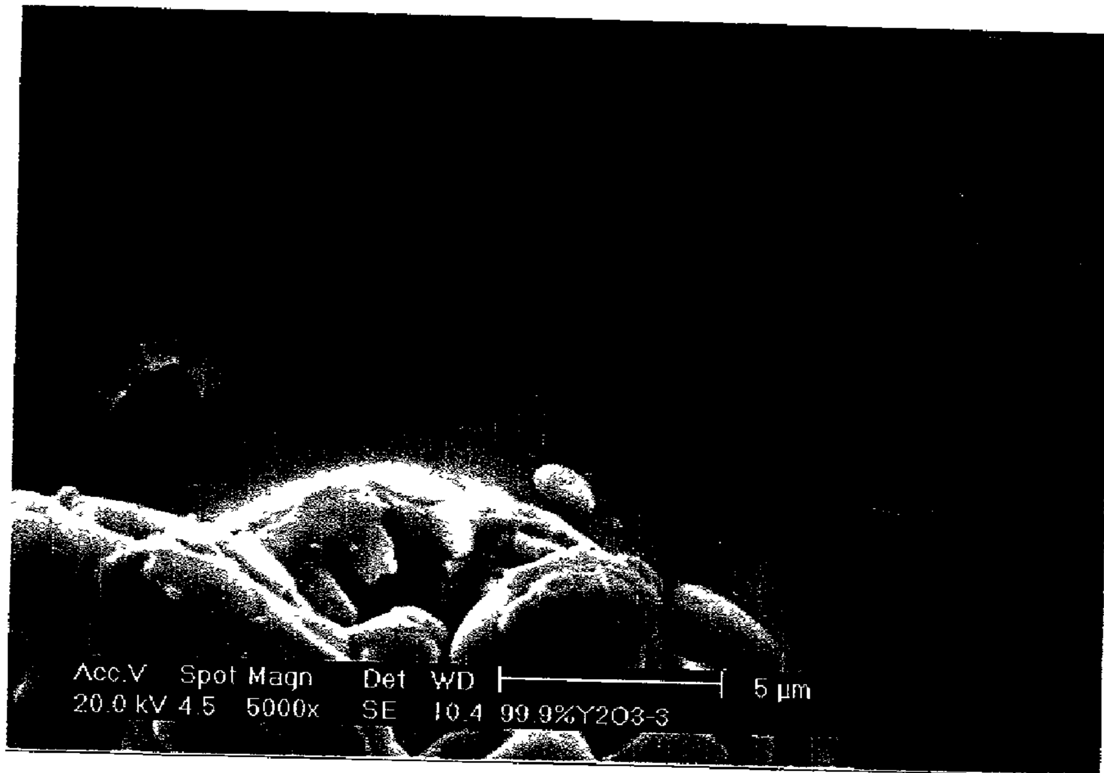
Surface of 99.9% Y 2 O 3 sprayed product (×5000)
