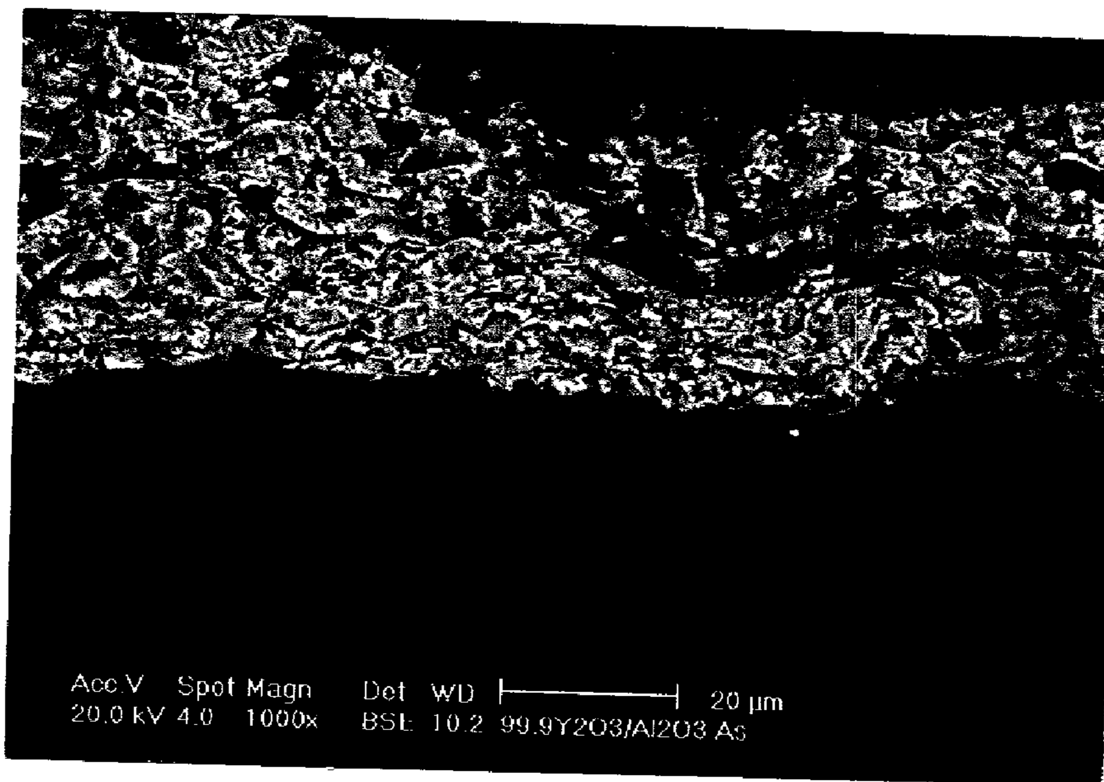
Section of 99.9% Y 2 O 3 sprayed product (×1000)
