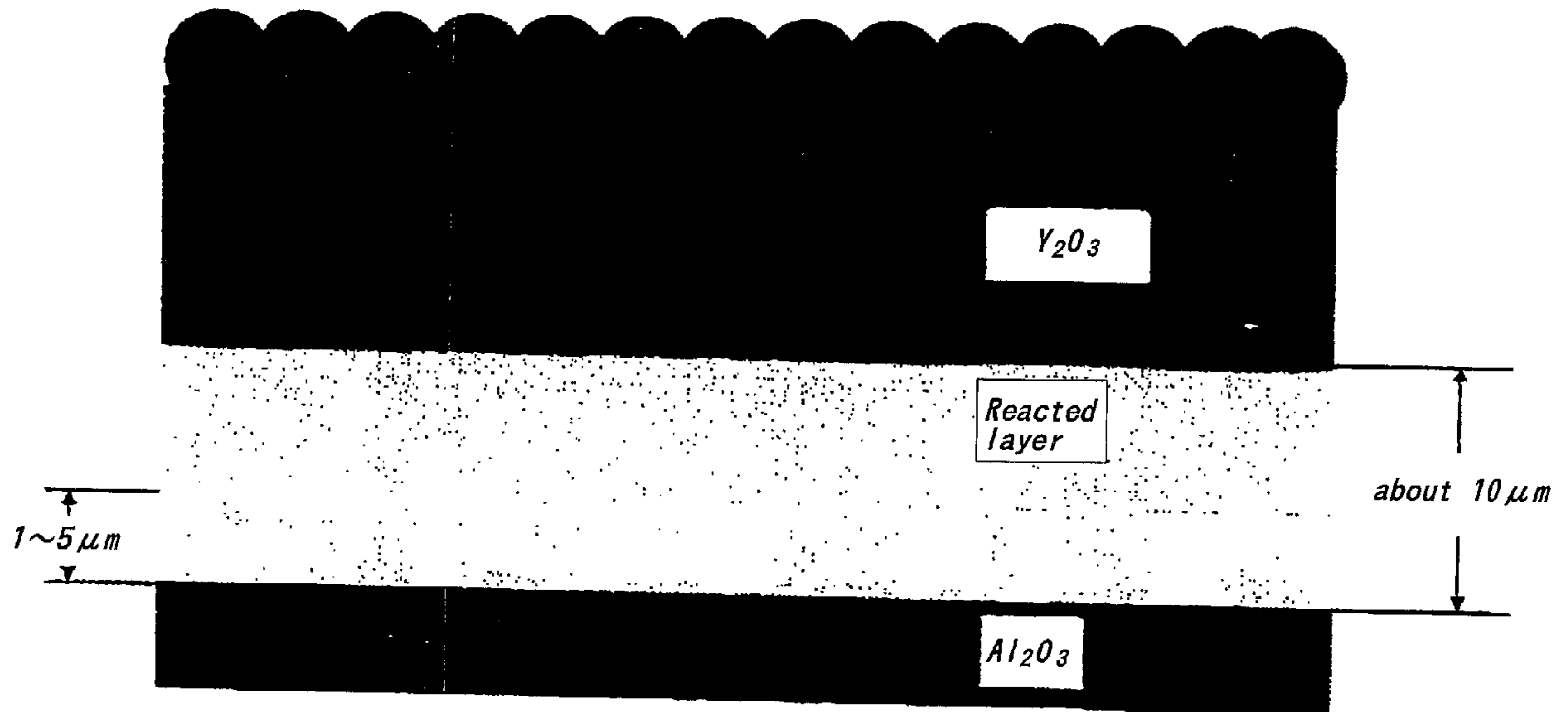
Structure of reacted layer (section)
