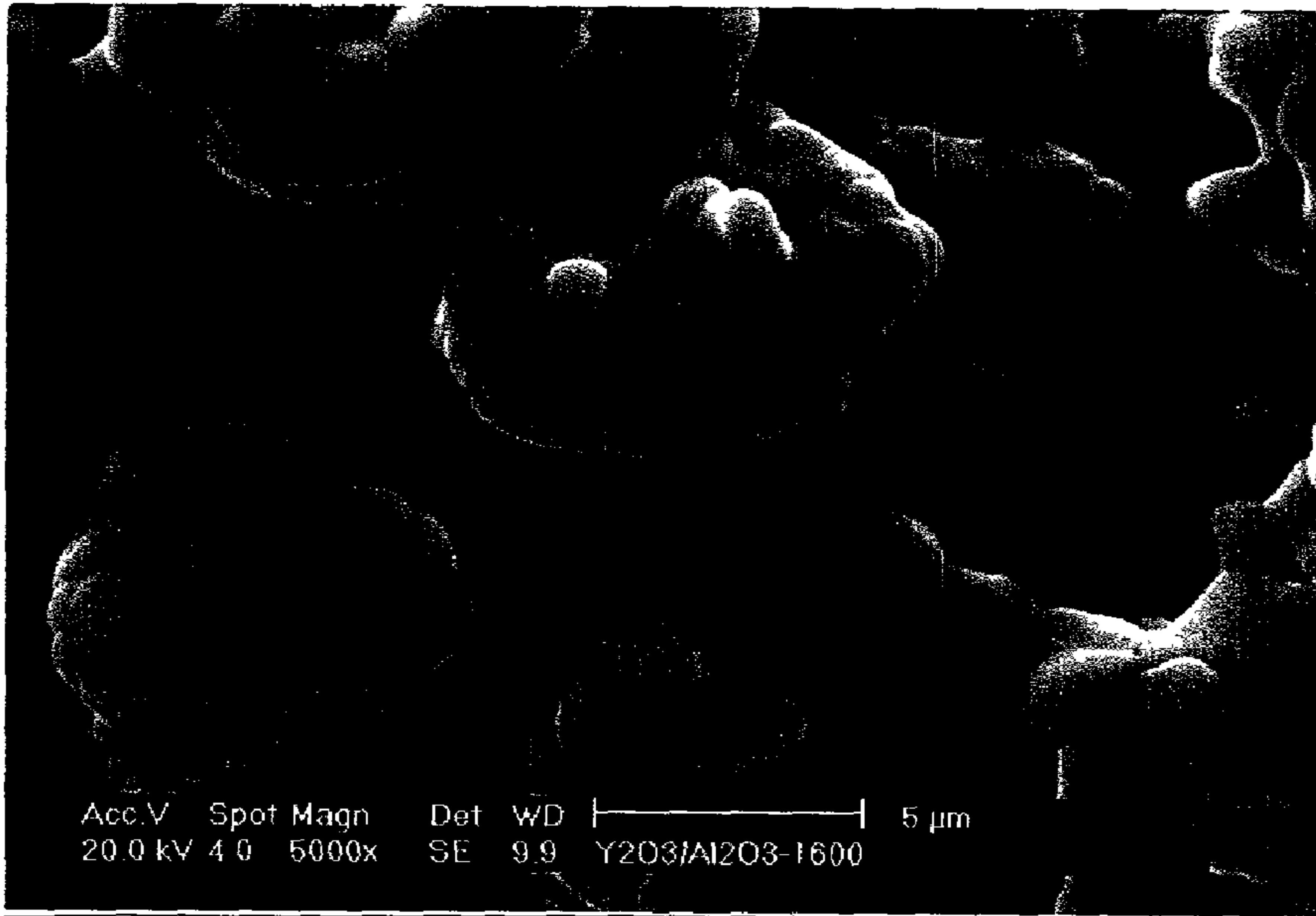
Surface of 1600°C × 3h Co-sintered product (×5000)
