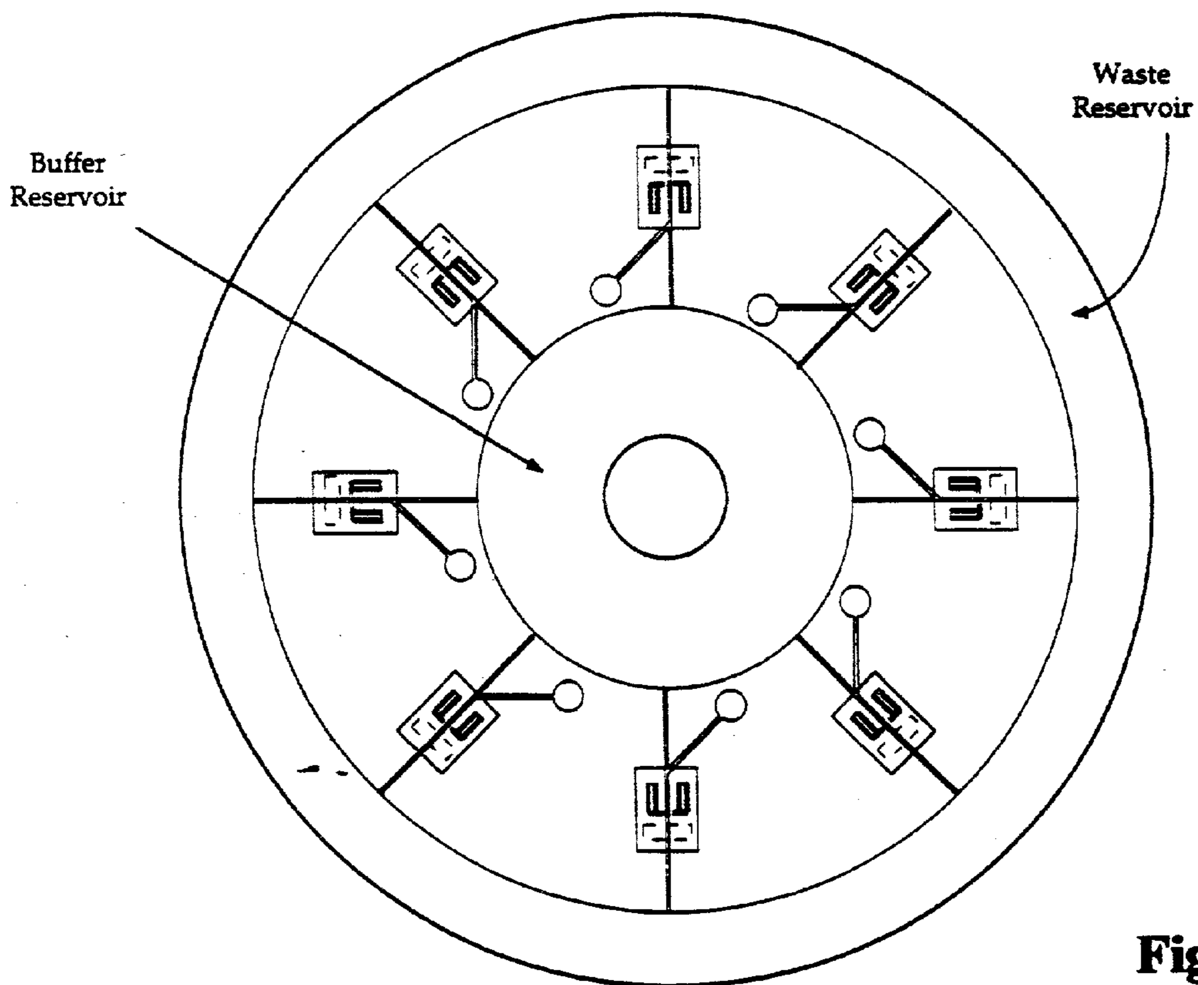
Eight Meltometers
