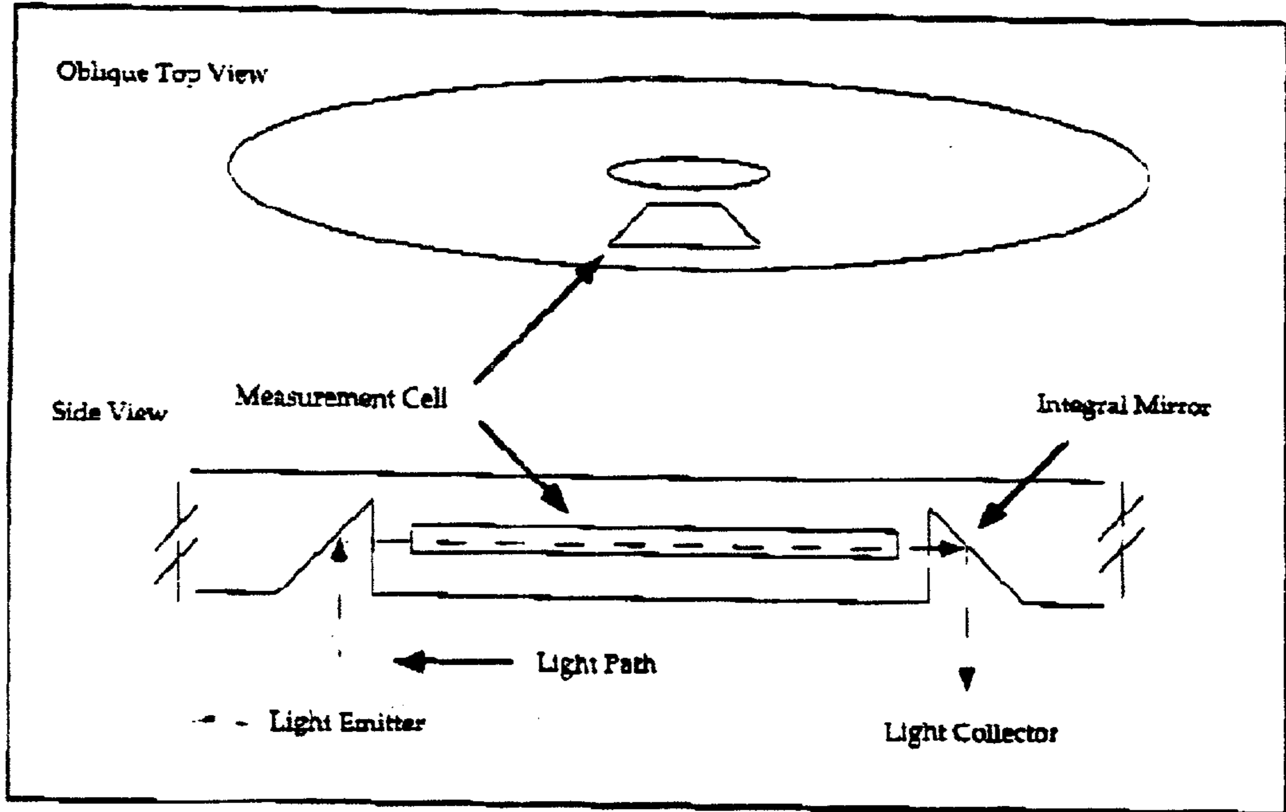
Schematic Representation of the Use of Integral Mirrors to Increase Optical Pathlength
