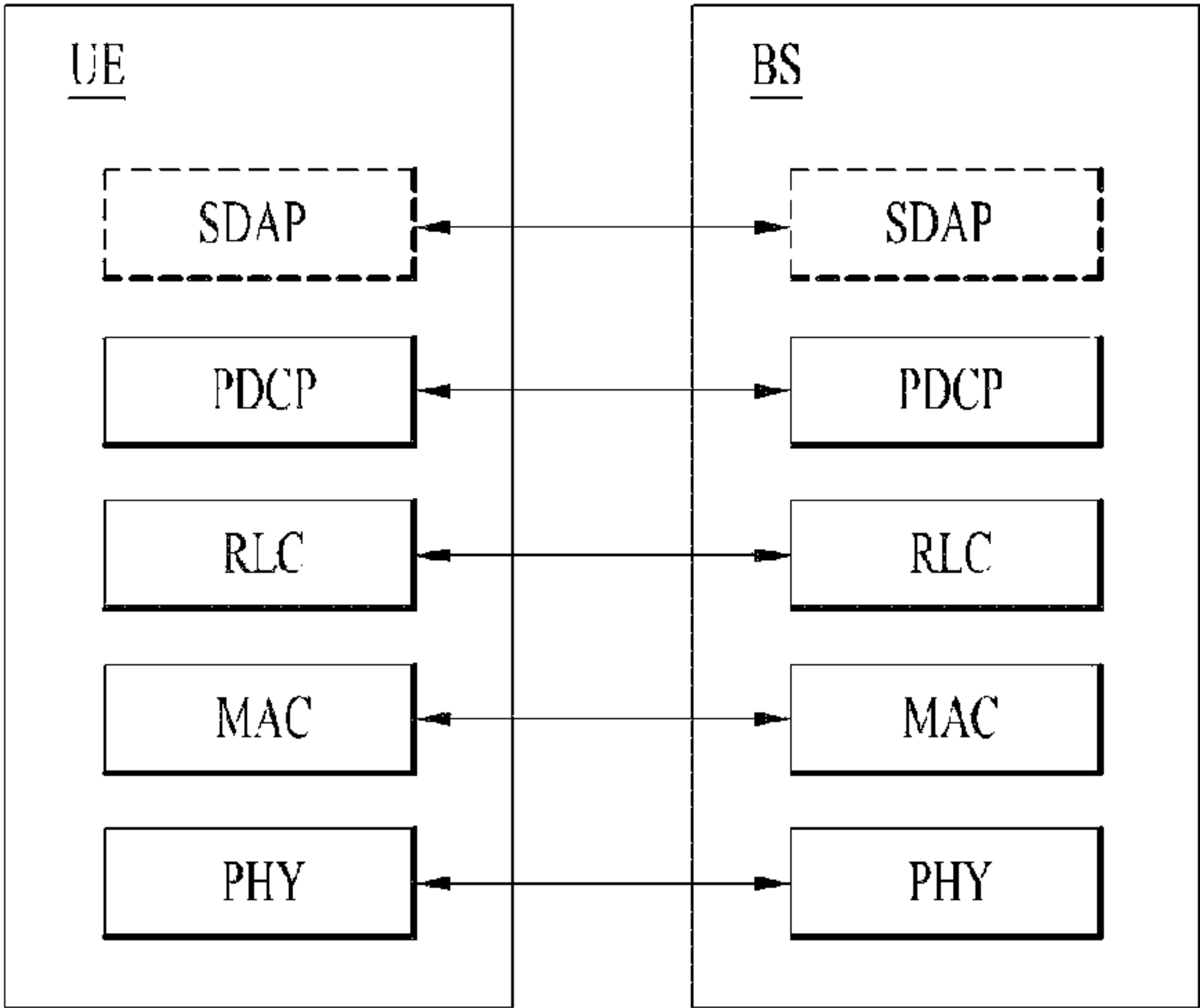
(a) User Plane Protocol Stack
