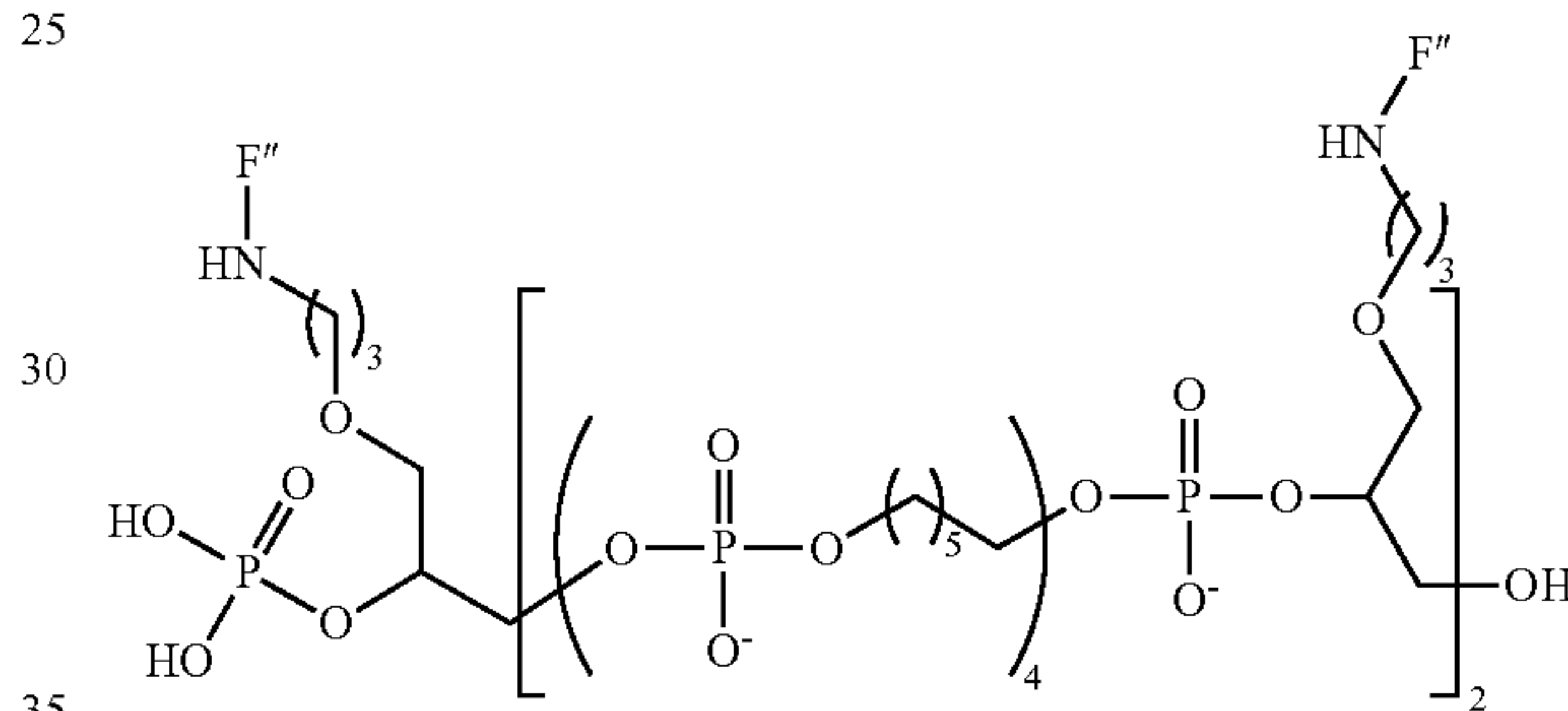
Compound F
