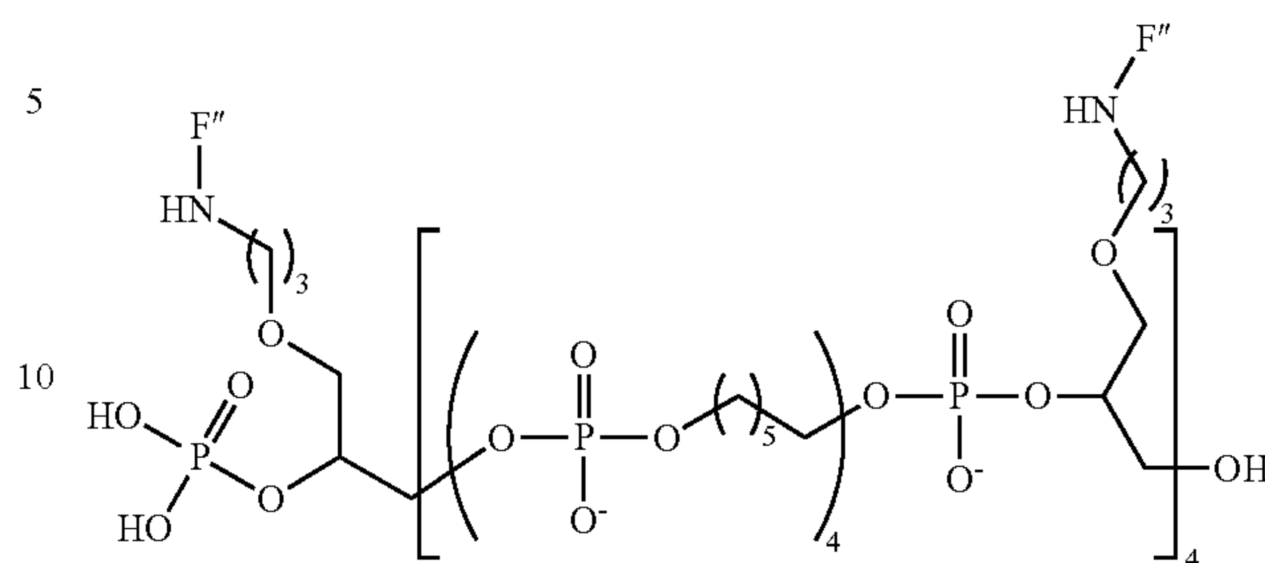
Compound E
