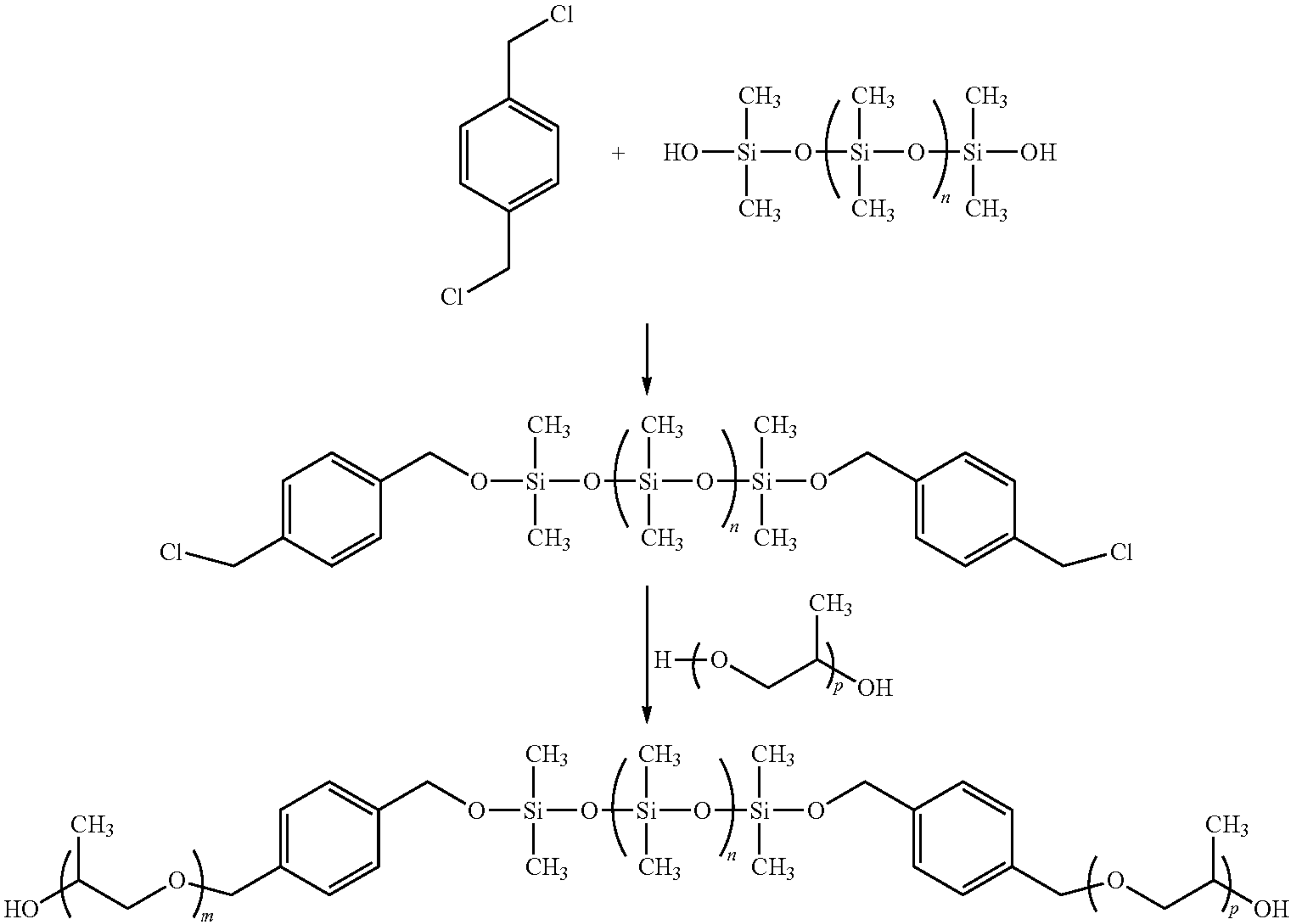
Synthesis of aromatic linked siloxane based triblock copolymer pre-soft-segment
