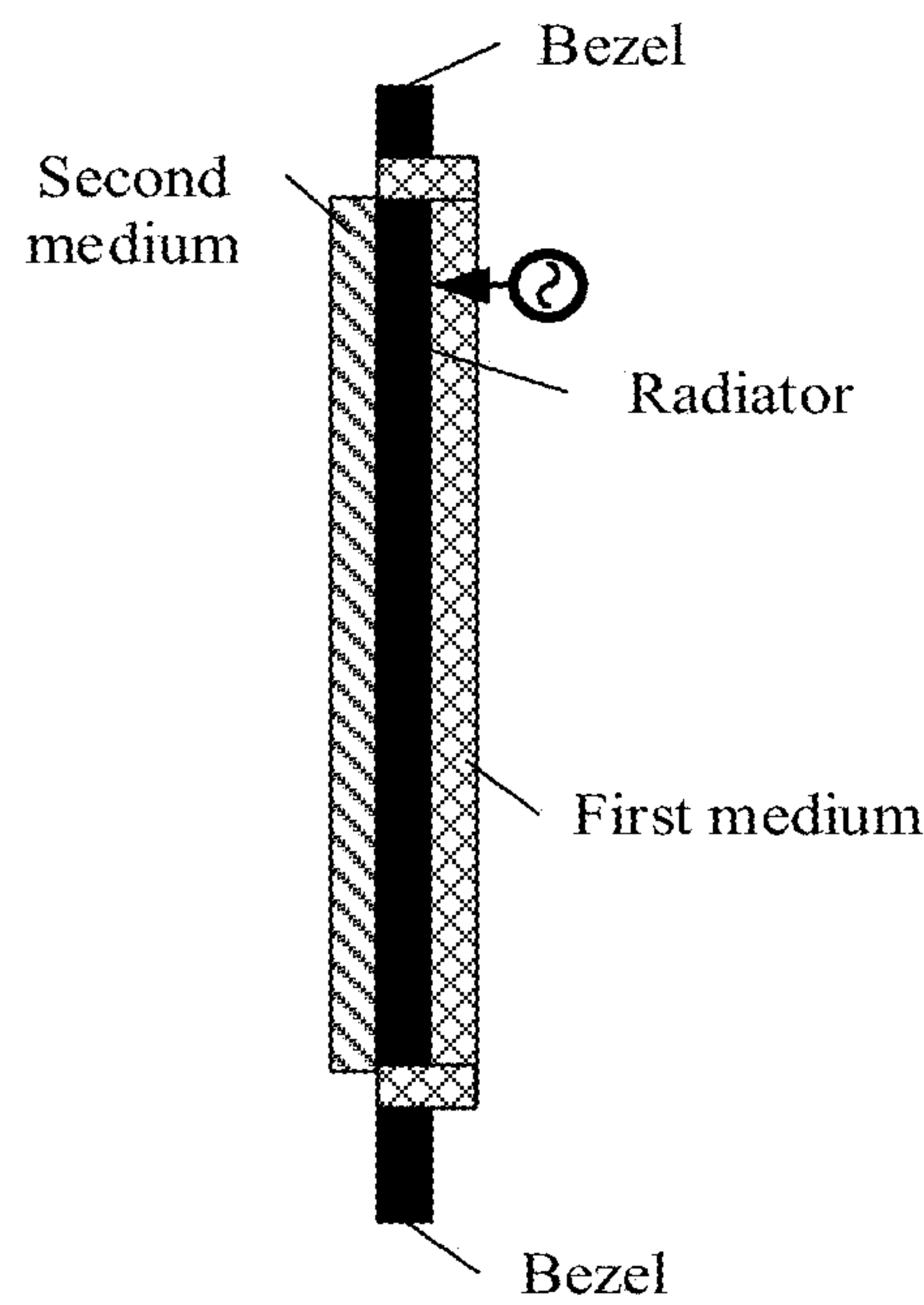
Full coverage of a radiator surface
