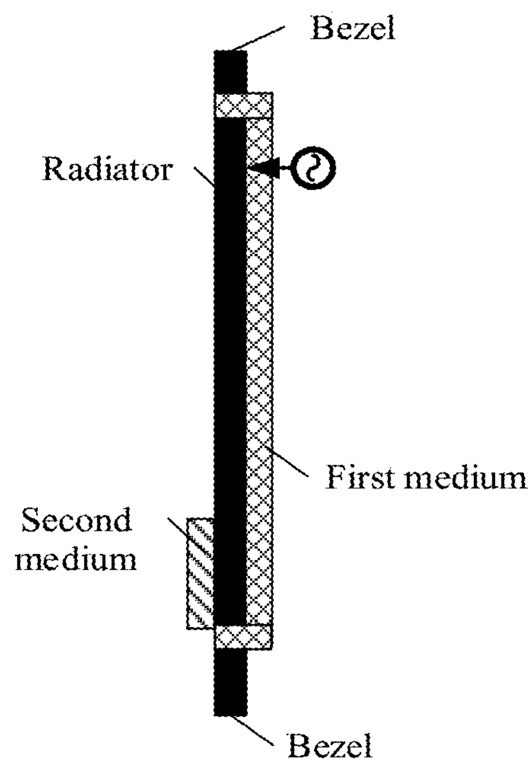
Partial coverage of a radiator surface
