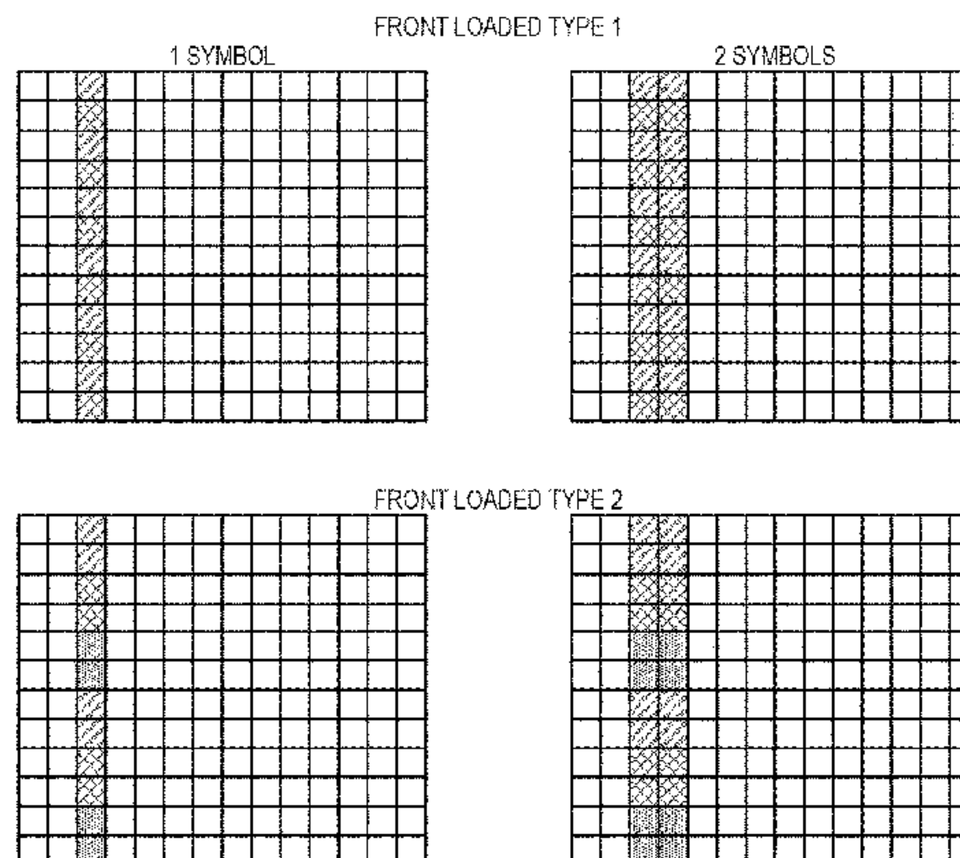
Front-loaded DM-RS for configuration type 1 and type 2. Different CDM groups indicated by different patterns. The figures to the left show a single front-loaded DMRS while to the right shows double DMRS. To enable the DMRS pattern to the right max_length=2 must be enabled by higher layer signaling
