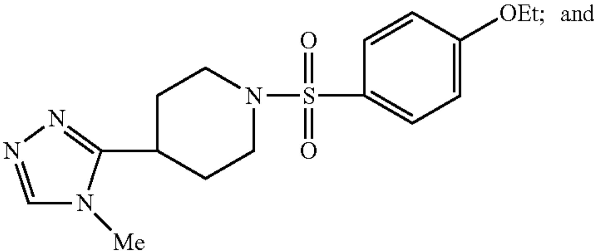
(compound W)
