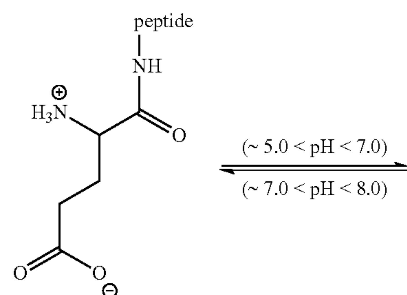
Scheme 3: N-terminal cyclization of uncharged glutamyl peptides by QC (EC)
