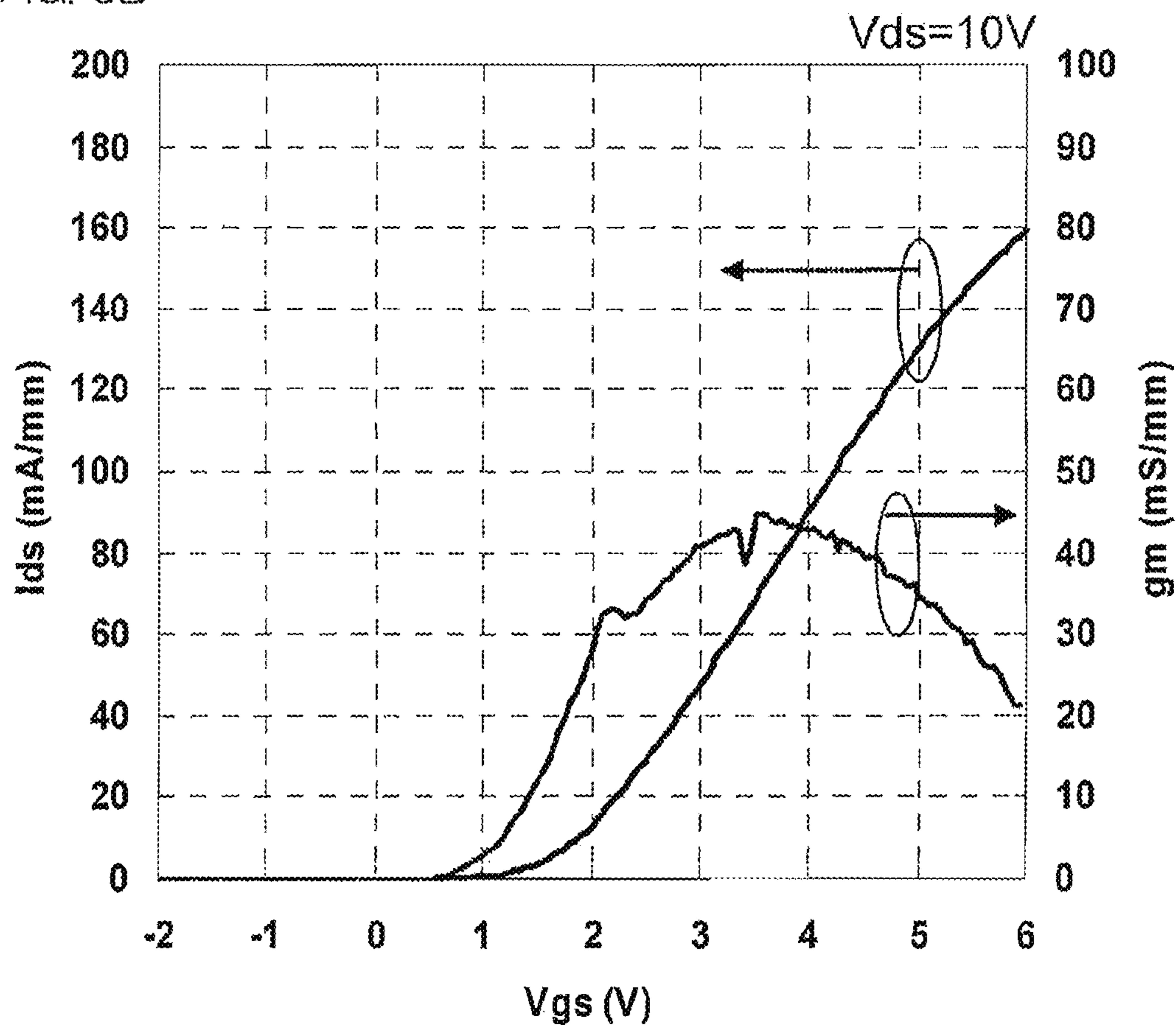
Transfer characteristics.
