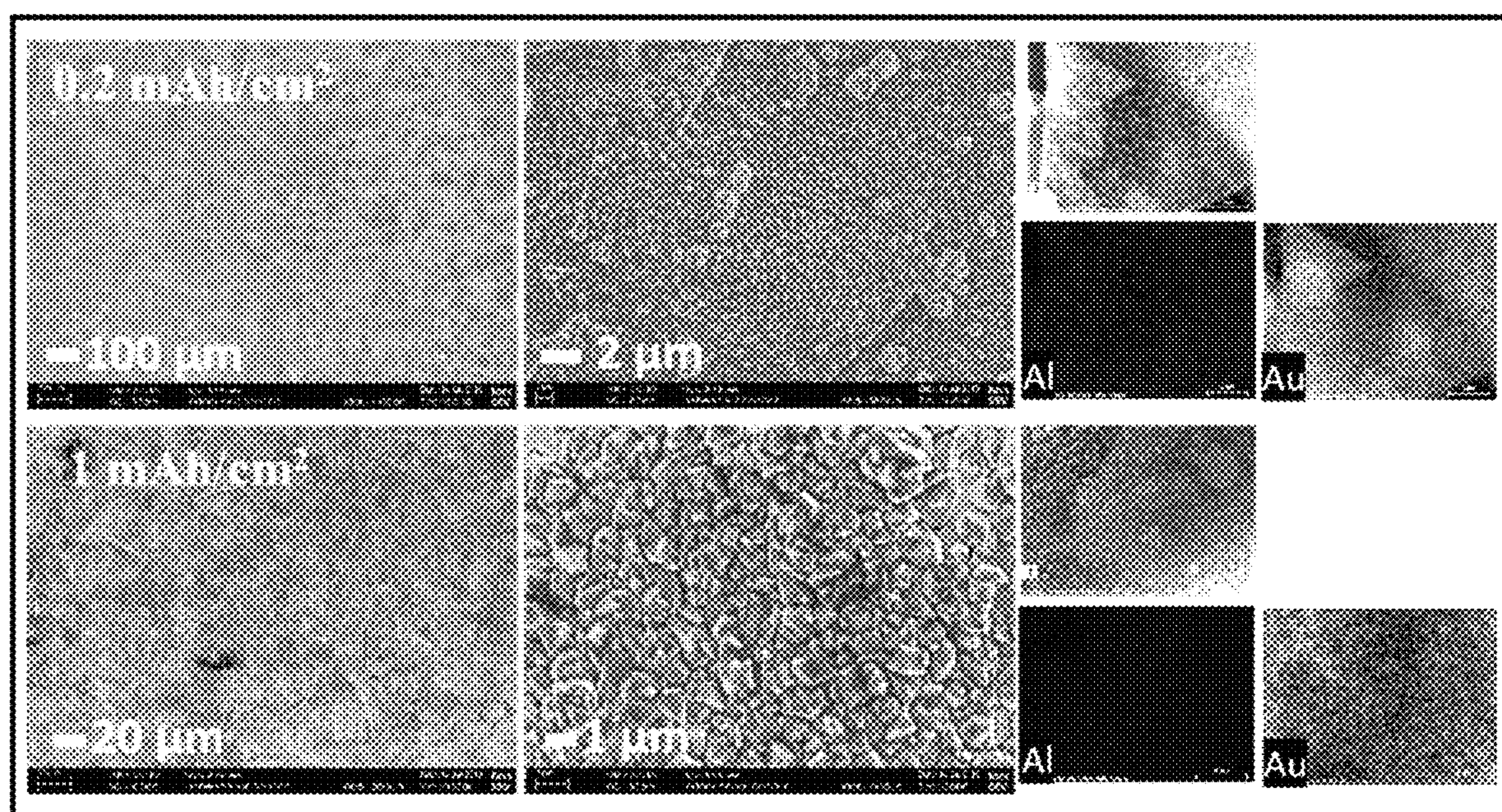
Al deposits on (111)-Au coated stainless steel
