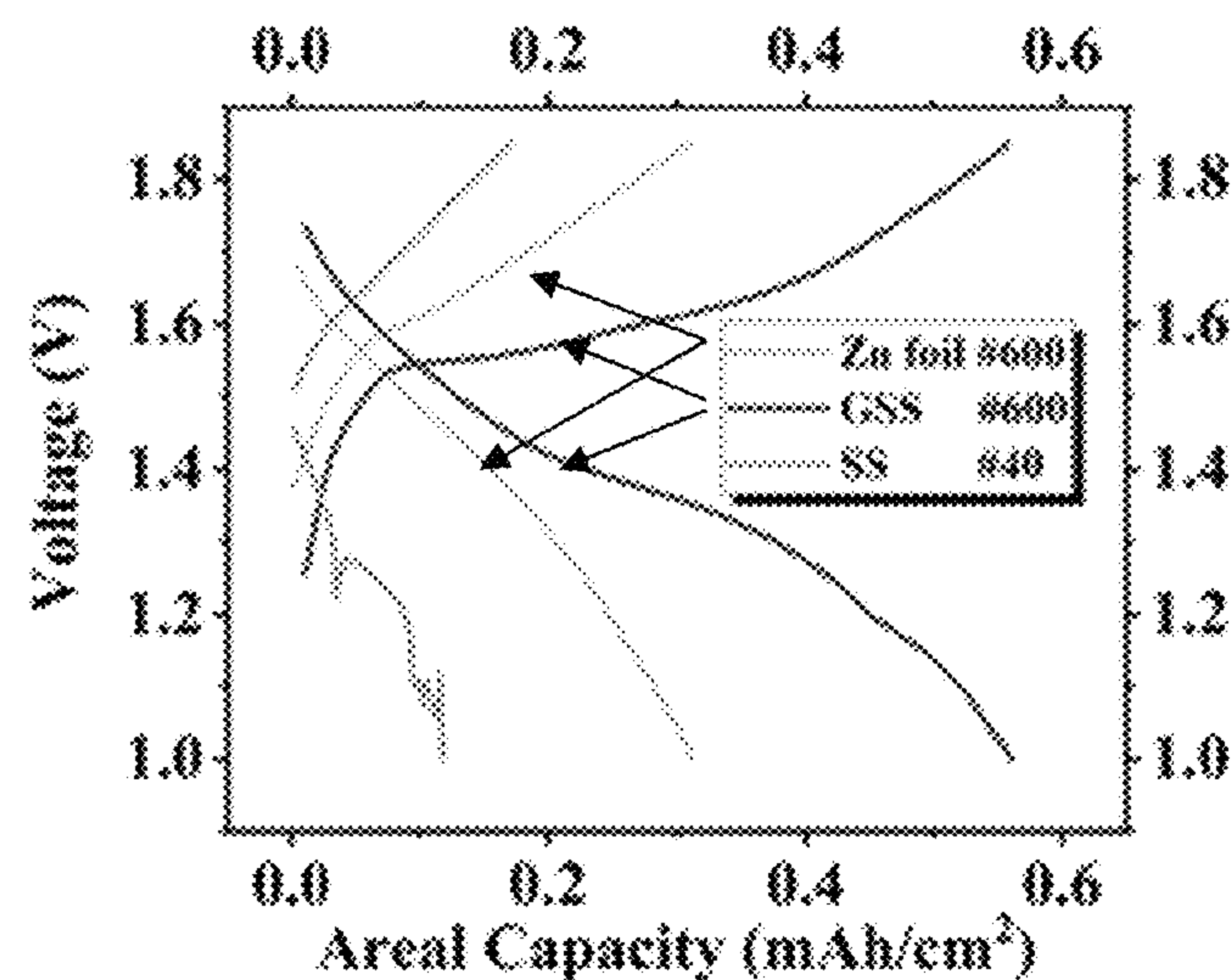
Voltage profile
