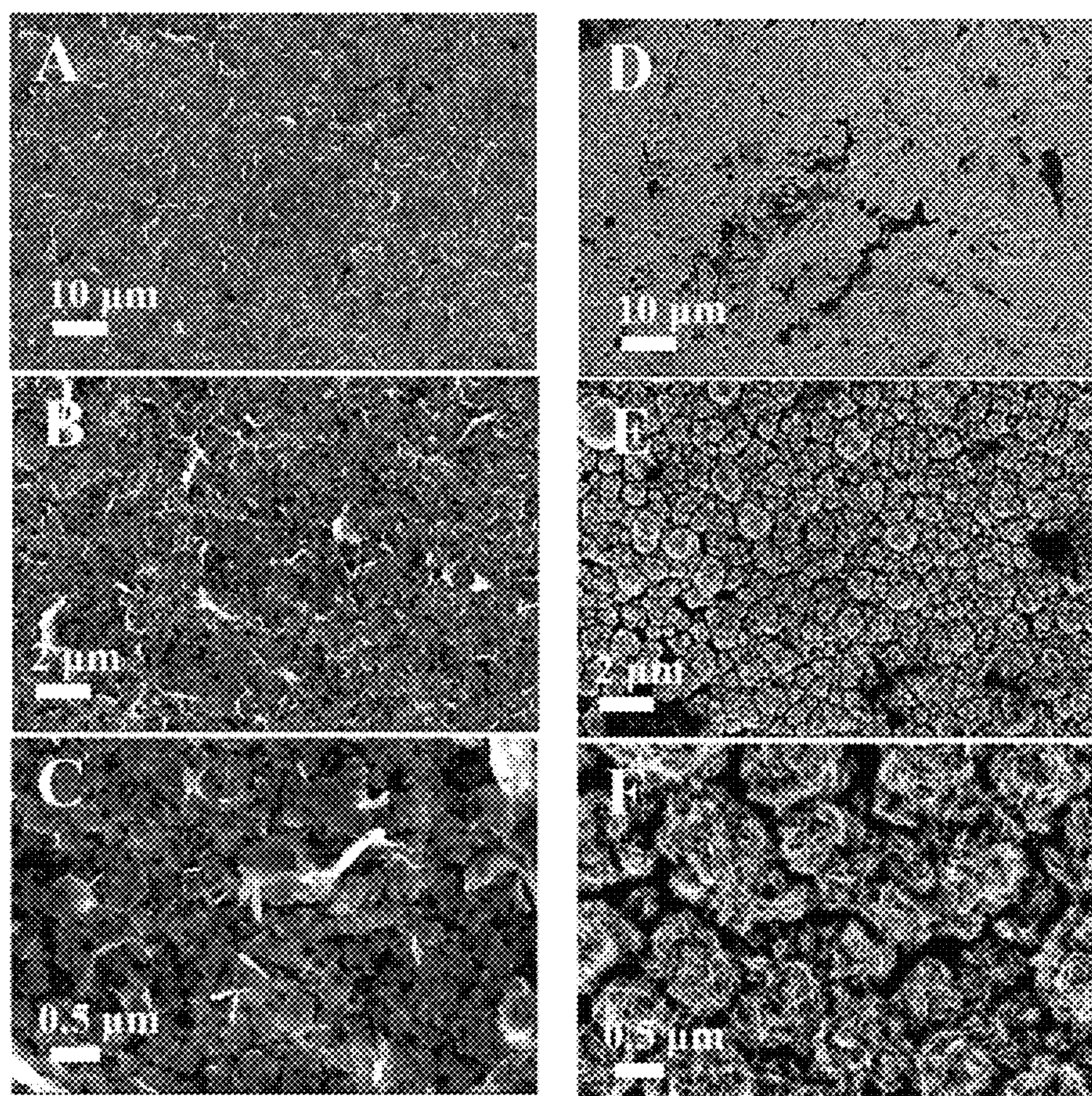
SEM of Zn in \text{Zn}(\text{CF}_3\text{SO}_3)_2/\text{DME} . Left: G-SS; Right: SS.
