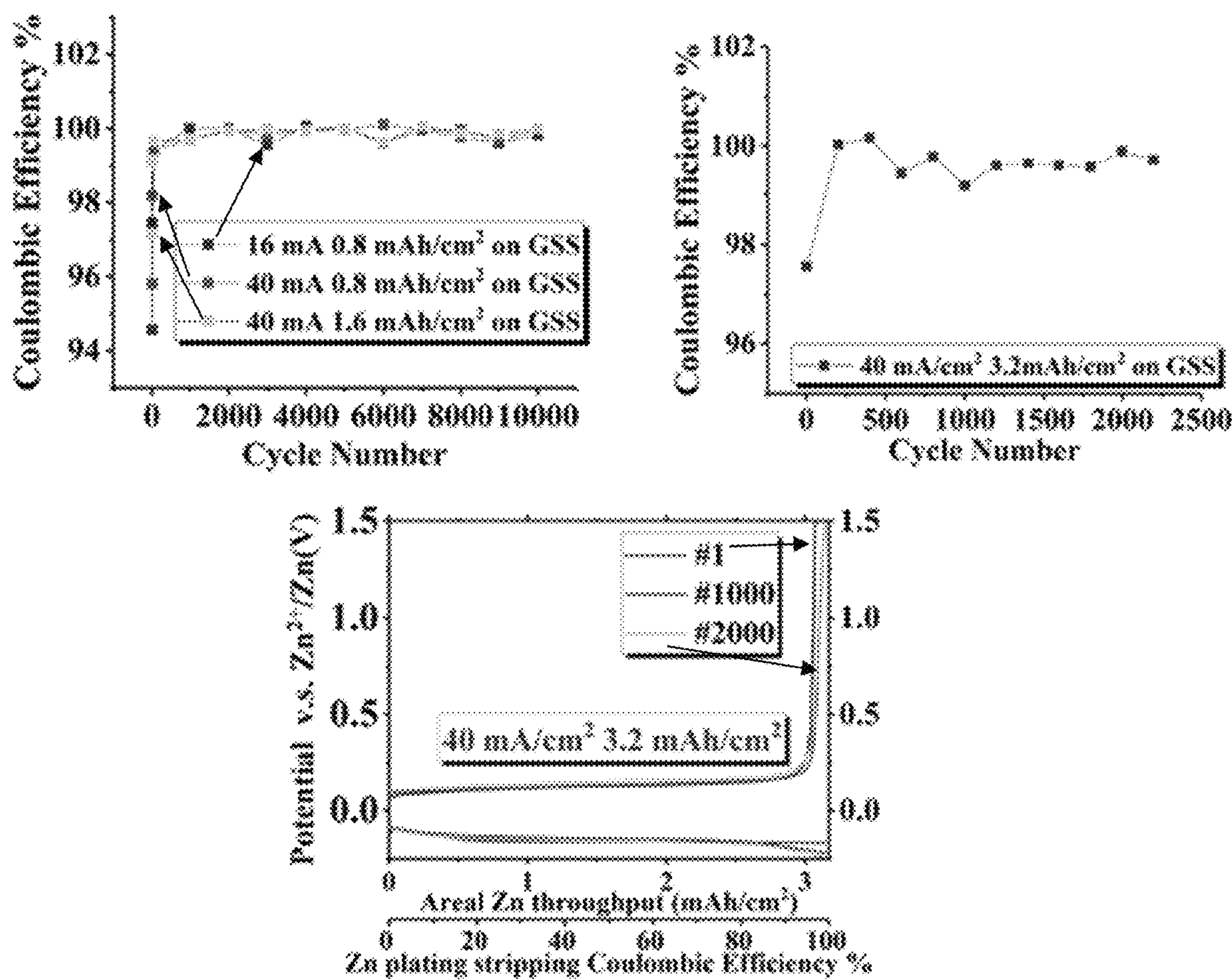
Zn CE on aligned graphene
