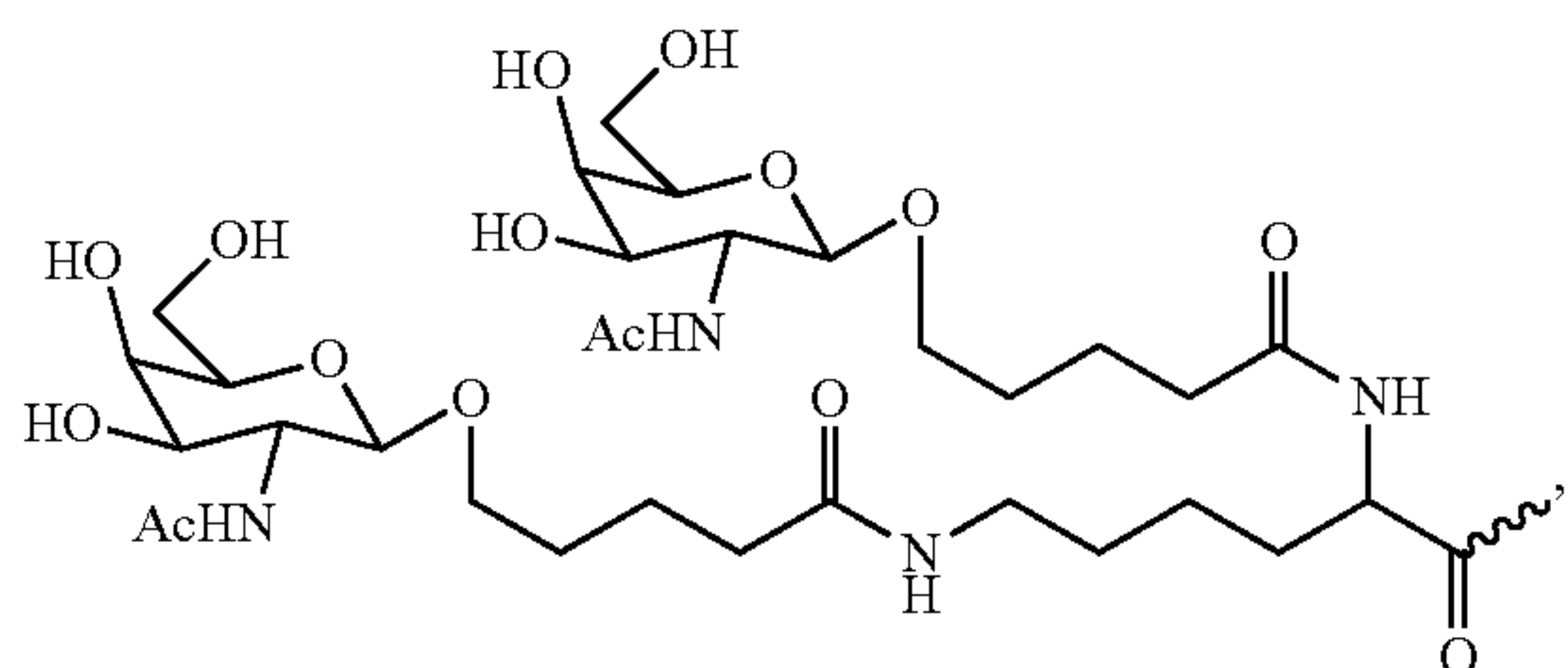
Formula XVIII
