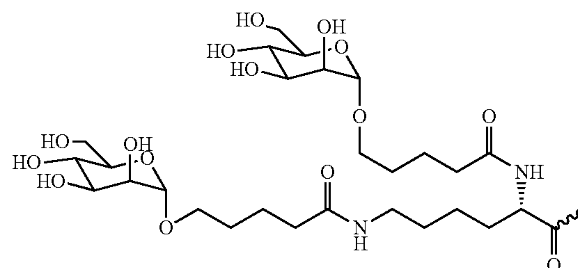
Formula XXI
