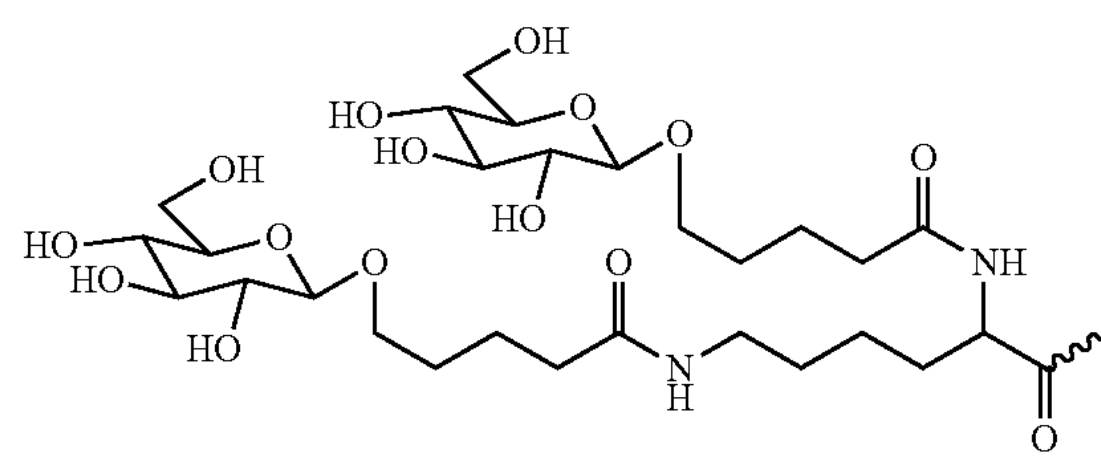
Formula XIX
