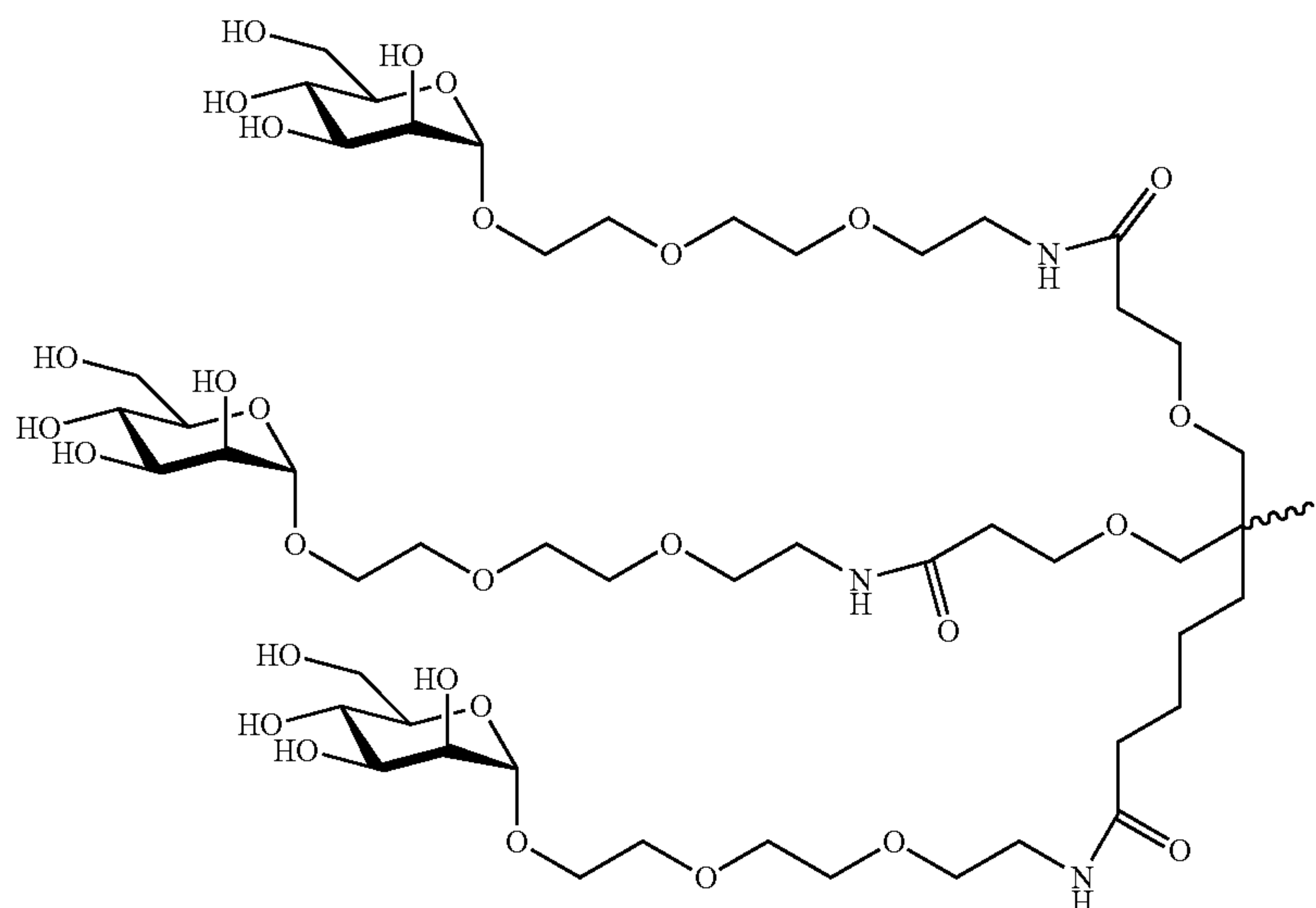
Formula IV
