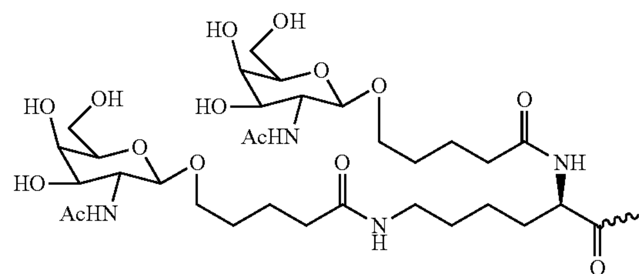
Formula XVII
