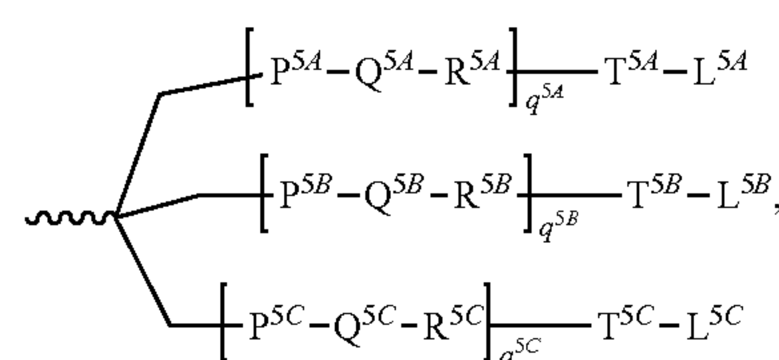
Formula XXXIII
