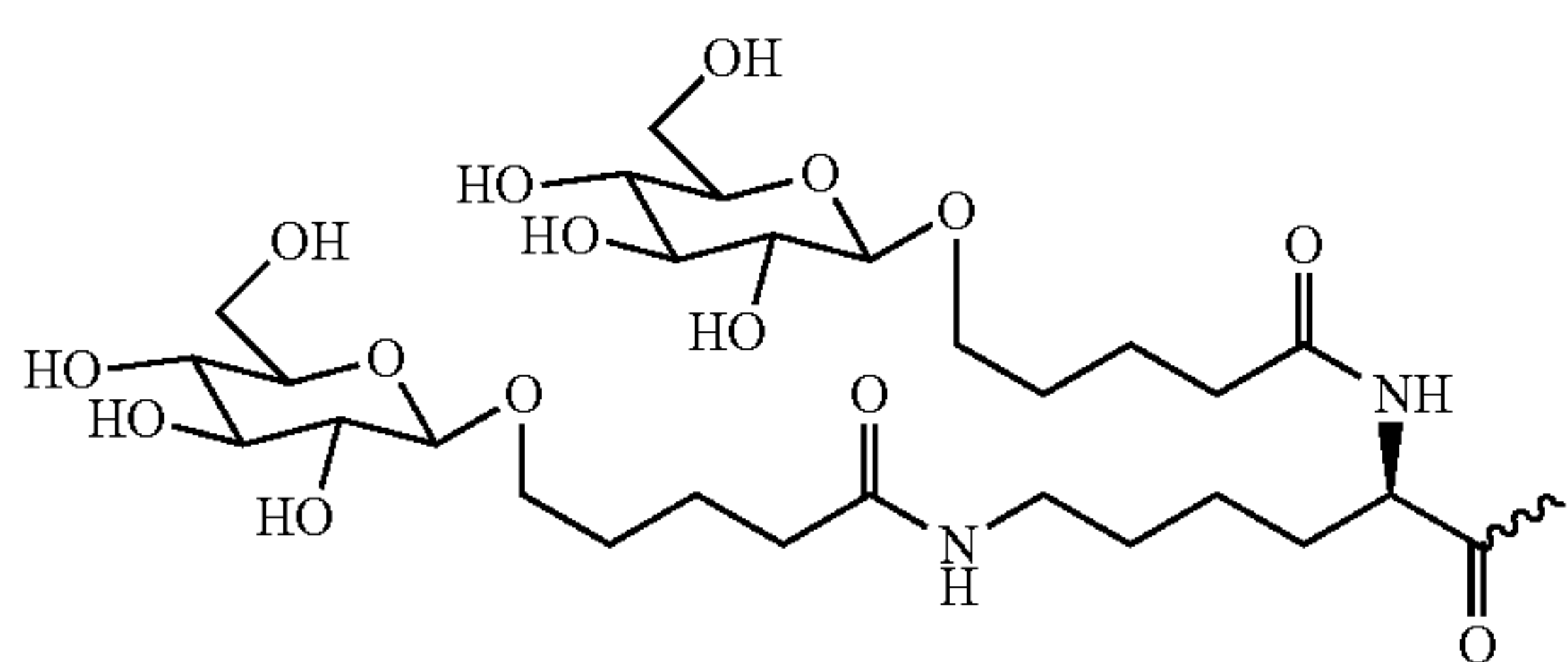
Formula XVIII
