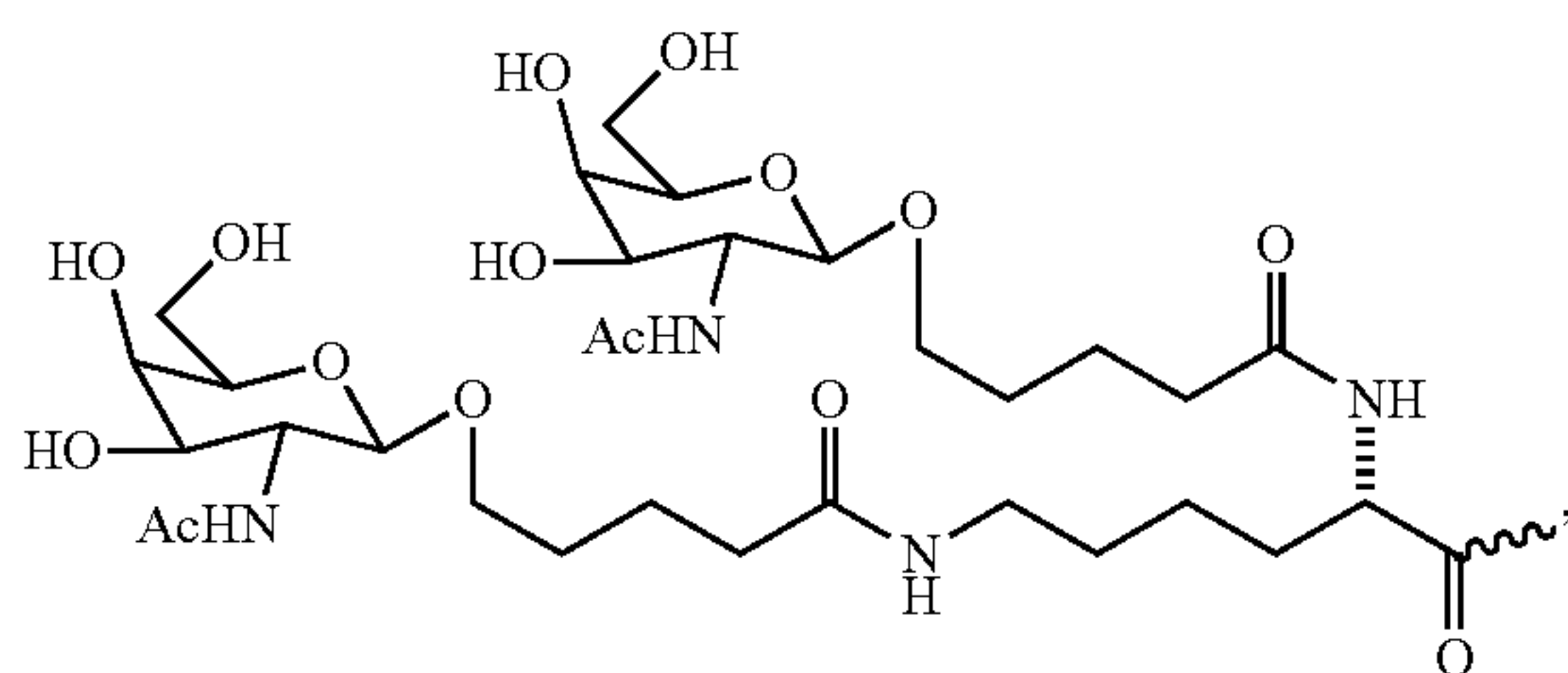
Formula XVI
