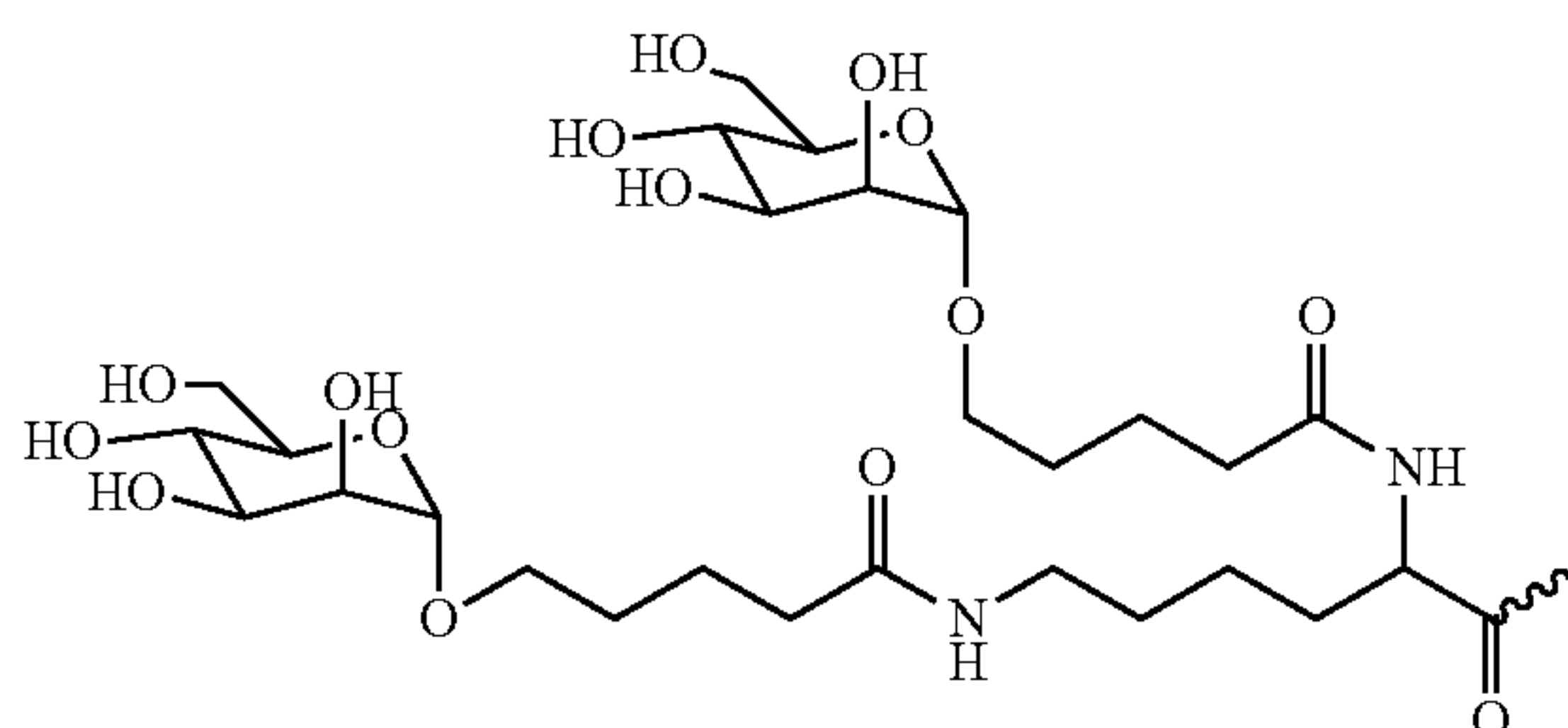
Formula XX
