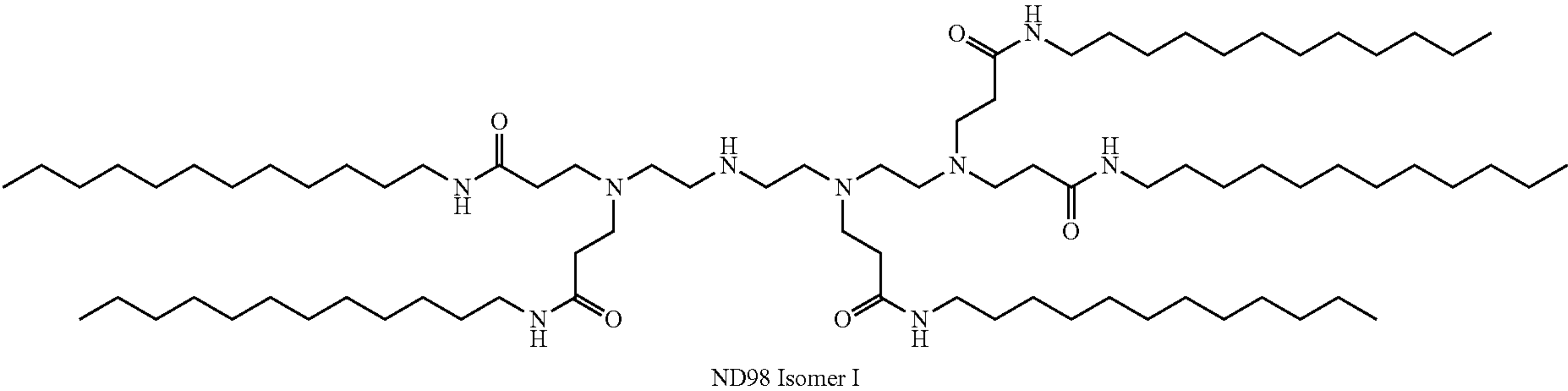
Formula 1
