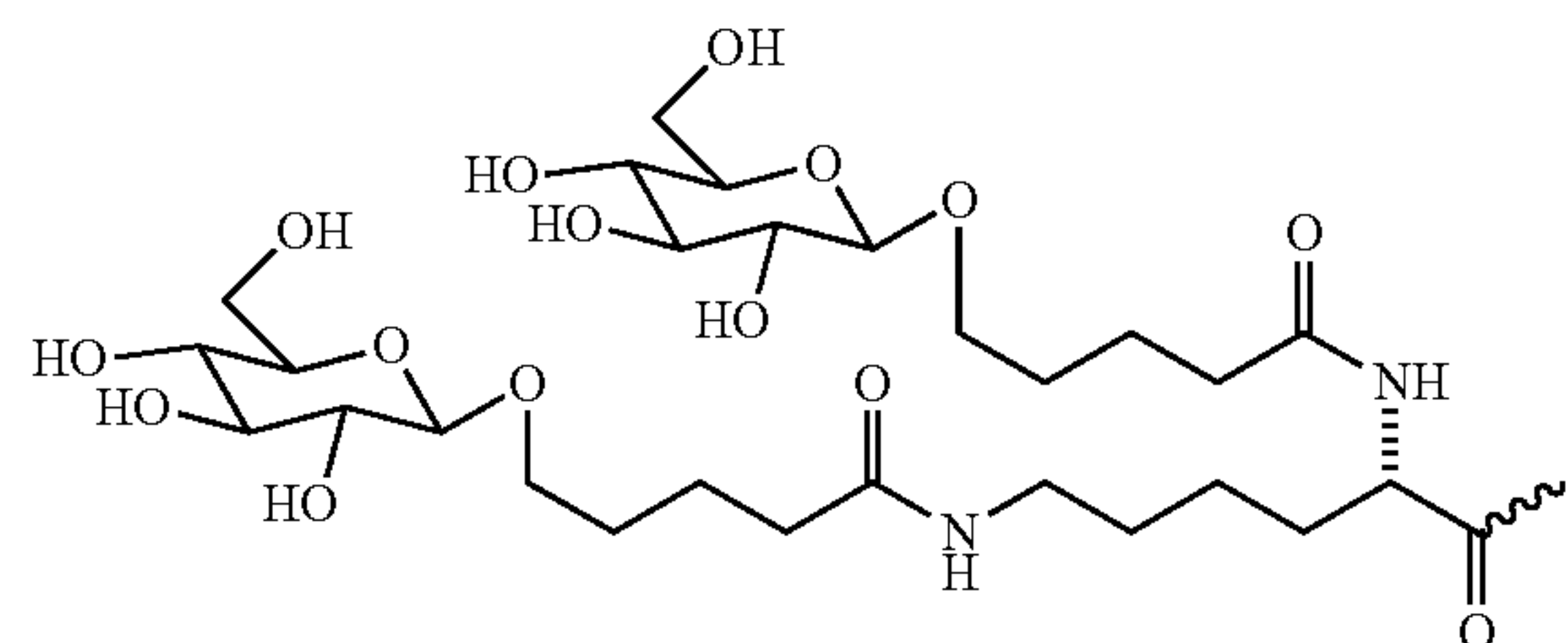
Formula XIX
