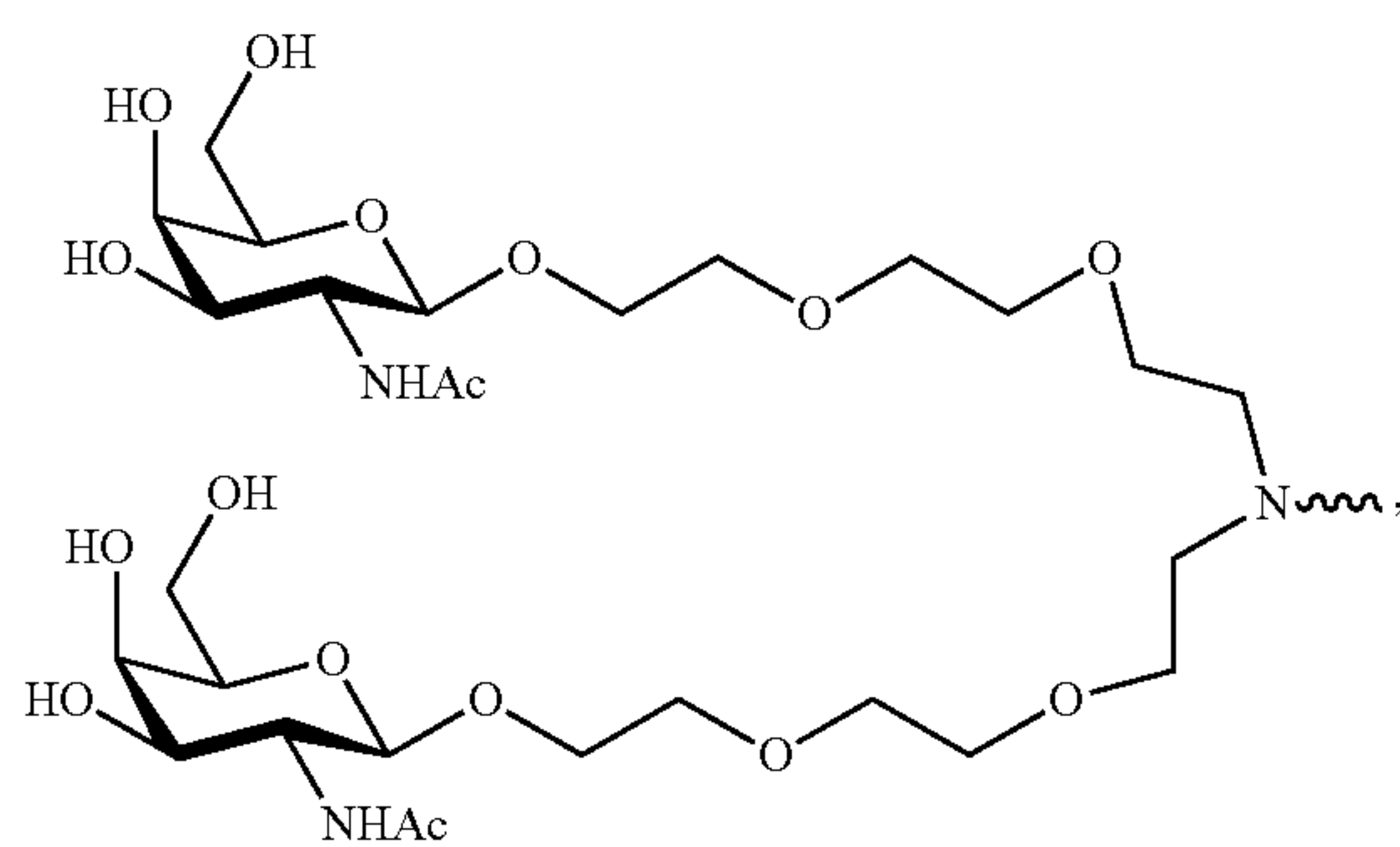
Formula IV
