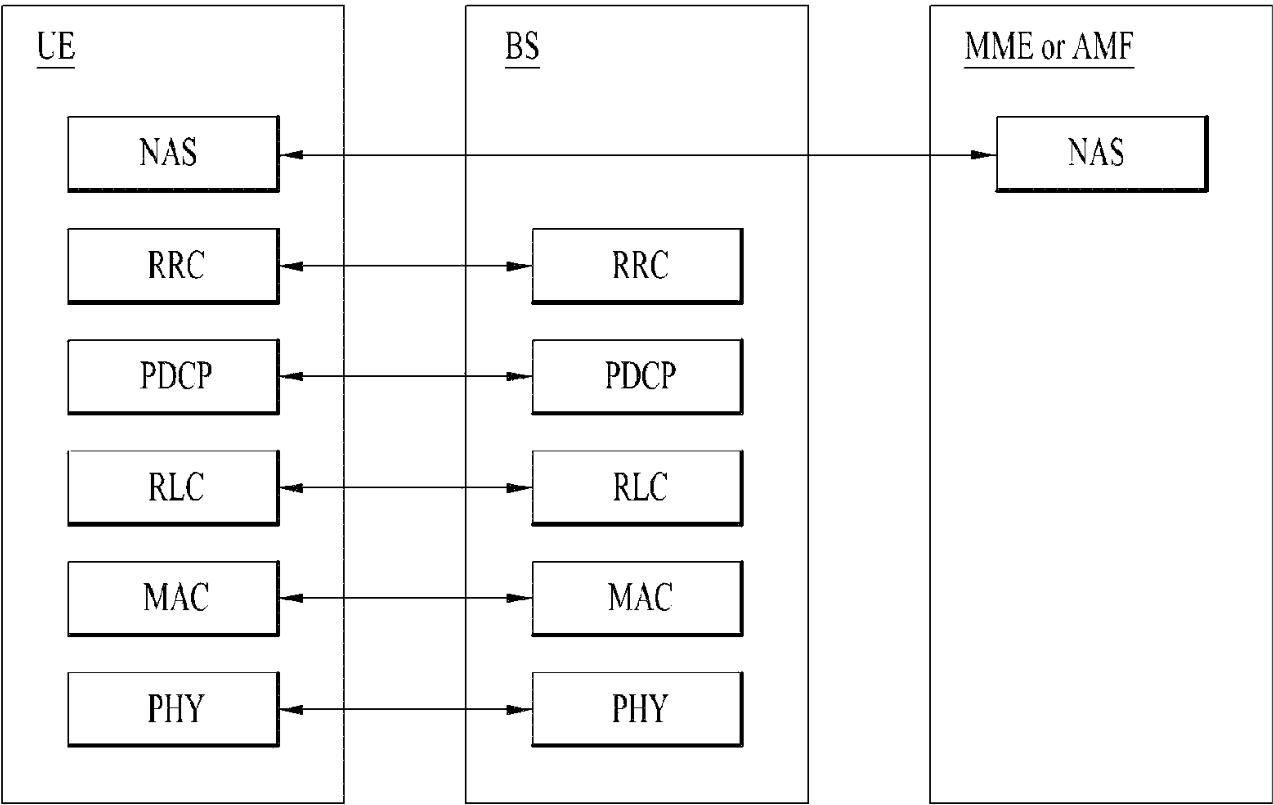
(b) Control Plane Protocol Stack
