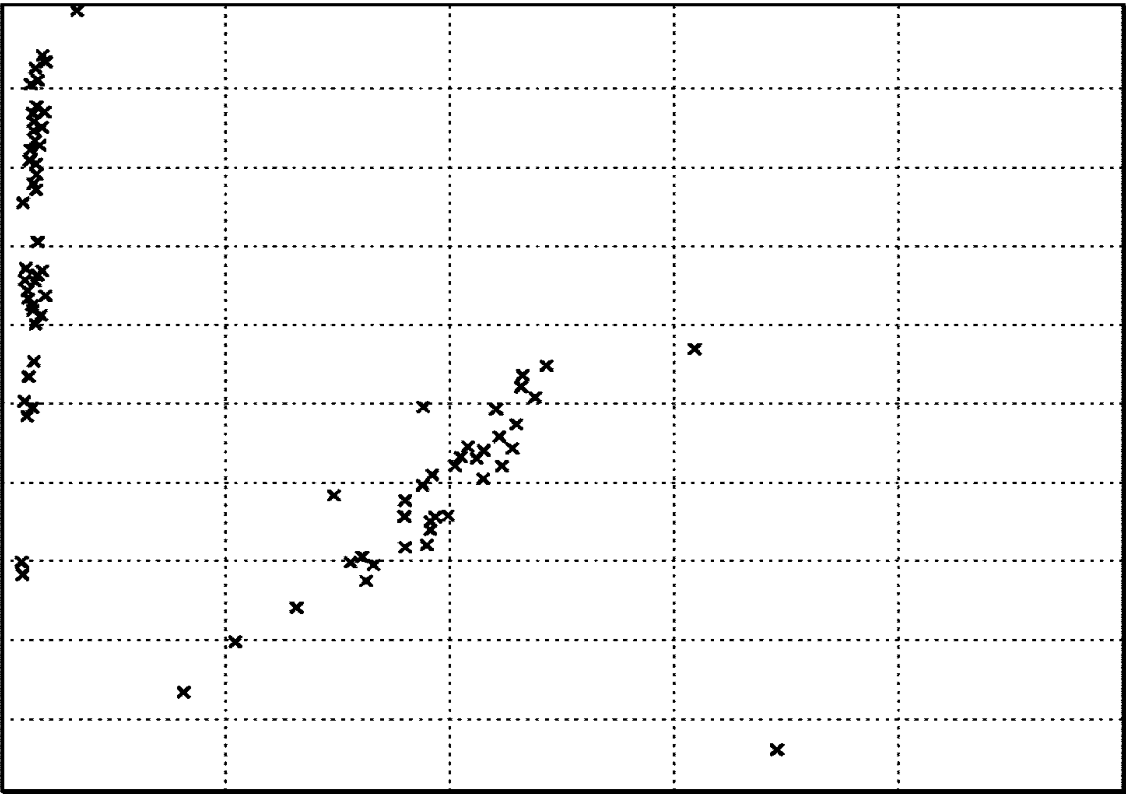
FIG. 18B Eureka Assay on PCR amplicons that isolate the target ("enrich selected genome")
