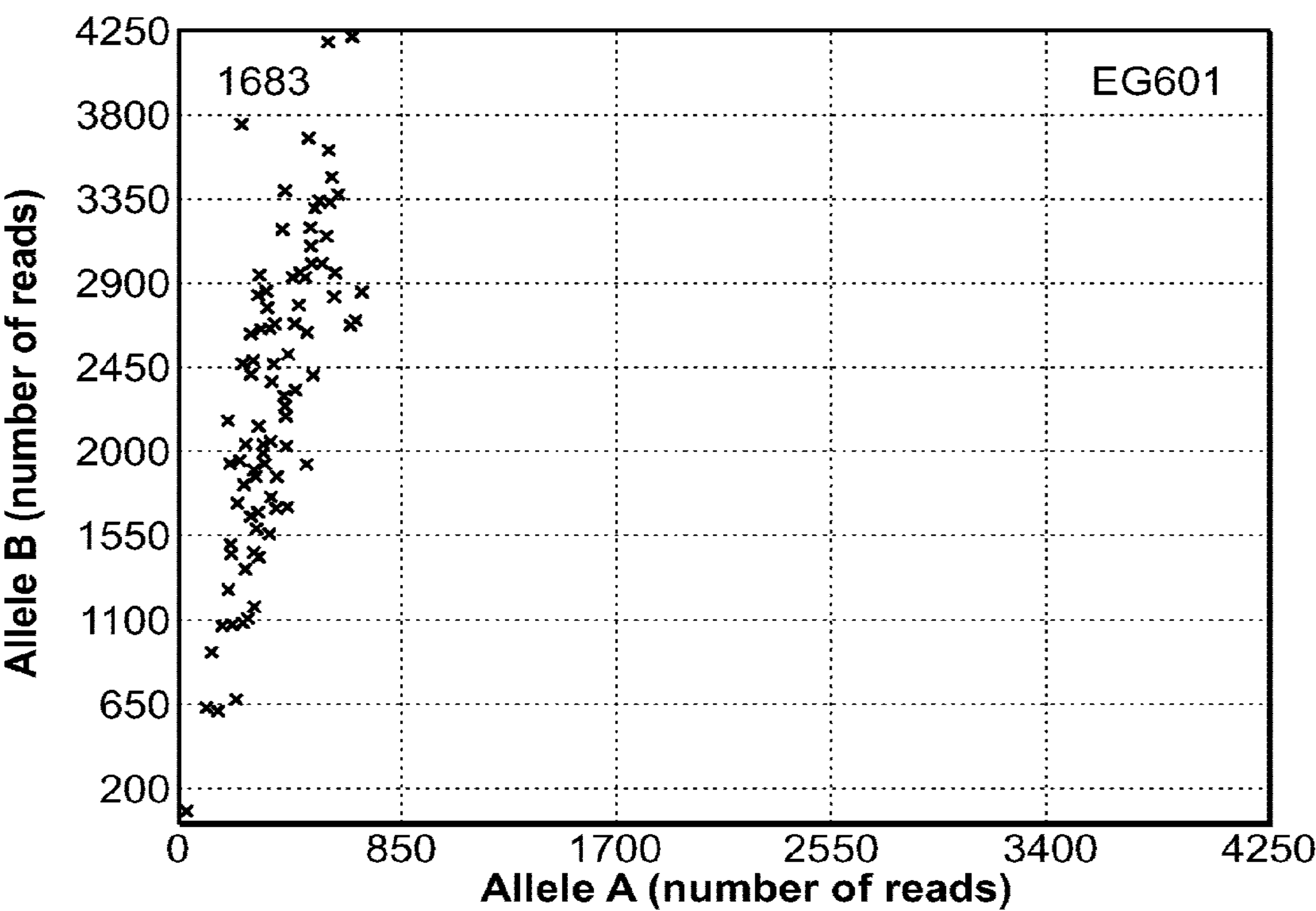
FIG. 18A Eureka Assay on genomic DNA
