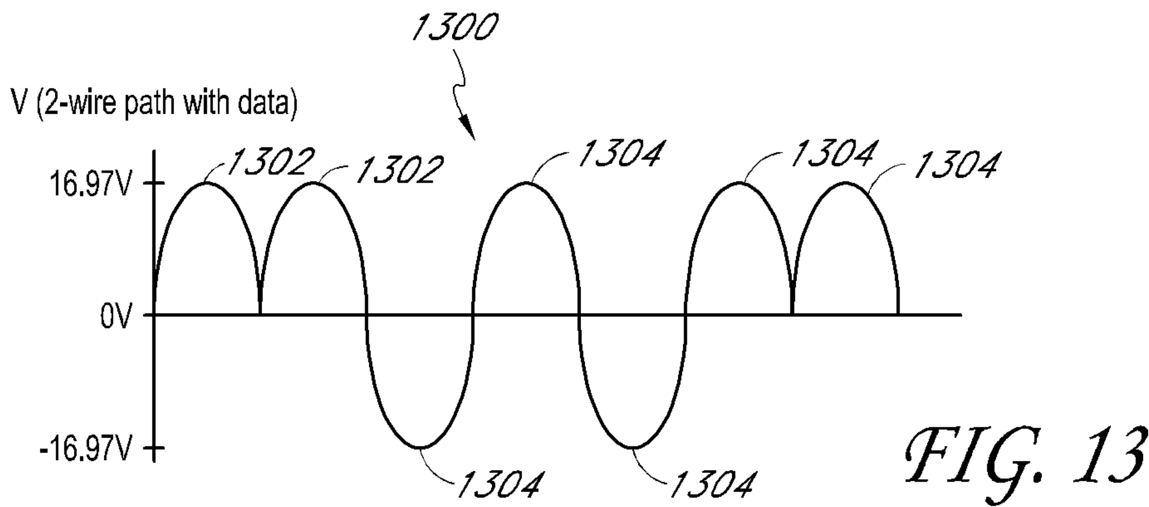
Bridge Waveforms
