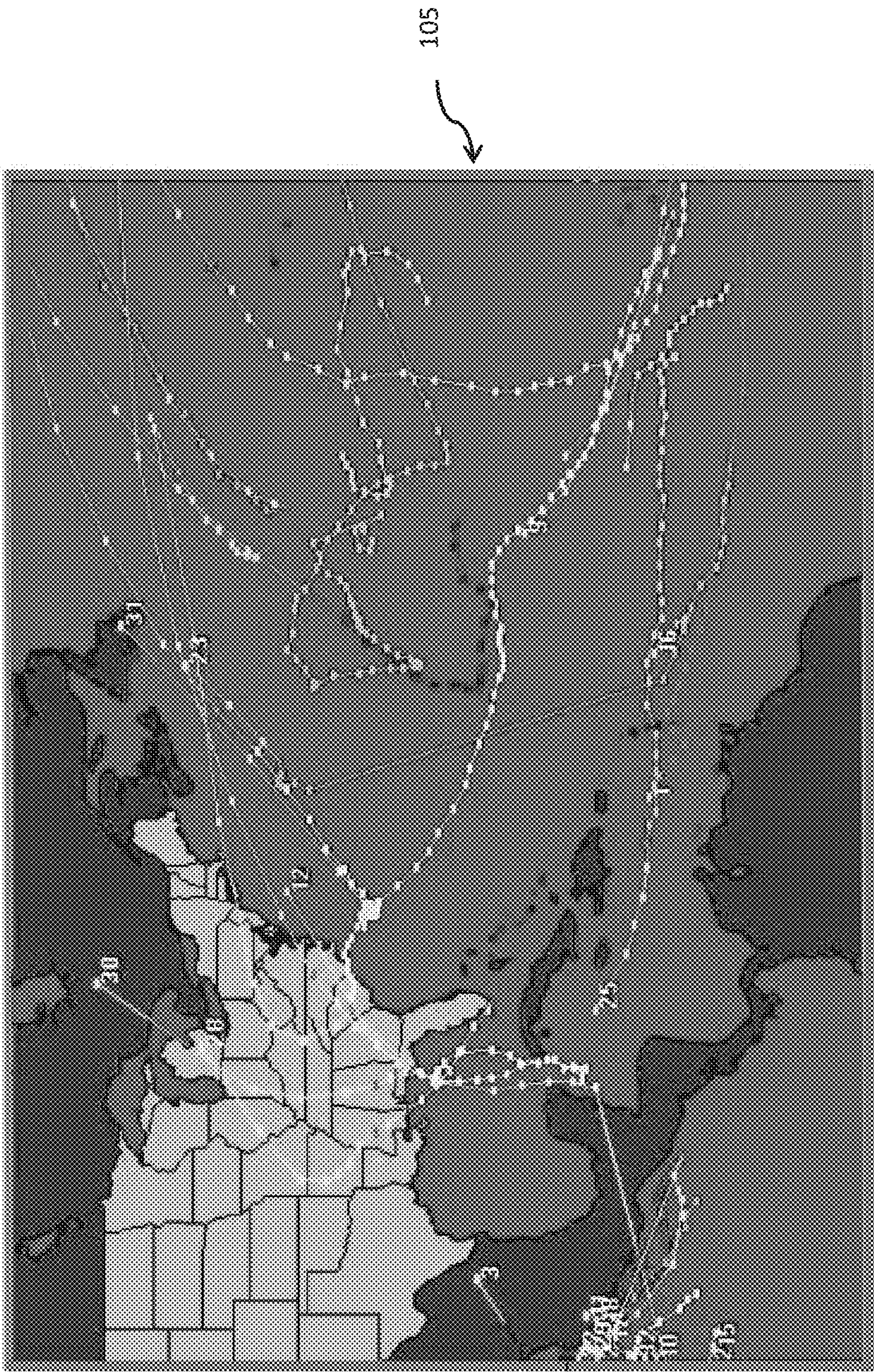
Data Input Examples FIGURE 8 Historical Analog Input (e.g. Hurricane Data from prior years)
