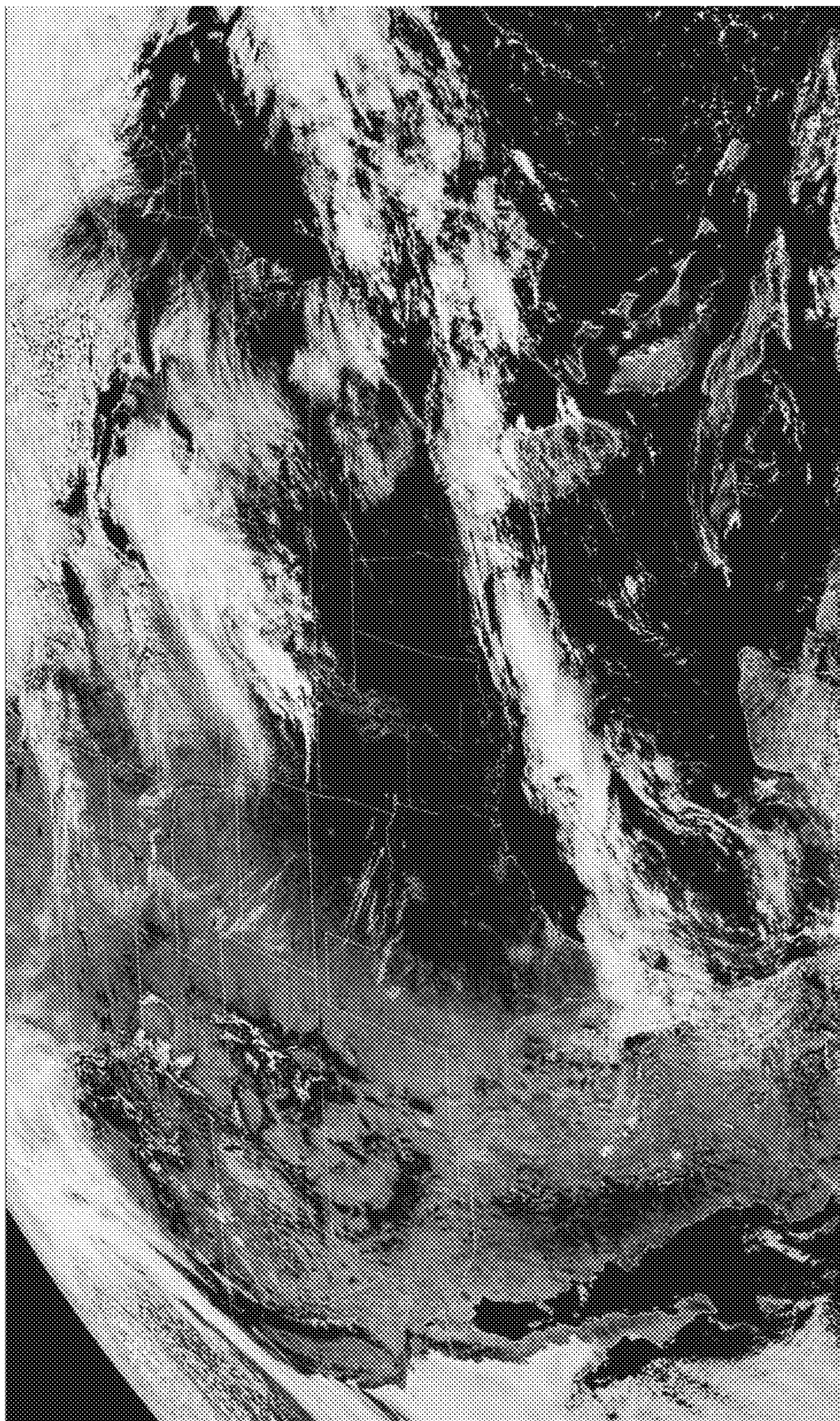
FIGURE 4 Satellite Imagery
