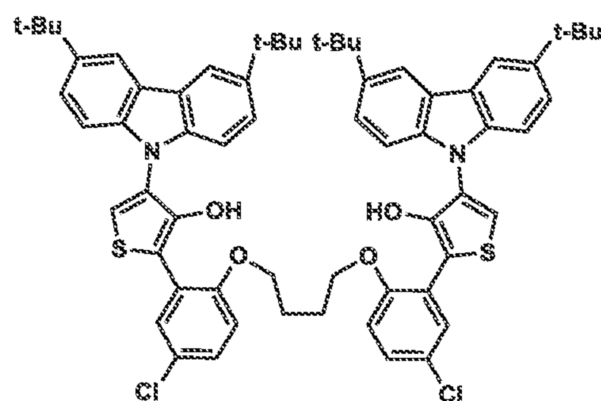
Ligand 21
