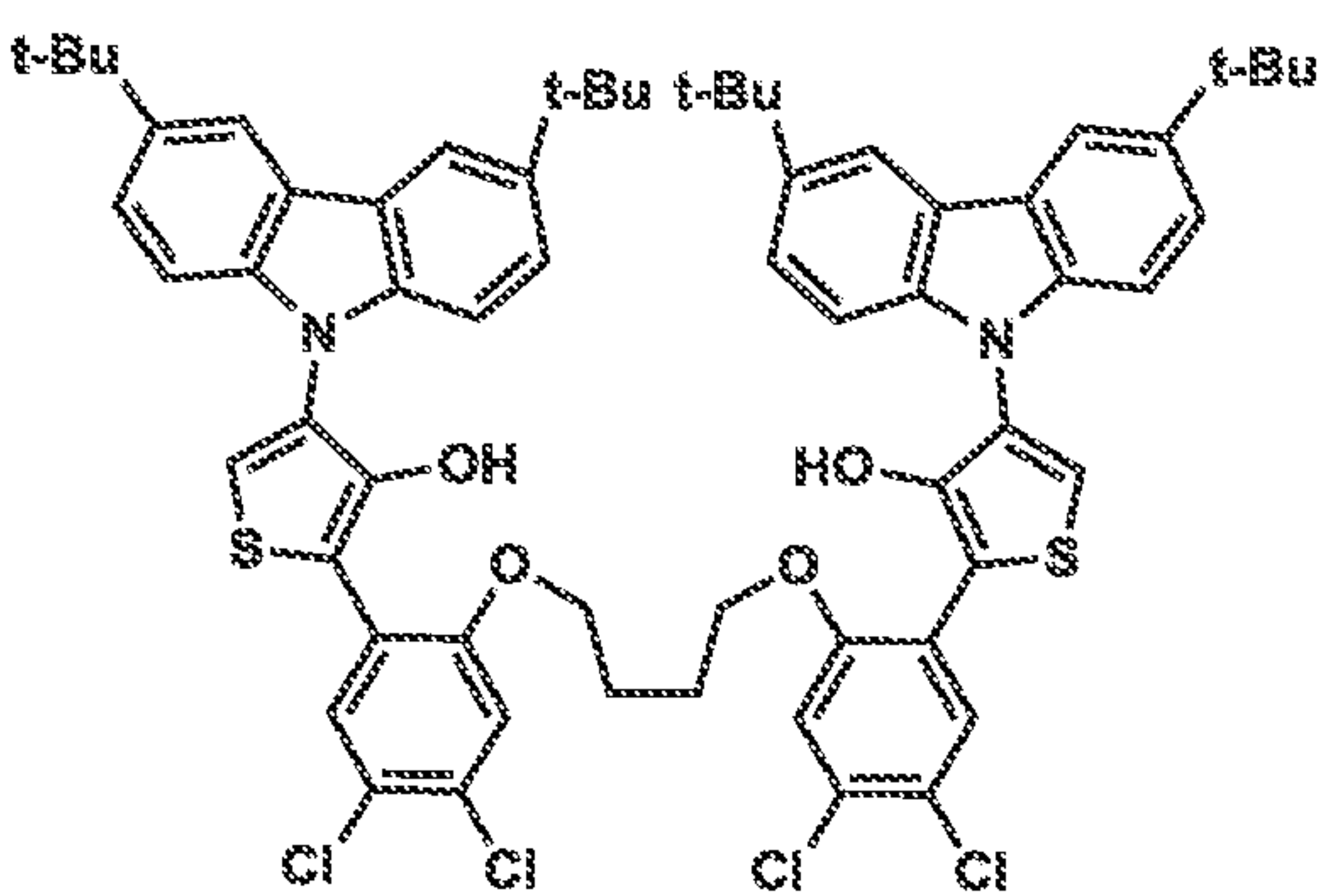
Ligand 24
