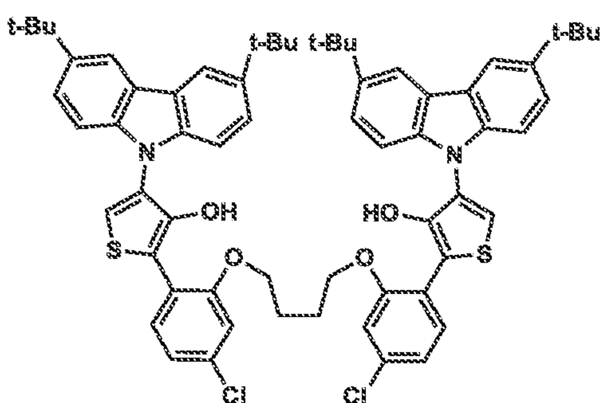
Ligand 22
