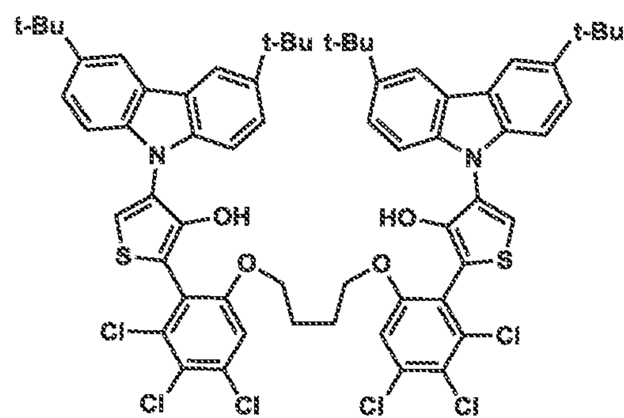
Ligand 25
